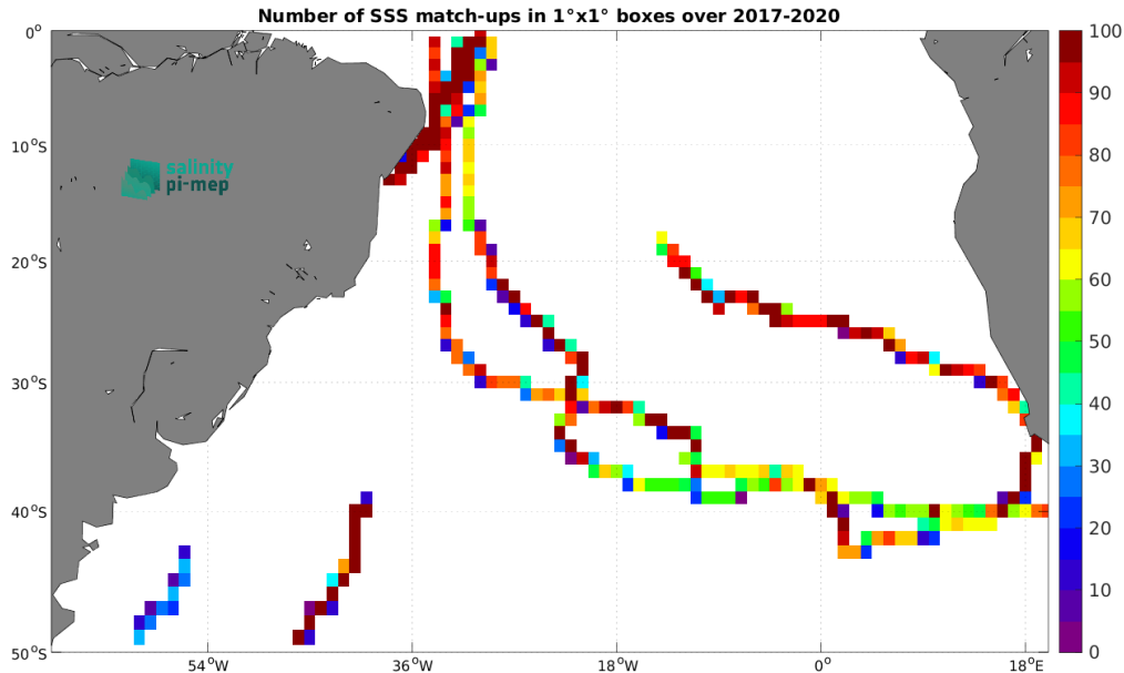
Figure 5: Number of SSS match-ups between TSG (GOSUD-Sailing-ship) SSS and the SMAP SSS L3 v6 - Monthly (RSS) SSS product for the South Atlantic Ocean Pi-MEP region over 1^\circ \times 1^\circ boxes and for the full satellite product period.
