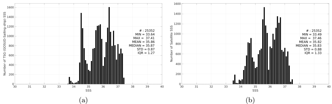
Figure 3: Histograms of SSS from TSG (GOSUD-Sailing-ship) (a) and SMAP SSS L3 v6 - Monthly (RSS) (b) considering all match-up pairs per bins of 0.1 over the South Atlantic Ocean Pi-MEP region and for the full satellite product period.
