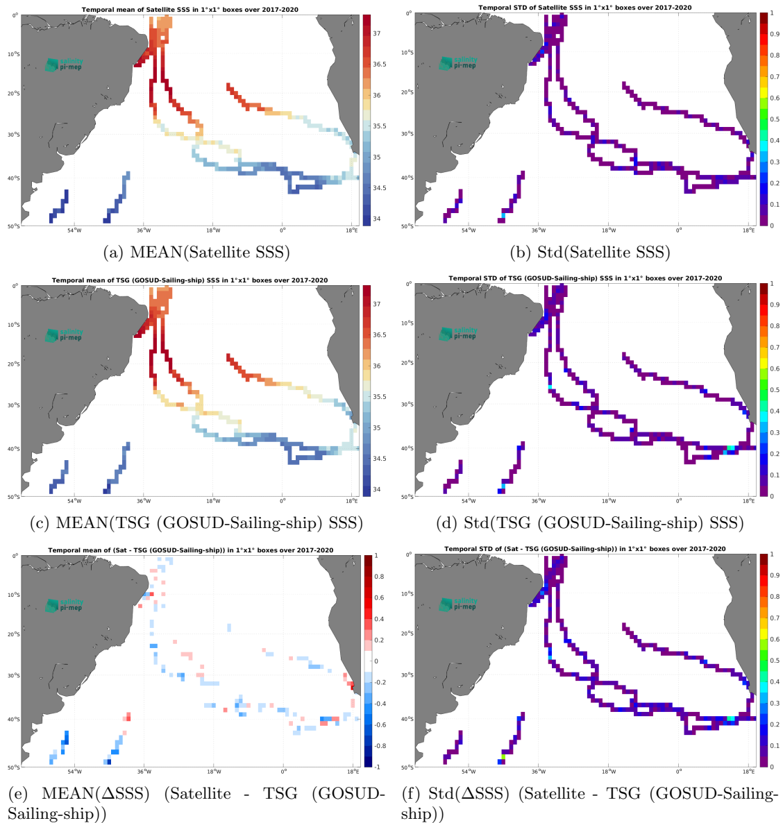
Figure 7: Temporal mean (left) and Std (right) of SSS from SMAP SSS L3 v6 - Monthly (RSS) (top), TSG (GOSUD-Sailing-ship) (middle), and of \Delta SSS (Satellite - TSG (GOSUD-Sailing-ship)). Only match-up pairs are used to generate these maps.
