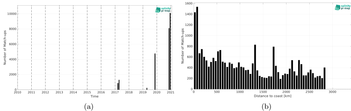
Figure 2: Number of match-ups between TSG (GOSUD-Sailing-ship) and SMAP SSS L3 v6 - Monthly (RSS) SSS as a function of time (a) and as function of the distance to coast (b) over the South Atlantic Ocean Pi-MEP region and for the full satellite product period.
