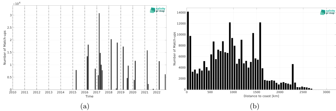
Figure 2: Number of match-ups between TSG (GOSUD-Research-vessel) and SMAP SSS L3 v6 - Monthly (RSS) SSS as a function of time (a) and as function of the distance to coast (b) over the South Atlantic Ocean Pi-MEP region and for the full satellite product period.
