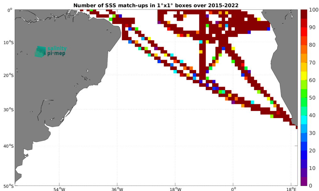
Figure 5: Number of SSS match-ups between TSG (GOSUD-Research-vessel) SSS and the SMAP SSS L3 v6 - Monthly (RSS) SSS product for the South Atlantic Ocean Pi-MEP region over 1^\circ \times 1^\circ boxes and for the full satellite product period.
