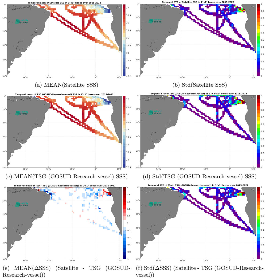
Figure 7: Temporal mean (left) and Std (right) of SSS from SMAP SSS L3 v6 - Monthly (RSS) (top), TSG (GOSUD-Research-vessel) (middle), and of \Delta SSS (Satellite - TSG (GOSUD-Research-vessel)). Only match-up pairs are used to generate these maps.
