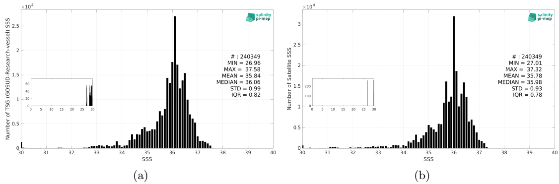
Figure 3: Histograms of SSS from TSG (GOSUD-Research-vessel) (a) and SMAP SSS L3 v6 - Monthly (RSS) (b) considering all match-up pairs per bins of 0.1 over the South Atlantic Ocean Pi-MEP region and for the full satellite product period.
