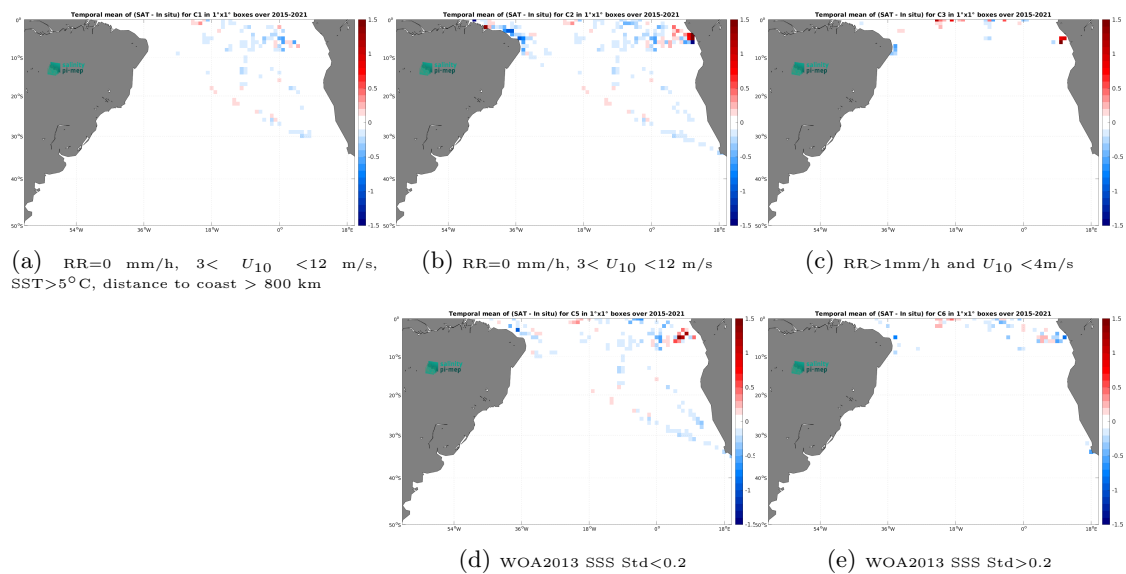
Figure 14: Temporal mean gridded over spatial boxes of size 1^\circ \times 1^\circ of \Delta\text{SSS} (SMAP SSS L3 v6 - Monthly (RSS) - TSG (GOSUD-Research-vessel)) for 5 different subdatasets corresponding to:RR=0 mm/h, 3 < U_{10} < 12 m/s, SST >5^\circ\text{C} , distance to coast > 800 km (a), RR=0 mm/h, 3 < U_{10} < 12 m/s (b), RR >1 mm/h and U_{10} < 4 m/s (c), WOA2013 SSS Std <0.2 (d), WOA2013 SSS Std >0.2 (e).
