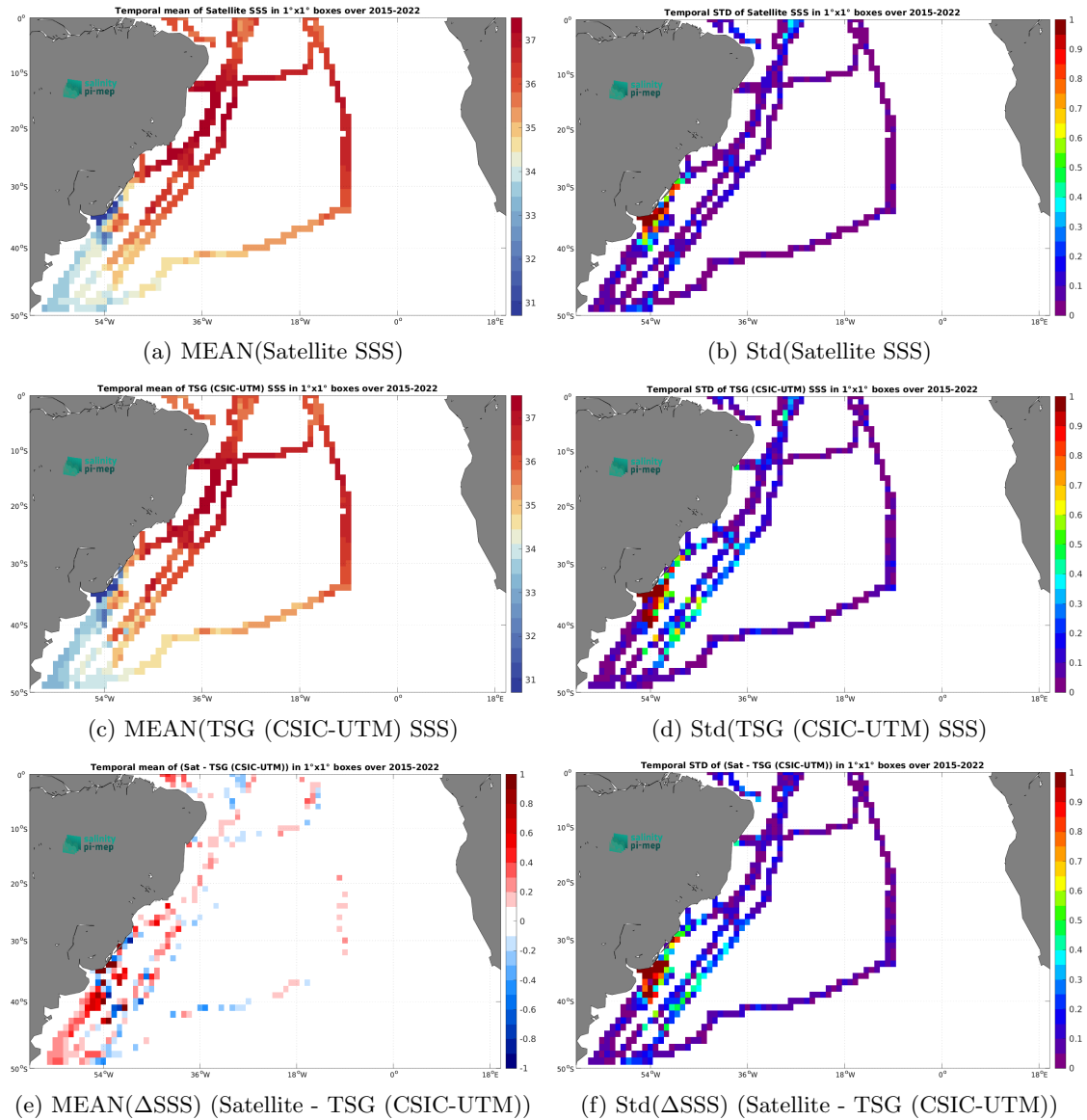
Figure 7: Temporal mean (left) and Std (right) of SSS from SMAP SSS L3 v6 - Monthly (RSS) (top), TSG (CSIC-UTM) (middle), and of \Delta SSS (Satellite - TSG (CSIC-UTM)). Only match-up pairs are used to generate these maps.
