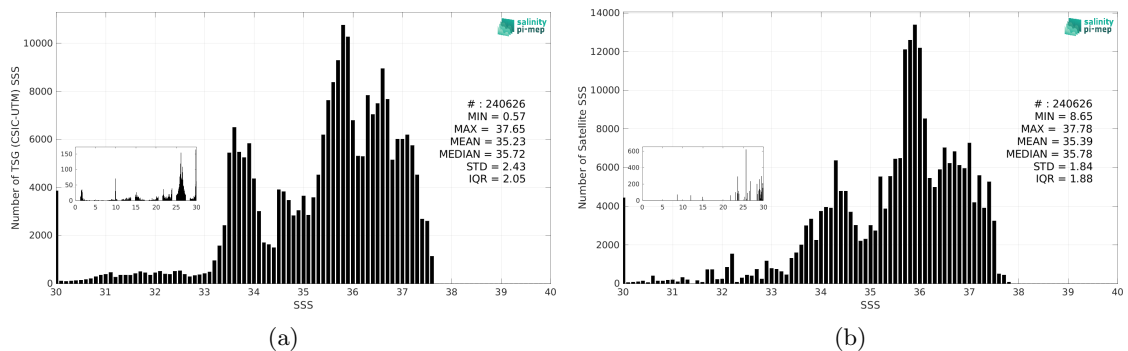
Figure 3: Histograms of SSS from TSG (CSIC-UTM) (a) and SMAP SSS L3 v6 - Monthly (RSS) (b) considering all match-up pairs per bins of 0.1 over the South Atlantic Ocean Pi-MEP region and for the full satellite product period.
