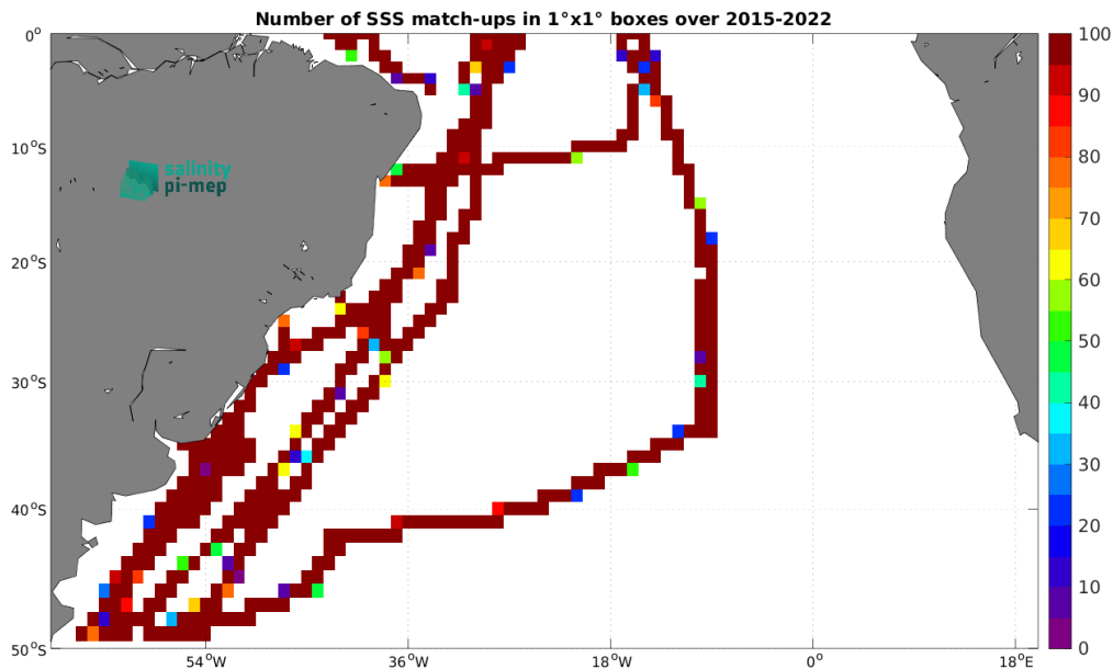
Figure 5: Number of SSS match-ups between TSG (CSIC-UTM) SSS and the SMAP SSS L3 v6 - Monthly (RSS) SSS product for the South Atlantic Ocean Pi-MEP region over 1^\circ \times 1^\circ boxes and for the full satellite product period.
