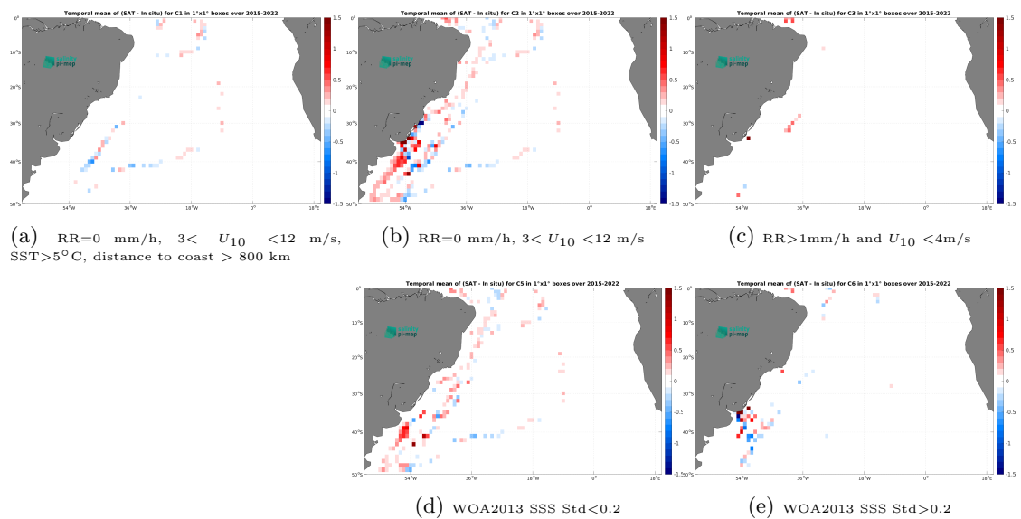
Figure 14: Temporal mean gridded over spatial boxes of size 1^\circ \times 1^\circ of \Delta SSS (SMAP SSS L3 v6 - Monthly (RSS) - TSG (CSIC-UTM)) for 5 different subdatasets corresponding to:RR=0 mm/h, 3 < U_{10} < 12 m/s, SST>5°C, distance to coast > 800 km (a), RR=0 mm/h, 3 < U_{10} < 12 m/s (b), RR>1mm/h and U_{10} < 4 m/s (c), WOA2013 SSS Std<0.2 (d), WOA2013 SSS Std>0.2 (e).
