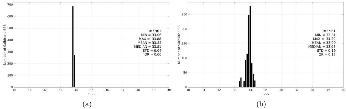
Figure 3: Histograms of SSS from Saildrone (a) and SMAP SSS L3 v6 - Monthly (RSS) (b) considering all match-up pairs per bins of 0.1 over the South Atlantic Ocean Pi-MEP region and for the full satellite product period.
