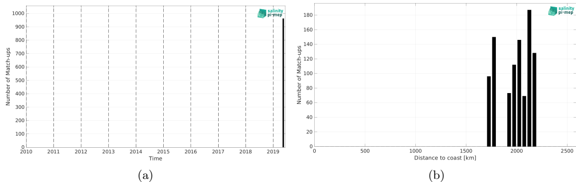
Figure 2: Number of match-ups between Sairdrone and SMAP SSS L3 v6 - Monthly (RSS) SSS as a function of time (a) and as function of the distance to coast (b) over the South Atlantic Ocean Pi-MEP region and for the full satellite product period.
