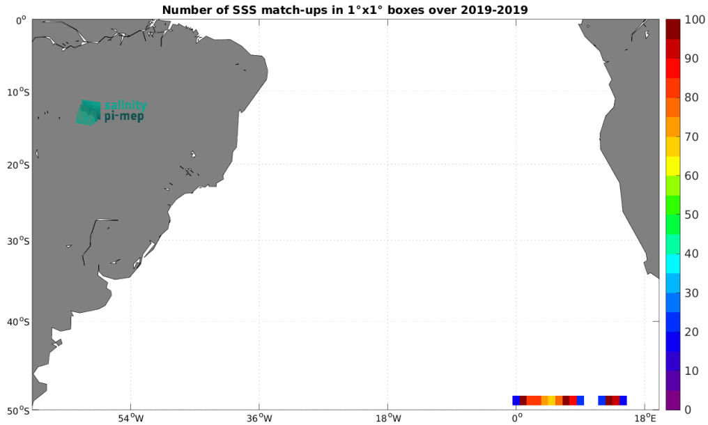
Figure 5: Number of SSS match-ups between Saildrone SSS and the SMAP SSS L3 v6 - Monthly (RSS) SSS product for the South Atlantic Ocean Pi-MEP region over 1^\circ \times 1^\circ boxes and for the full satellite product period.
