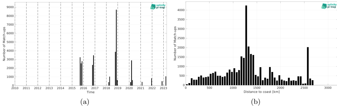
Figure 2: Number of match-ups between TSG (SAMOS) and SMAP SSS L3 v5.3 - 8-Day running (RSS) SSS as a function of time (a) and as function of the distance to coast (b) over the South Atlantic Ocean Pi-MEP region and for the full satellite product period.
