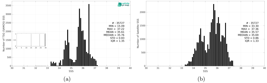
Figure 3: Histograms of SSS from TSG (SAMOS) (a) and SMAP SSS L3 v5.3 - 8-Day running (RSS) (b) considering all match-up pairs per bins of 0.1 over the South Atlantic Ocean Pi-MEP region and for the full satellite product period.
