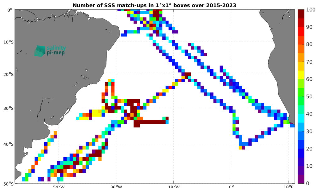
Figure 5: Number of SSS match-ups between TSG (SAMOS) SSS and the SMAP SSS L3 v5.3 - 8-Day running (RSS) SSS product for the South Atlantic Ocean Pi-MEP region over 1^\circ \times 1^\circ boxes and for the full satellite product period.
