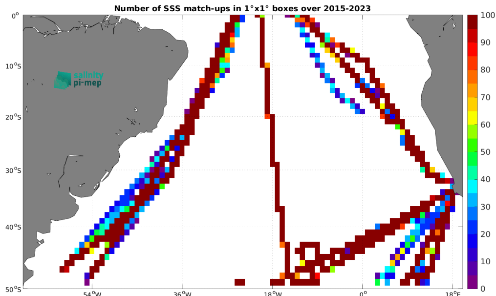
Figure 5: Number of SSS match-ups between TSG (Polarstern) SSS and the SMAP SSS L3 v5.3 - 8-Day running (RSS) SSS product for the South Atlantic Ocean Pi-MEP region over 1^\circ \times 1^\circ boxes and for the full satellite product period.
