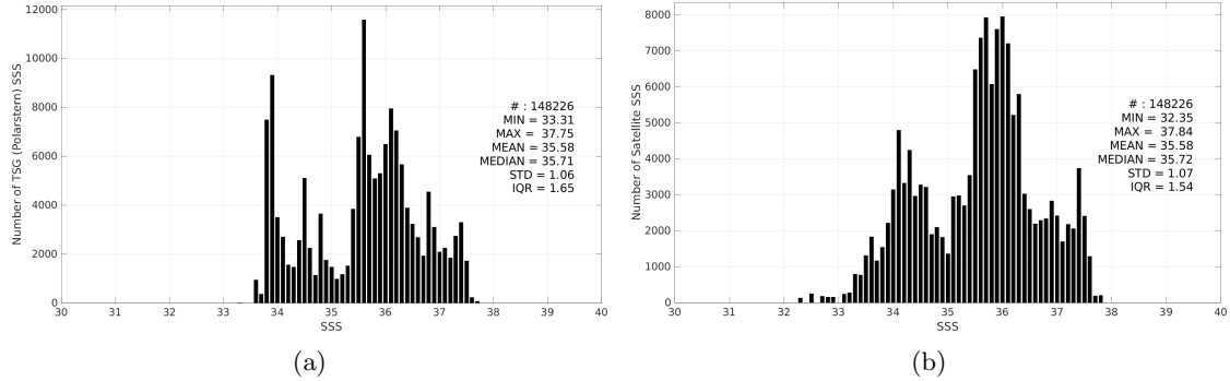
Figure 3: Histograms of SSS from TSG (Polarstern) (a) and SMAP SSS L3 v5.3 - 8-Day running (RSS) (b) considering all match-up pairs per bins of 0.1 over the South Atlantic Ocean Pi-MEP region and for the full satellite product period.
