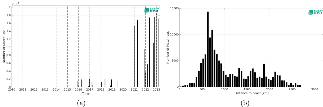
Figure 2: Number of match-ups between TSG (Polarstern) and SMAP SSS L3 v5.3 - 8-Day running (RSS) SSS as a function of time (a) and as function of the distance to coast (b) over the South Atlantic Ocean Pi-MEP region and for the full satellite product period.
