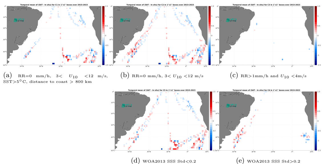
Figure 14: Temporal mean gridded over spatial boxes of size 1^\circ \times 1^\circ of \Delta\text{SSS} (SMAP SSS L3 v5.3 - 8-Day running (RSS) - TSG (Polarstern)) for 5 different subdatasets corresponding to:RR=0 mm/h, 3 < U_{10} < 12 m/s, SST >5^\circ\text{C} , distance to coast > 800 km (a), RR=0 mm/h, 3 < U_{10} < 12 m/s (b), RR >1 mm/h and U_{10} < 4 m/s (c), WOA2013 SSS Std <0.2 (d), WOA2013 SSS Std >0.2 (e).
