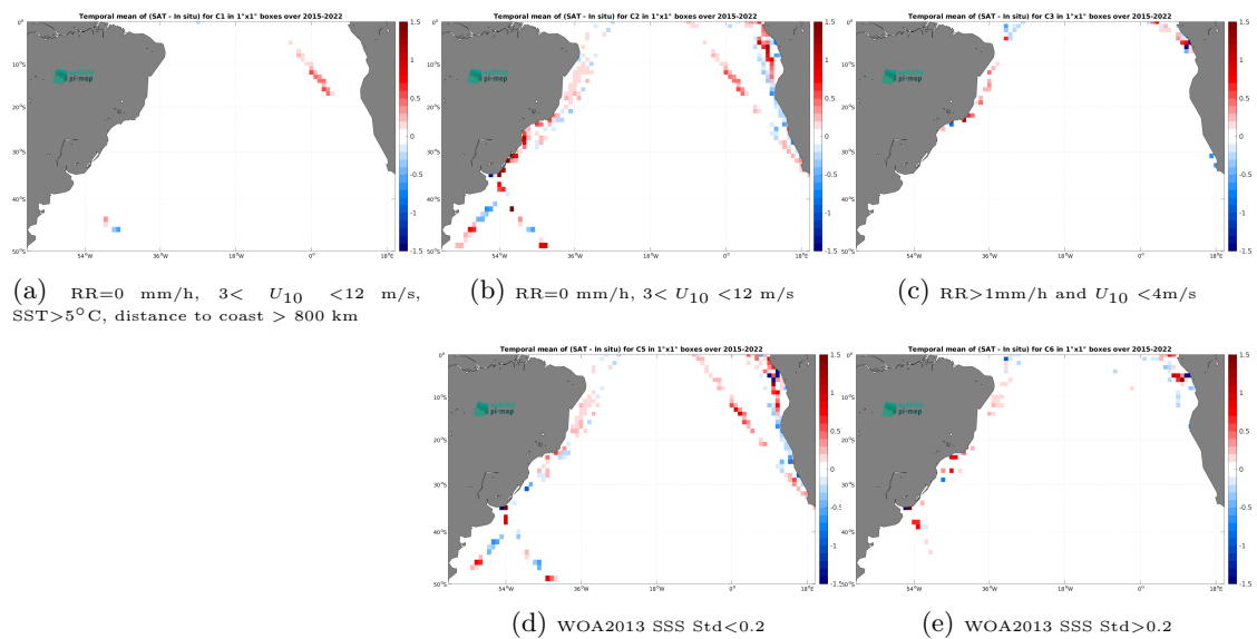
Figure 14: Temporal mean gridded over spatial boxes of size 1^\circ \times 1^\circ of \Delta SSS (SMAP SSS L3 v5.3 - 8-Day running (RSS) - TSG (LEGOS-DM)) for 5 different subdatasets corresponding to:RR=0 mm/h, 3 < U_{10} < 12 m/s, SST >5^\circ\text{C} , distance to coast > 800 km (a), RR=0 mm/h, 3 < U_{10} < 12 m/s (b), RR >1 mm/h and U_{10} < 4 m/s (c), WOA2013 SSS Std <0.2 (d), WOA2013 SSS Std >0.2 (e).
