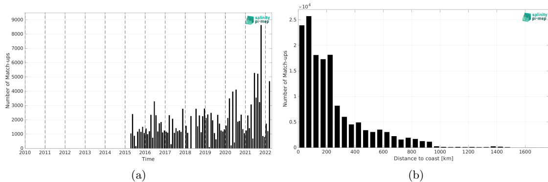
Figure 2: Number of match-ups between TSG (LEGOS-DM) and SMAP SSS L3 v5.3 - 8-Day running (RSS) SSS as a function of time (a) and as function of the distance to coast (b) over the South Atlantic Ocean Pi-MEP region and for the full satellite product period.
