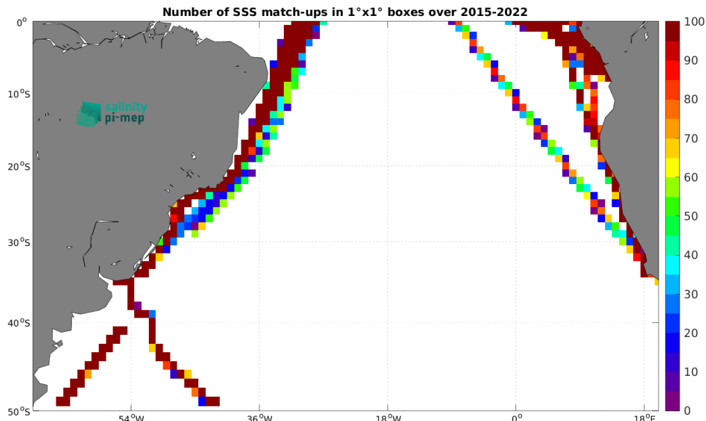
Figure 5: Number of SSS match-ups between TSG (LEGOS-DM) SSS and the SMAP SSS L3 v5.3 - 8-Day running (RSS) SSS product for the South Atlantic Ocean Pi-MEP region over 1^\circ \times 1^\circ boxes and for the full satellite product period.
