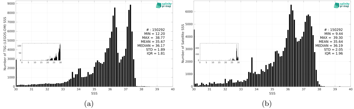
Figure 3: Histograms of SSS from TSG (LEGOS-DM) (a) and SMAP SSS L3 v5.3 - 8-Day running (RSS) (b) considering all match-up pairs per bins of 0.1 over the South Atlantic Ocean Pi-MEP region and for the full satellite product period.
