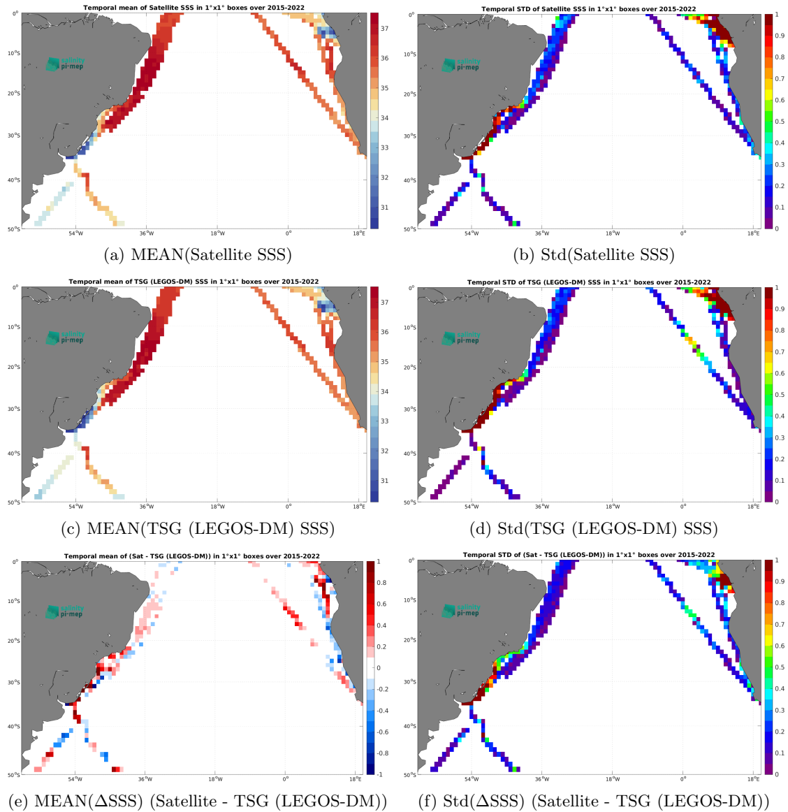
Figure 7: Temporal mean (left) and Std (right) of SSS from SMAP SSS L3 v5.3 - 8-Day running (RSS) (top), TSG (LEGOS-DM) (middle), and of \Delta SSS (Satellite - TSG (LEGOS-DM)). Only match-up pairs are used to generate these maps.
