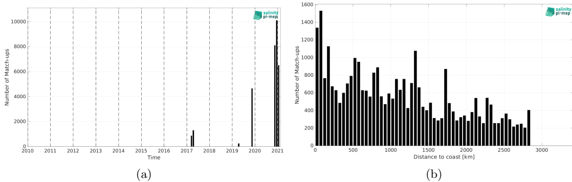
Figure 2: Number of match-ups between TSG (GOSUD-Sailing-ship) and SMAP SSS L3 v5.3 - 8-Day running (RSS) SSS as a function of time (a) and as function of the distance to coast (b) over the South Atlantic Ocean Pi-MEP region and for the full satellite product period.
