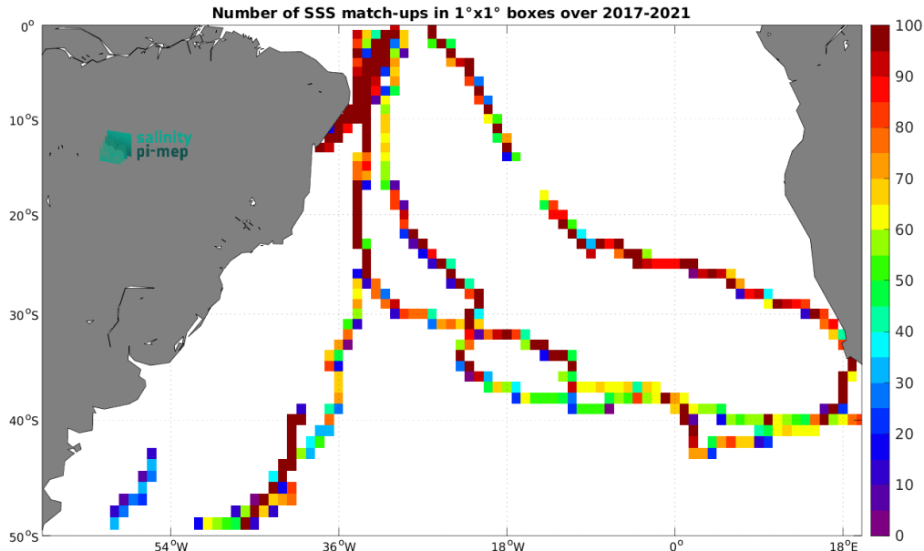
Figure 5: Number of SSS match-ups between TSG (GOSUD-Sailing-ship) SSS and the SMAP SSS L3 v5.3 - 8-Day running (RSS) SSS product for the South Atlantic Ocean Pi-MEP region over 1^\circ \times 1^\circ boxes and for the full satellite product period.
