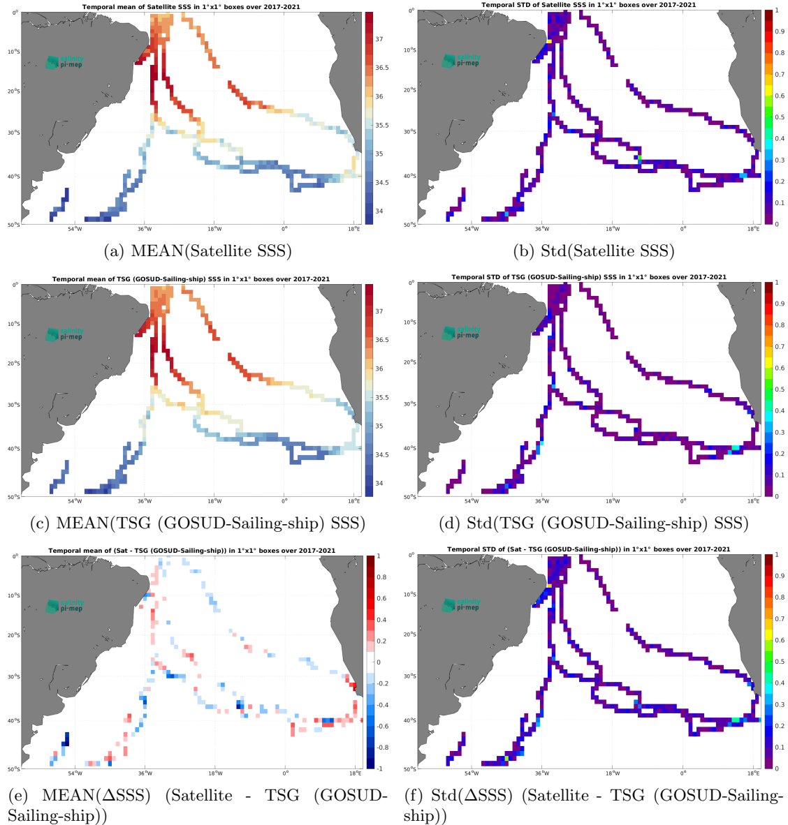
Figure 7: Temporal mean (left) and Std (right) of SSS from SMAP SSS L3 v5.3 - 8-Day running (RSS) (top), TSG (GOSUD-Sailing-ship) (middle), and of \Delta SSS (Satellite - TSG (GOSUD-Sailing-ship)). Only match-up pairs are used to generate these maps.
