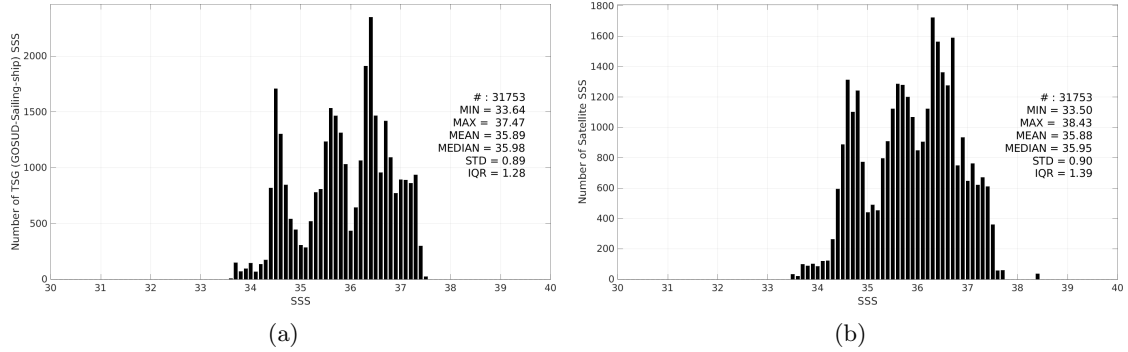
Figure 3: Histograms of SSS from TSG (GOSUD-Sailing-ship) (a) and SMAP SSS L3 v5.3 - 8-Day running (RSS) (b) considering all match-up pairs per bins of 0.1 over the South Atlantic Ocean Pi-MEP region and for the full satellite product period.
