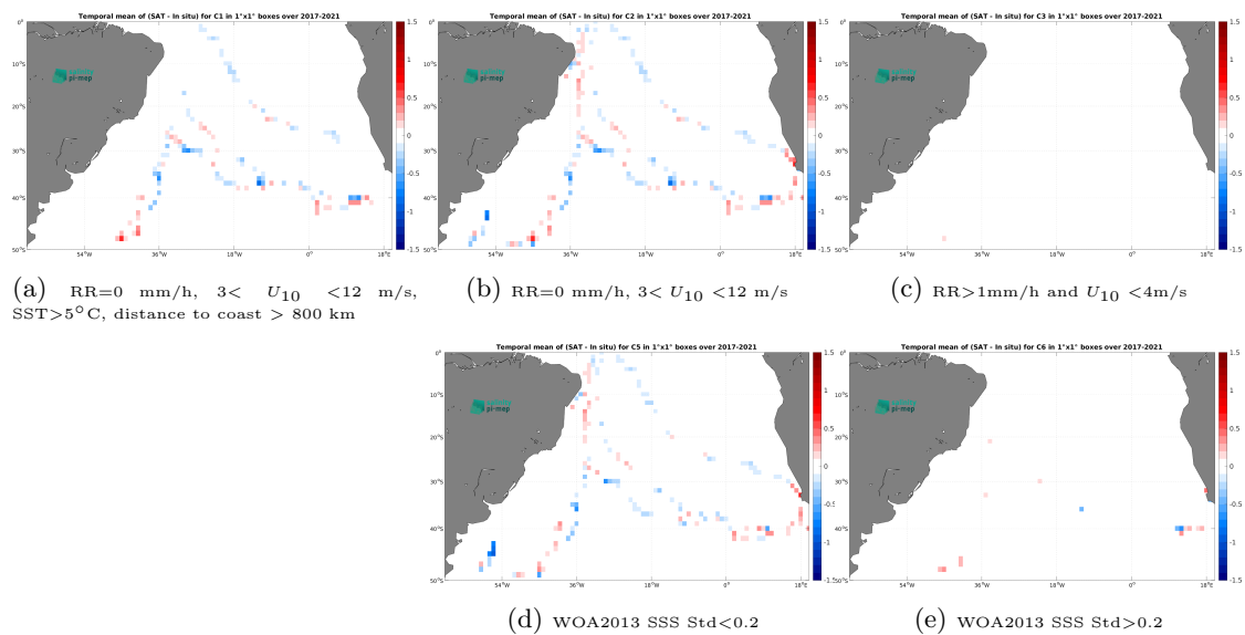
Figure 14: Temporal mean gridded over spatial boxes of size 1^\circ \times 1^\circ of \Delta\text{SSS} (SMAP SSS L3 v5.3 - 8-Day running (RSS) - TSG (GOSUD-Sailing-ship)) for 5 different subdatasets corresponding to:RR=0 mm/h, 3 < U_{10} < 12 m/s, SST >5^\circ\text{C} , distance to coast > 800 km (a), RR=0 mm/h, 3 < U_{10} < 12 m/s (b), RR >1 mm/h and U_{10} < 4 m/s (c), WOA2013 SSS Std <0.2 (d), WOA2013 SSS Std >0.2 (e).
