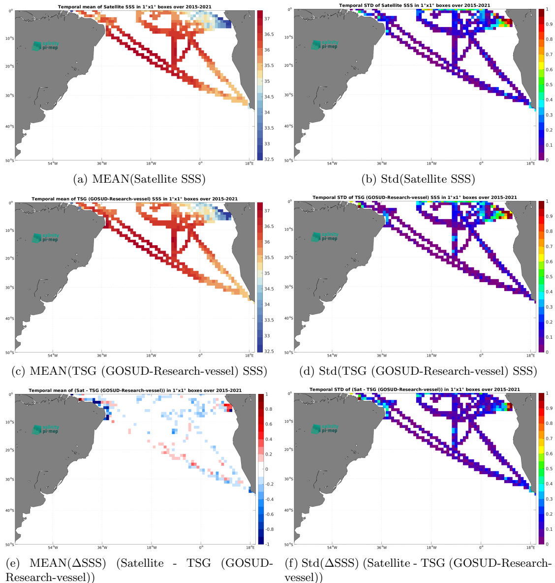
Figure 7: Temporal mean (left) and Std (right) of SSS from SMAP SSS L3 v5.3 - 8-Day running (RSS) (top), TSG (GOSUD-Research-vessel) (middle), and of \Delta SSS (Satellite - TSG (GOSUD-Research-vessel)). Only match-up pairs are used to generate these maps.
