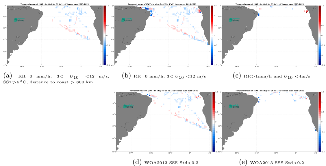
Figure 14: Temporal mean gridded over spatial boxes of size 1^\circ \times 1^\circ of \Delta SSS (SMAP SSS L3 v5.3 - 8-Day running (RSS) - TSG (GOSUD-Research-vessel)) for 5 different subdatasets corresponding to:RR=0 mm/h, 3 < U_{10} < 12 m/s, SST >5^\circ\text{C} , distance to coast > 800 km (a), RR=0 mm/h, 3 < U_{10} < 12 m/s (b), RR >1 mm/h and U_{10} < 4 m/s (c), WOA2013 SSS Std <0.2 (d), WOA2013 SSS Std >0.2 (e).
