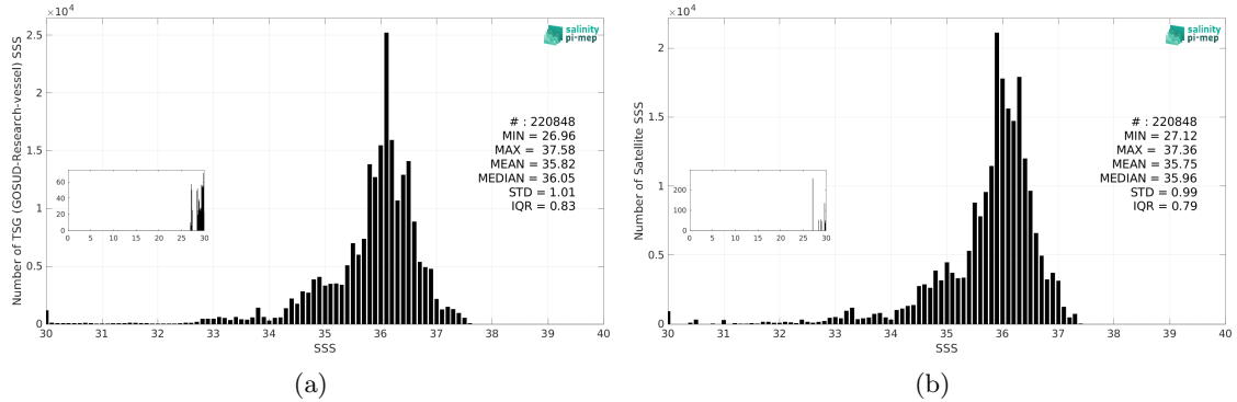
Figure 3: Histograms of SSS from TSG (GOSUD-Research-vessel) (a) and SMAP SSS L3 v5.3 - 8-Day running (RSS) (b) considering all match-up pairs per bins of 0.1 over the South Atlantic Ocean Pi-MEP region and for the full satellite product period.
