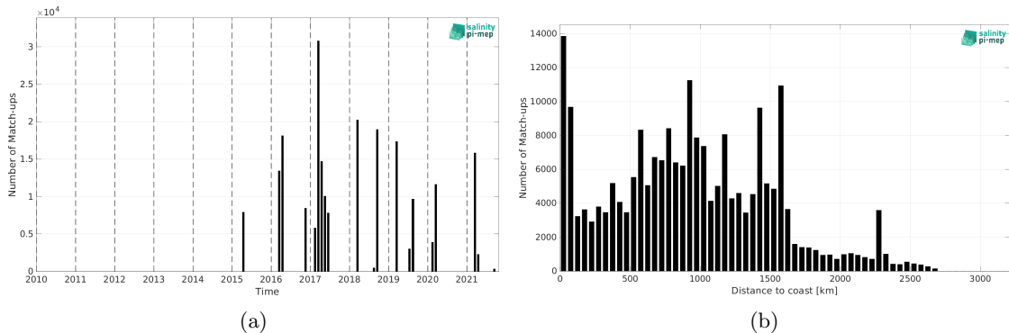
Figure 2: Number of match-ups between TSG (GOSUD-Research-vessel) and SMAP SSS L3 v5.3 - 8-Day running (RSS) SSS as a function of time (a) and as function of the distance to coast (b) over the South Atlantic Ocean Pi-MEP region and for the full satellite product period.
