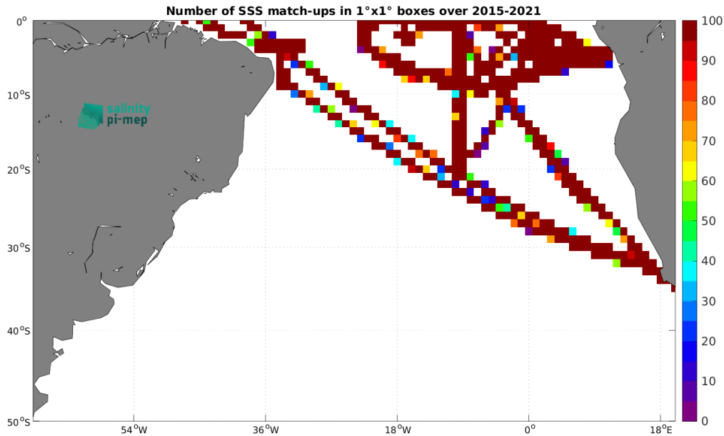
Figure 5: Number of SSS match-ups between TSG (GOSUD-Research-vessel) SSS and the SMAP SSS L3 v5.3 - 8-Day running (RSS) SSS product for the South Atlantic Ocean Pi-MEP region over 1^\circ \times 1^\circ boxes and for the full satellite product period.
