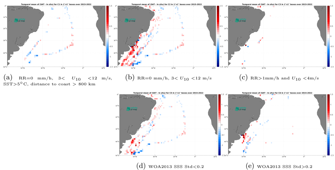
Figure 14: Temporal mean gridded over spatial boxes of size 1^\circ \times 1^\circ of \Delta\text{SSS} (SMAP SSS L3 v5.3 - 8-Day running (RSS) - TSG (CSIC-UTM)) for 5 different subdatasets corresponding to:RR=0 mm/h, 3 < U_{10} < 12 m/s, SST >5^\circ\text{C} , distance to coast > 800 km (a), RR=0 mm/h, 3 < U_{10} < 12 m/s (b), RR >1 mm/h and U_{10} < 4 m/s (c), WOA2013 SSS Std <0.2 (d), WOA2013 SSS Std >0.2 (e).
