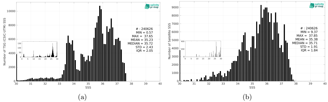
Figure 3: Histograms of SSS from TSG (CSIC-UTM) (a) and SMAP SSS L3 v5.3 - 8-Day running (RSS) (b) considering all match-up pairs per bins of 0.1 over the South Atlantic Ocean Pi-MEP region and for the full satellite product period.
