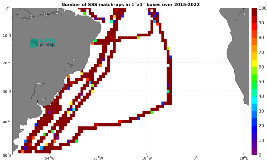
Figure 5: Number of SSS match-ups between TSG (CSIC-UTM) SSS and the SMAP SSS L3 v5.3 - 8-Day running (RSS) SSS product for the South Atlantic Ocean Pi-MEP region over 1^\circ \times 1^\circ boxes and for the full satellite product period.
