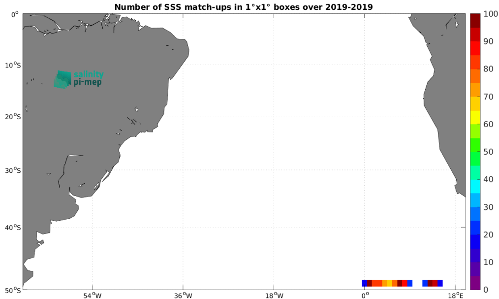
Figure 5: Number of SSS match-ups between Sairdrone SSS and the SMAP SSS L3 v5.3 - 8-Day running (RSS) SSS product for the South Atlantic Ocean Pi-MEP region over 1^\circ \times 1^\circ boxes and for the full satellite product period.
