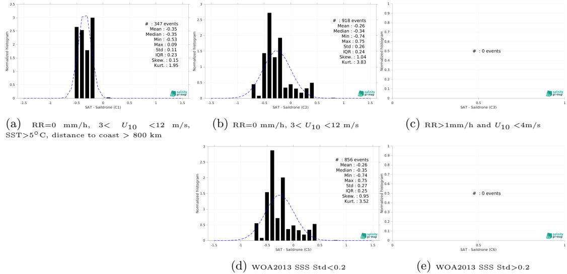
Figure 15: Normalized histogram of \Delta SSS (SMAP SSS L3 v5.3 - 8-Day running (RSS) - Saildrone) for 5 different subdatasets corresponding to: RR=0 mm/h, 3 < U_{10} < 12 m/s, SST > 5°C, distance to coast > 800 km (a), RR=0 mm/h, 3 < U_{10} < 12 m/s (b), RR > 1mm/h and U_{10} < 4 m/s (c), WOA2013 SSS Std < 0.2 (d), WOA2013 SSS Std > 0.2 (e).
