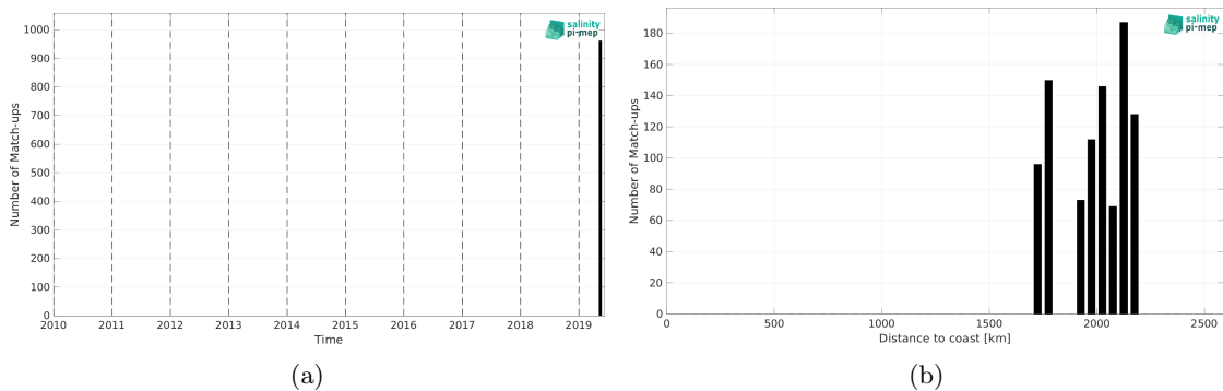
Figure 2: Number of match-ups between Saildrone and SMAP SSS L3 v5.3 - 8-Day running (RSS) SSS as a function of time (a) and as a function of the distance to coast (b) over the South Atlantic Ocean Pi-MEP region and for the full satellite product period.
