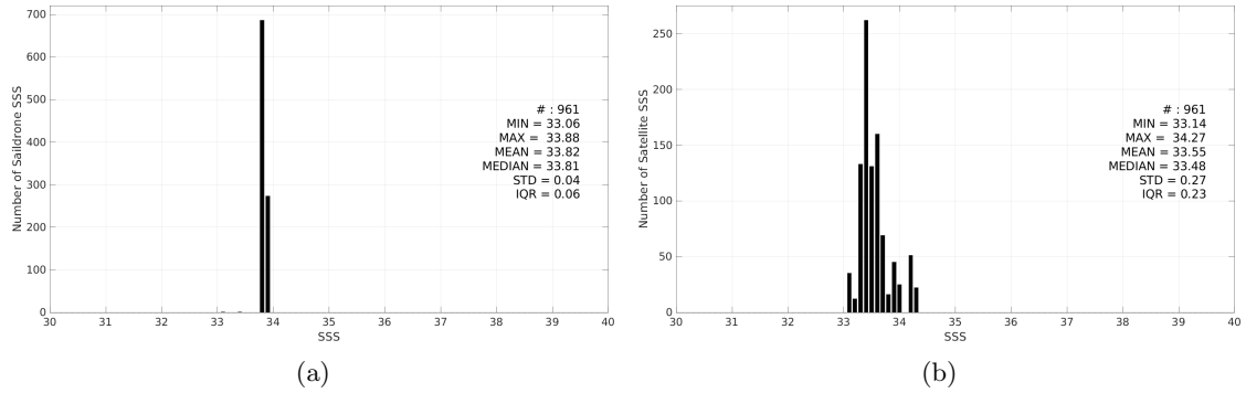
Figure 3: Histograms of SSS from Saildrone (a) and SMAP SSS L3 v5.3 - 8-Day running (RSS) (b) considering all match-up pairs per bins of 0.1 over the South Atlantic Ocean Pi-MEP region and for the full satellite product period.
