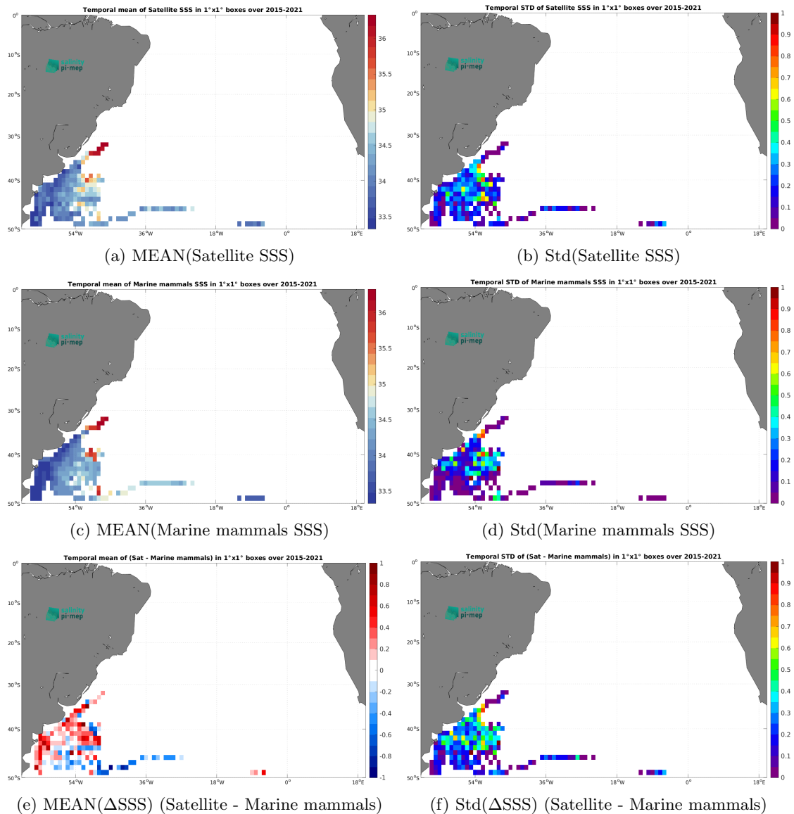
Figure 7: Temporal mean (left) and Std (right) of SSS from SMAP SSS L3 v5.3 - 8-Day running (RSS) (top), Marine mammals (middle), and of \Delta SSS (Satellite - Marine mammals). Only match-up pairs are used to generate these maps.
