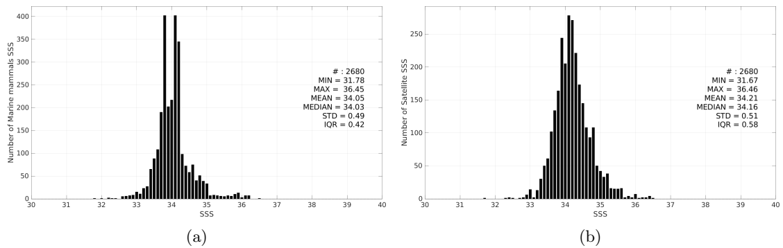
Figure 3: Histograms of SSS from Marine mammals (a) and SMAP SSS L3 v5.3 - 8-Day running (RSS) (b) considering all match-up pairs per bins of 0.1 over the South Atlantic Ocean Pi-MEP region and for the full satellite product period.
