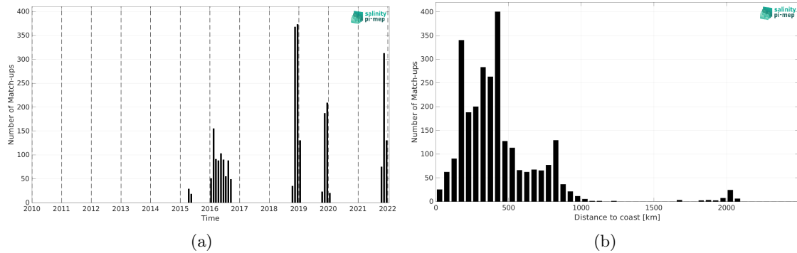
Figure 2: Number of match-ups between Marine mammals and SMAP SSS L3 v5.3 - 8-Day running (RSS) SSS as a function of time (a) and as function of the distance to coast (b) over the South Atlantic Ocean Pi-MEP region and for the full satellite product period.
