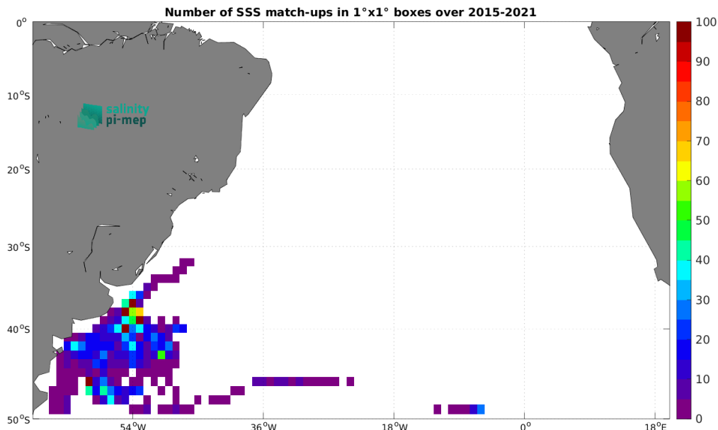
Figure 5: Number of SSS match-ups between Marine mammals SSS and the SMAP SSS L3 v5.3 - 8-Day running (RSS) SSS product for the South Atlantic Ocean Pi-MEP region over 1^\circ \times 1^\circ boxes and for the full satellite product period.
