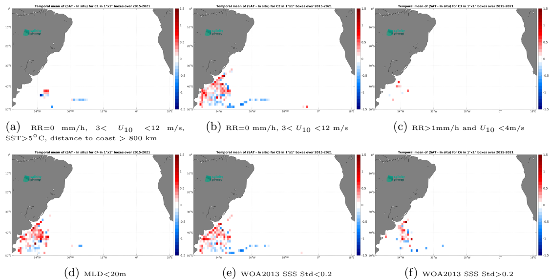
Figure 14: Temporal mean gridded over spatial boxes of size 1^\circ \times 1^\circ of \Delta SSS (SMAP SSS L3 v5.3 - 8-Day running (RSS) - Marine mammals) for 6 different subdatasets corresponding to:RR=0 mm/h, 3 < U_{10} < 12 m/s, SST >5^\circ C, distance to coast > 800 km (a), RR=0 mm/h, 3 < U_{10} < 12 m/s (b), RR >1 mm/h and U_{10} < 4 m/s (c),MLD <20 m (d),WOA2013 SSS Std <0.2 (e),WOA2013 SSS Std >0.2 (f).
