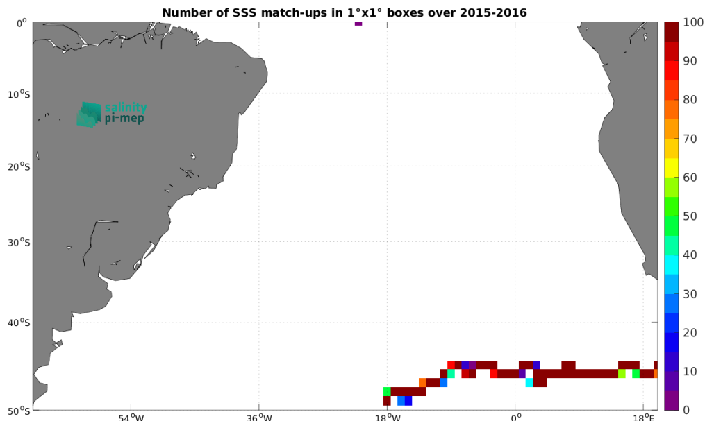
Figure 4: Number of SSS match-ups between Surface drifters SSS and the SMAP SSS L3 v5.3 - 8-Day running (RSS) SSS product for the South Atlantic Ocean Pi-MEP region over 1^\circ \times 1^\circ boxes and for the full satellite product period.
