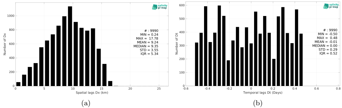
Figure 5: Histograms of the spatial (a) and temporal (b) lags between the location/time of the Surface drifters measurement and the date of the corresponding SMAP SSS L3 v5.3 - 8-Day running (RSS) SSS pixel.
