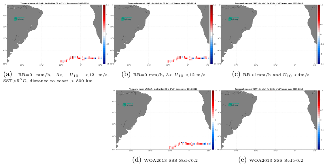
Figure 13: Temporal mean gridded over spatial boxes of size 1^\circ \times 1^\circ of \Delta\text{SSS} (SMAP SSS L3 v5.3 - 8-Day running (RSS) - Surface drifters) for 5 different subdatasets corresponding to: \text{RR}=0 mm/h, 3 < U_{10} < 12 m/s, \text{SST} > 5^\circ\text{C} , distance to coast > 800 km (a), \text{RR}=0 mm/h, 3 < U_{10} < 12 m/s (b), \text{RR} > 1\text{mm/h} and U_{10} < 4\text{m/s} (c), WOA2013 SSS Std < 0.2 (d), WOA2013 SSS Std > 0.2 (e).
