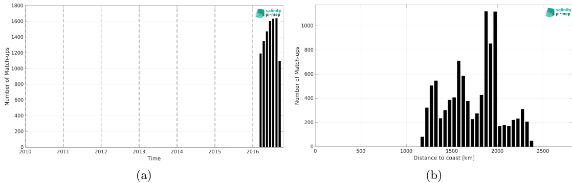
Figure 2: Number of match-ups between Surface drifters and SMAP SSS L3 v5.3 - 8-Day running (RSS) SSS as a function of time (a) and as function of the distance to coast (b) over the South Atlantic Ocean Pi-MEP region and for the full satellite product period.
