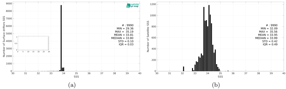
Figure 3: Histograms of SSS from Surface drifters (a) and SMAP SSS L3 v5.3 - 8-Day running (RSS) (b) considering all match-up pairs per bins of 0.1 over the South Atlantic Ocean Pi-MEP region and for the full satellite product period.
