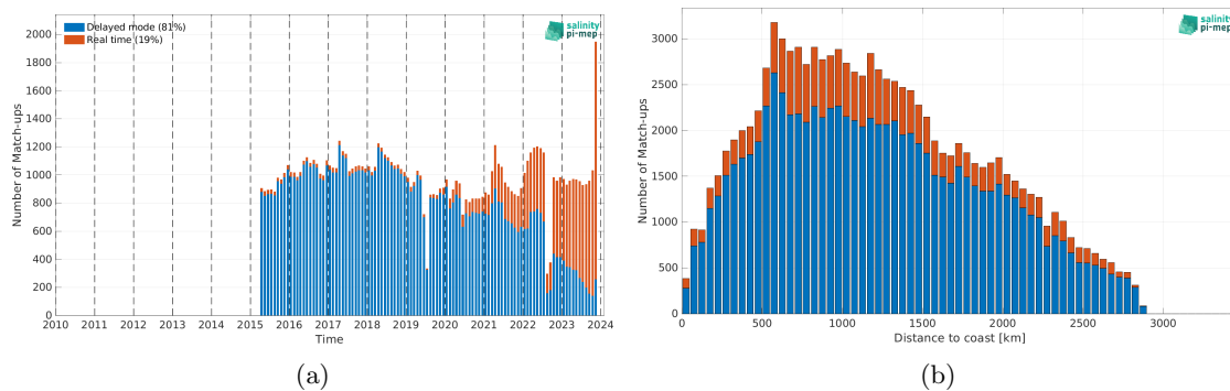
Figure 2: Number of match-ups between Argo and SMAP SSS L3 v5.3 - 8-Day running (RSS) SSS as a function of time (a) and as function of the distance to coast (b) over the South Atlantic Ocean Pi-MEP region and for the full satellite product period.
