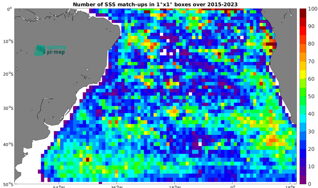
Figure 5: Number of SSS match-ups between Argo SSS and the SMAP SSS L3 v5.3 - 8-Day running (RSS) SSS product for the South Atlantic Ocean Pi-MEP region over 1^\circ \times 1^\circ boxes and for the full satellite product period.
