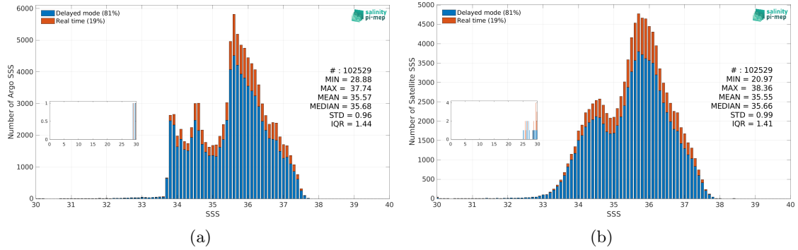
Figure 3: Histograms of SSS from Argo (a) and SMAP SSS L3 v5.3 - 8-Day running (RSS) (b) considering all match-up pairs per bins of 0.1 over the South Atlantic Ocean Pi-MEP region and for the full satellite product period.
