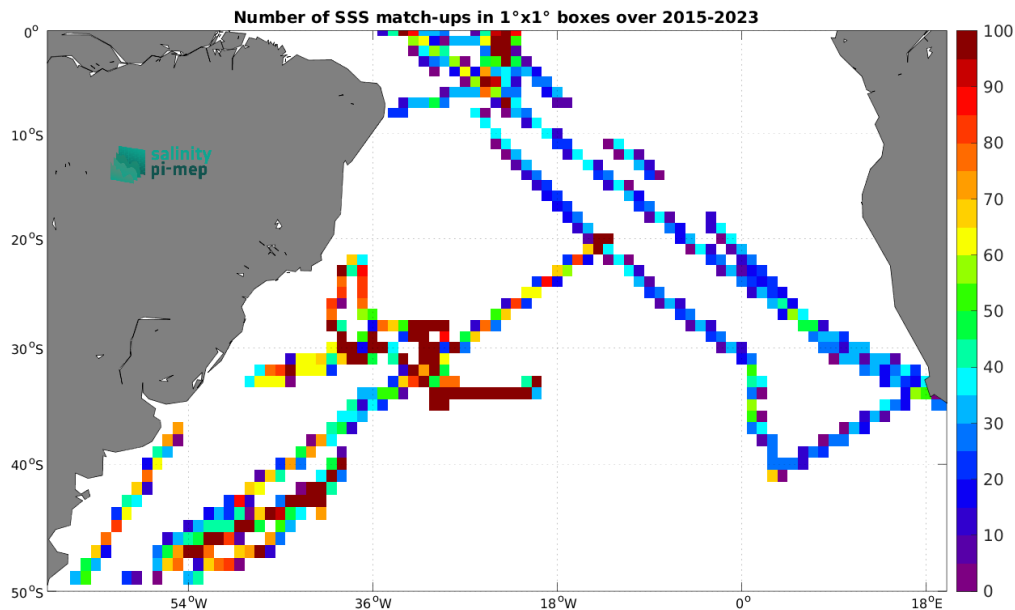
Figure 5: Number of SSS match-ups between TSG (SAMOS) SSS and the SMAP SSS L3 v5.3 - Monthly (RSS) SSS product for the South Atlantic Ocean Pi-MEP region over 1^\circ \times 1^\circ boxes and for the full satellite product period.
