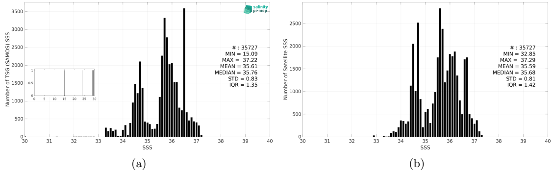
Figure 3: Histograms of SSS from TSG (SAMOS) (a) and SMAP SSS L3 v5.3 - Monthly (RSS) (b) considering all match-up pairs per bins of 0.1 over the South Atlantic Ocean Pi-MEP region and for the full satellite product period.
