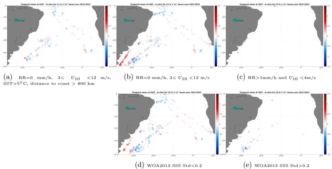
Figure 14: Temporal mean gridded over spatial boxes of size 1^\circ \times 1^\circ of \Delta SSS (SMAP SSS L3 v5.3 - Monthly (RSS) - TSG (SAMOS)) for 5 different subdatasets corresponding to:RR=0 mm/h, 3 < U_{10} < 12 m/s, SST>5°C, distance to coast > 800 km (a), RR=0 mm/h, 3 < U_{10} < 12 m/s (b), RR>1mm/h and U_{10} < 4 m/s (c), WOA2013 SSS Std<0.2 (d), WOA2013 SSS Std>0.2 (e).
