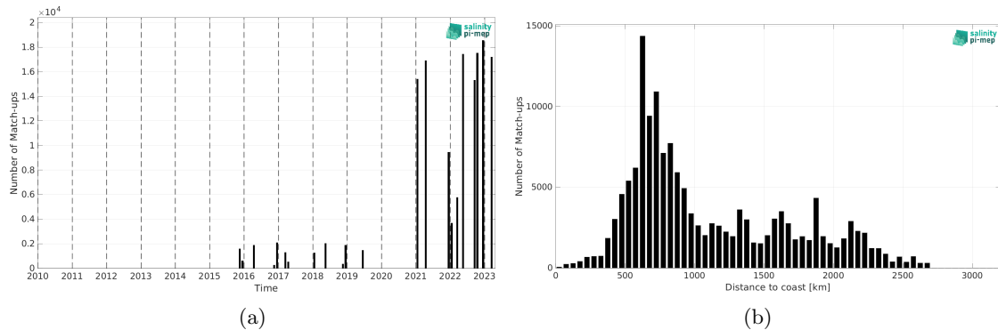
Figure 2: Number of match-ups between TSG (Polarstern) and SMAP SSS L3 v5.3 - Monthly (RSS) SSS as a function of time (a) and as function of the distance to coast (b) over the South Atlantic Ocean Pi-MEP region and for the full satellite product period.
