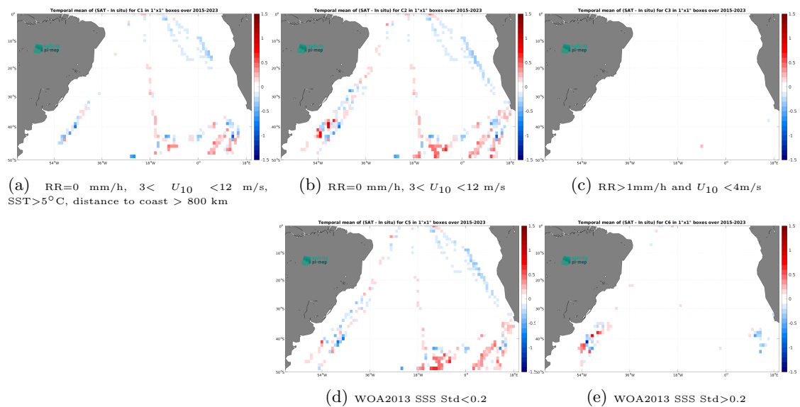
Figure 14: Temporal mean gridded over spatial boxes of size 1^\circ \times 1^\circ of \Delta SSS (SMAP SSS L3 v5.3 - Monthly (RSS) - TSG (Polarstern)) for 5 different subdatasets corresponding to: RR=0 mm/h, 3 < U_{10} < 12 m/s, SST > 5^\circ C , distance to coast > 800 km (a), RR=0 mm/h, 3 < U_{10} < 12 m/s (b), RR > 1 mm/h and U_{10} < 4 m/s (c), WOA2013 SSS Std < 0.2 (d), WOA2013 SSS Std > 0.2 (e).
