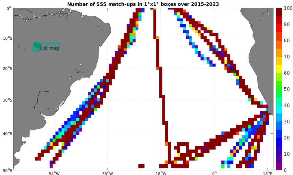
Figure 5: Number of SSS match-ups between TSG (Polarstern) SSS and the SMAP SSS L3 v5.3 - Monthly (RSS) SSS product for the South Atlantic Ocean Pi-MEP region over 1^\circ \times 1^\circ boxes and for the full satellite product period.
