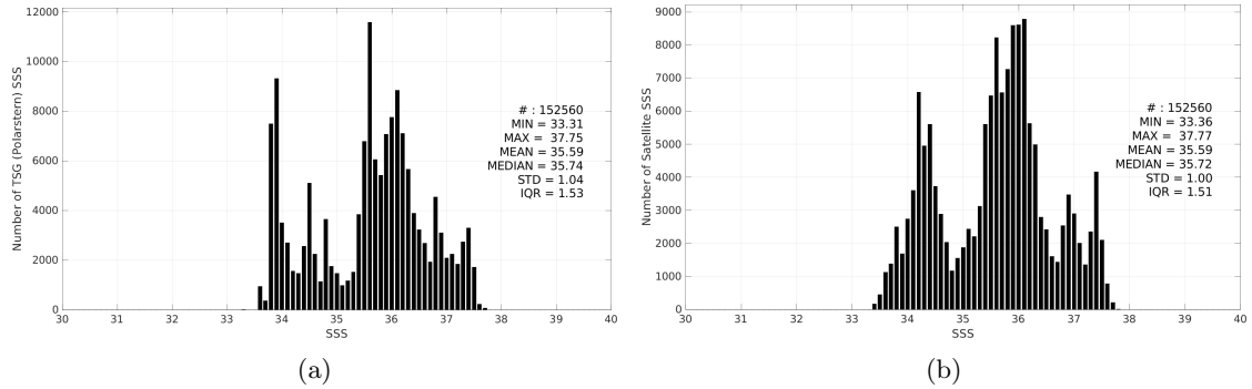
Figure 3: Histograms of SSS from TSG (Polarstern) (a) and SMAP SSS L3 v5.3 - Monthly (RSS) (b) considering all match-up pairs per bins of 0.1 over the South Atlantic Ocean Pi-MEP region and for the full satellite product period.
