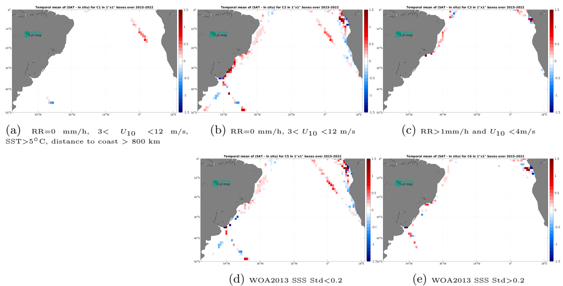
Figure 14: Temporal mean gridded over spatial boxes of size 1^\circ \times 1^\circ of \Delta SSS (SMAP SSS L3 v5.3 - Monthly (RSS) - TSG (LEGOS-DM)) for 5 different subdatasets corresponding to:RR=0 mm/h, 3 < U_{10} < 12 m/s, SST>5°C, distance to coast > 800 km (a), RR=0 mm/h, 3 < U_{10} < 12 m/s (b), RR>1mm/h and U_{10} < 4 m/s (c), WOA2013 SSS Std<0.2 (d), WOA2013 SSS Std>0.2 (e).
