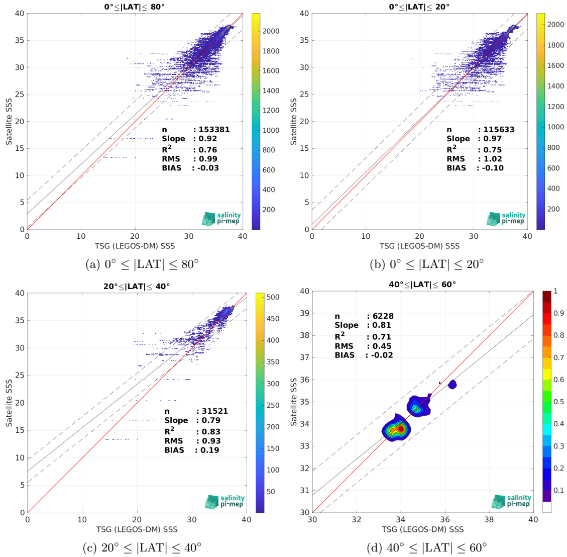
Figure 10: Contour maps of the concentration of SMAP SSS L3 v5.3 - Monthly (RSS) SSS (y-axis) versus TSG (LEGOS-DM) SSS (x-axis) at match-up pairs for different latitude bands. For each plot, the red line shows x=y . The black thin and dashed lines indicate a linear fit through the data cloud and the \pm 95\% confidence levels, respectively. The number match-up pairs n , the slope and R^2 coefficient of the linear fit, the root mean square (RMS) and the mean bias between satellite and in situ data are indicated for each latitude band in each plots.
