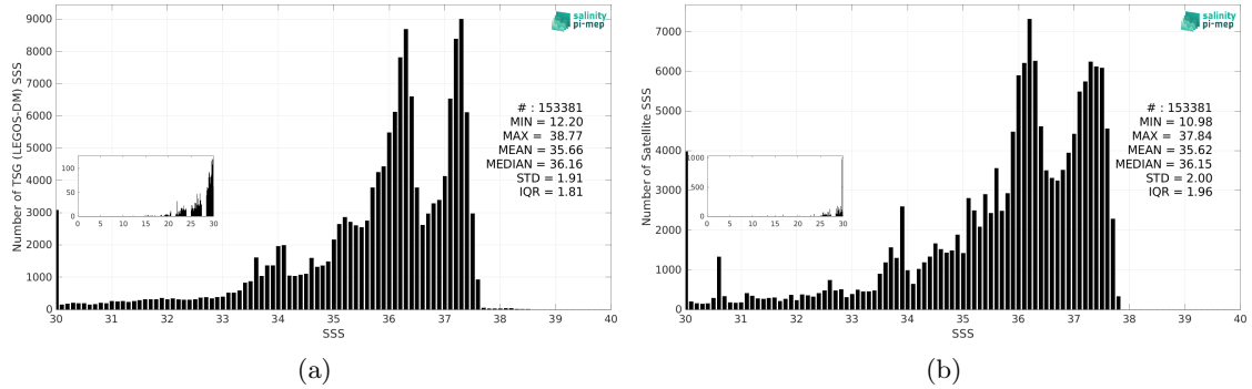
Figure 3: Histograms of SSS from TSG (LEGOS-DM) (a) and SMAP SSS L3 v5.3 - Monthly (RSS) (b) considering all match-up pairs per bins of 0.1 over the South Atlantic Ocean Pi-MEP region and for the full satellite product period.
