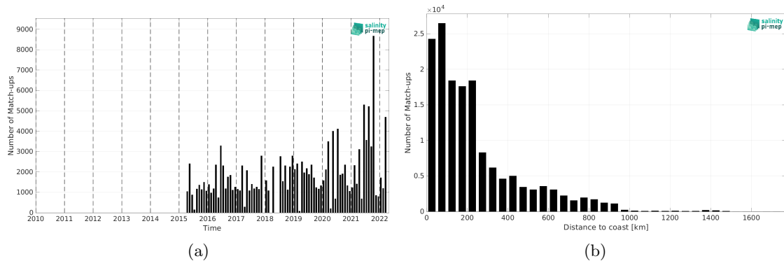
Figure 2: Number of match-ups between TSG (LEGOS-DM) and SMAP SSS L3 v5.3 - Monthly (RSS) SSS as a function of time (a) and as function of the distance to coast (b) over the South Atlantic Ocean Pi-MEP region and for the full satellite product period.
