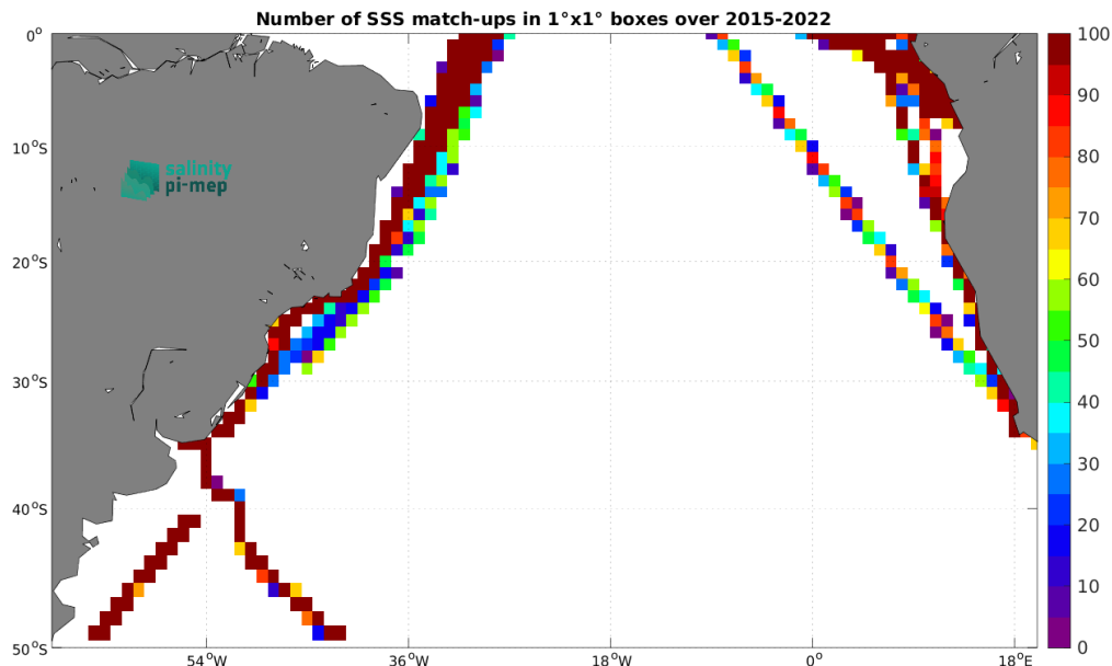
Figure 5: Number of SSS match-ups between TSG (LEGOS-DM) SSS and the SMAP SSS L3 v5.3 - Monthly (RSS) SSS product for the South Atlantic Ocean Pi-MEP region over 1^\circ \times 1^\circ boxes and for the full satellite product period.
