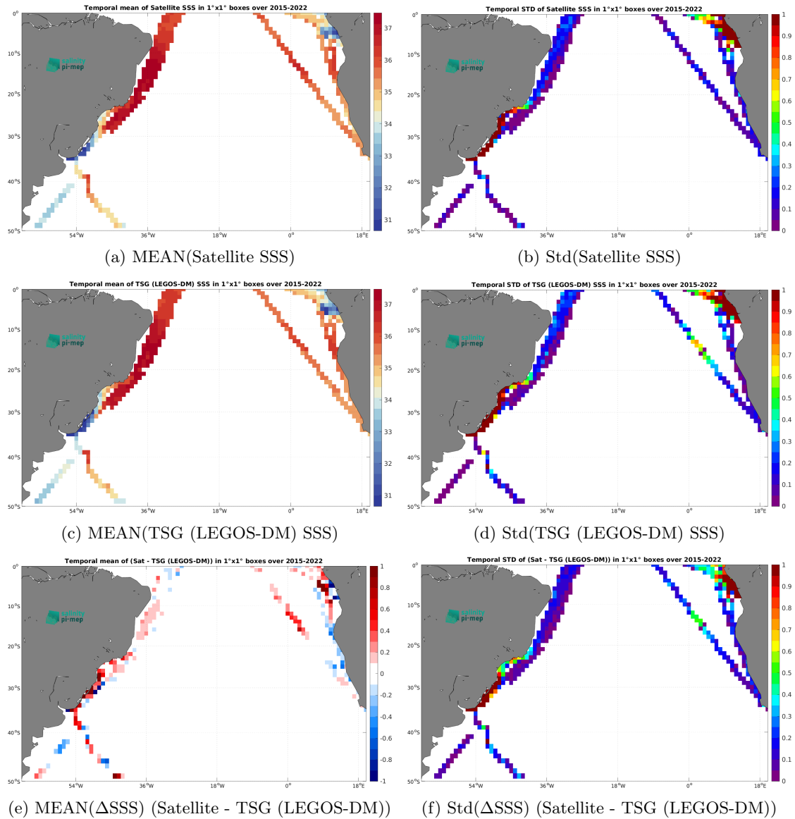
Figure 7: Temporal mean (left) and Std (right) of SSS from SMAP SSS L3 v5.3 - Monthly (RSS) (top), TSG (LEGOS-DM) (middle), and of \Delta SSS (Satellite - TSG (LEGOS-DM)). Only match-up pairs are used to generate these maps.
