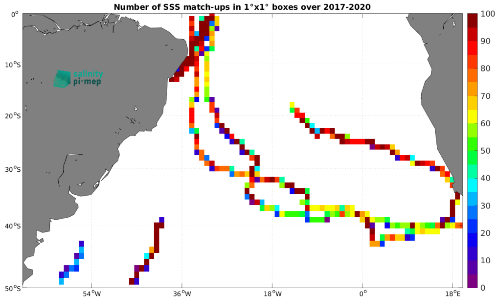
Figure 5: Number of SSS match-ups between TSG (GOSUD-Sailing-ship) SSS and the SMAP SSS L3 v5.3 - Monthly (RSS) SSS product for the South Atlantic Ocean Pi-MEP region over 1^\circ \times 1^\circ boxes and for the full satellite product period.
