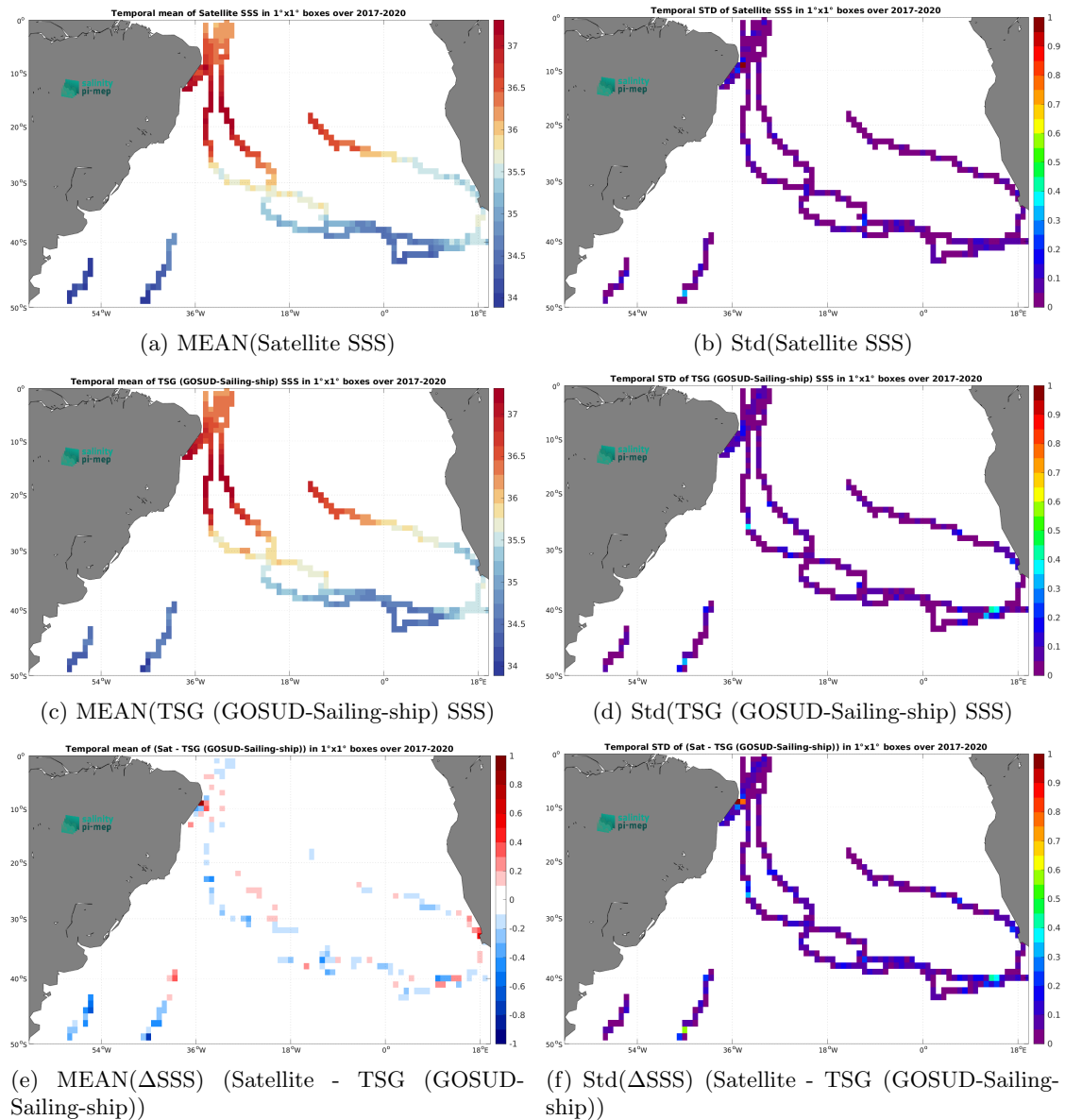
Figure 7: Temporal mean (left) and Std (right) of SSS from SMAP SSS L3 v5.3 - Monthly (RSS) (top), TSG (GOSUD-Sailing-ship) (middle), and of \Delta SSS (Satellite - TSG (GOSUD-Sailing-ship)). Only match-up pairs are used to generate these maps.
