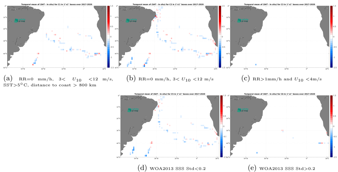
Figure 14: Temporal mean gridded over spatial boxes of size 1^\circ \times 1^\circ of \Delta\text{SSS} (SMAP SSS L3 v5.3 - Monthly (RSS) - TSG (GOSUD-Sailing-ship)) for 5 different subdatasets corresponding to:RR=0 mm/h, 3 < U_{10} < 12 m/s, SST >5^\circ\text{C} , distance to coast > 800 km (a), RR=0 mm/h, 3 < U_{10} < 12 m/s (b), RR >1 mm/h and U_{10} < 4 m/s (c), WOA2013 SSS Std <0.2 (d), WOA2013 SSS Std >0.2 (e).
