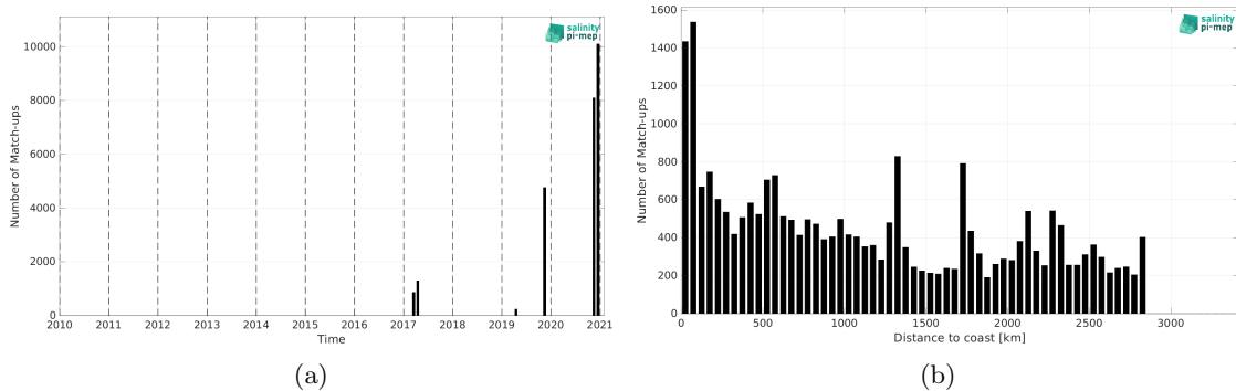
Figure 2: Number of match-ups between TSG (GOSUD-Sailing-ship) and SMAP SSS L3 v5.3 - Monthly (RSS) SSS as a function of time (a) and as function of the distance to coast (b) over the South Atlantic Ocean Pi-MEP region and for the full satellite product period.
