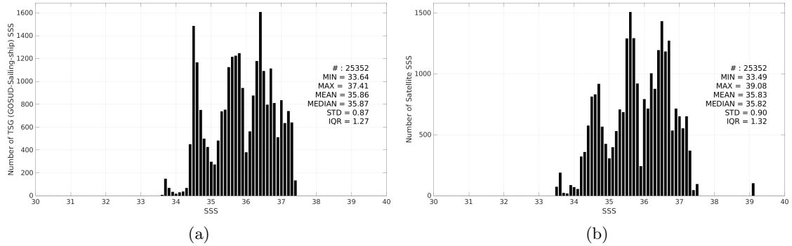
Figure 3: Histograms of SSS from TSG (GOSUD-Sailing-ship) (a) and SMAP SSS L3 v5.3 - Monthly (RSS) (b) considering all match-up pairs per bins of 0.1 over the South Atlantic Ocean Pi-MEP region and for the full satellite product period.
