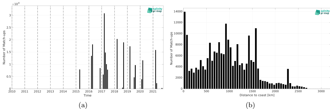
Figure 2: Number of match-ups between TSG (GOSUD-Research-vessel) and SMAP SSS L3 v5.3 - Monthly (RSS) SSS as a function of time (a) and as function of the distance to coast (b) over the South Atlantic Ocean Pi-MEP region and for the full satellite product period.
