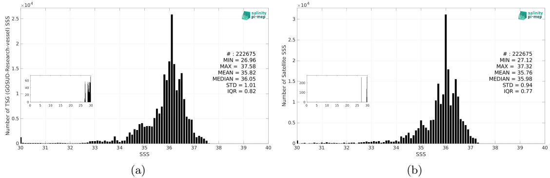
Figure 3: Histograms of SSS from TSG (GOSUD-Research-vessel) (a) and SMAP SSS L3 v5.3 - Monthly (RSS) (b) considering all match-up pairs per bins of 0.1 over the South Atlantic Ocean Pi-MEP region and for the full satellite product period.
