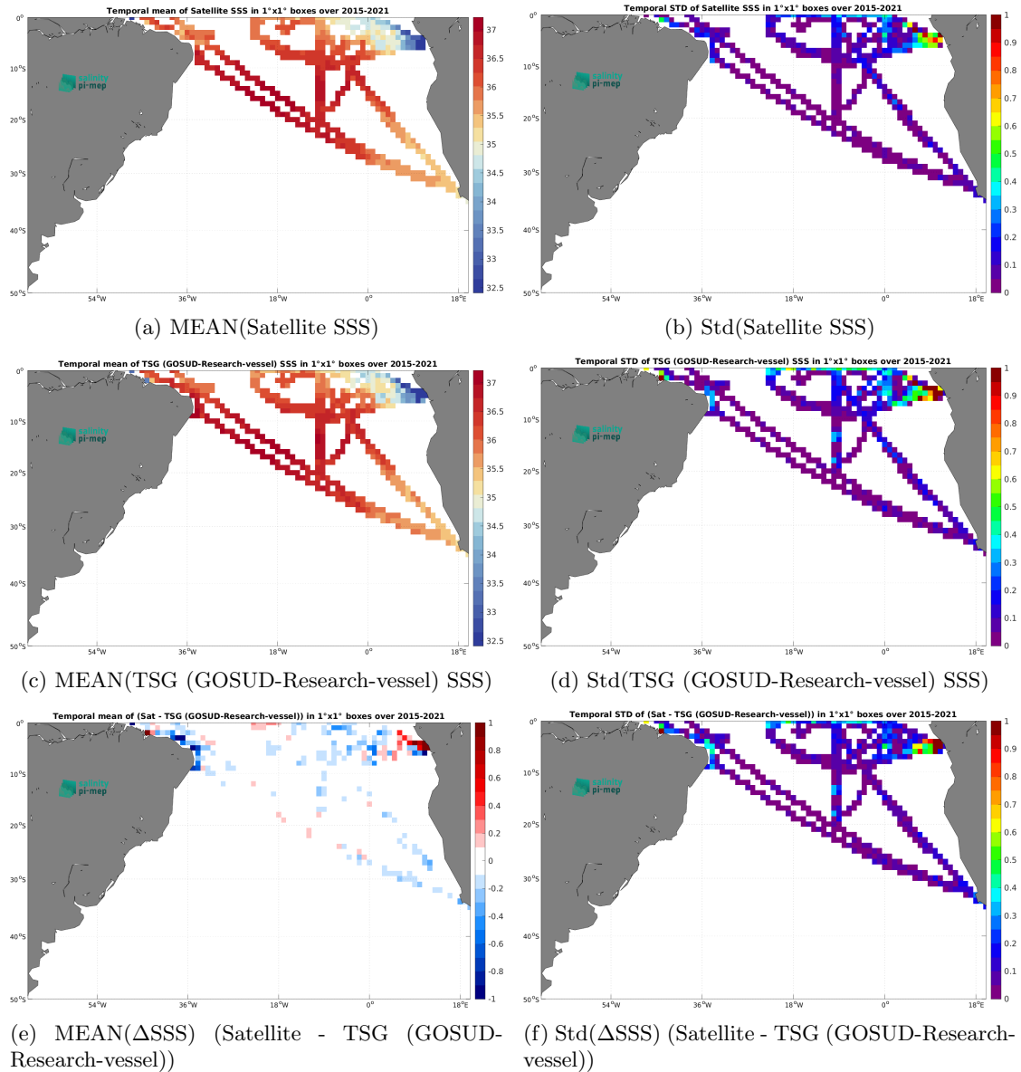
Figure 7: Temporal mean (left) and Std (right) of SSS from SMAP SSS L3 v5.3 - Monthly (RSS) (top), TSG (GOSUD-Research-vessel) (middle), and of \Delta SSS (Satellite - TSG (GOSUD-Research-vessel)). Only match-up pairs are used to generate these maps.
