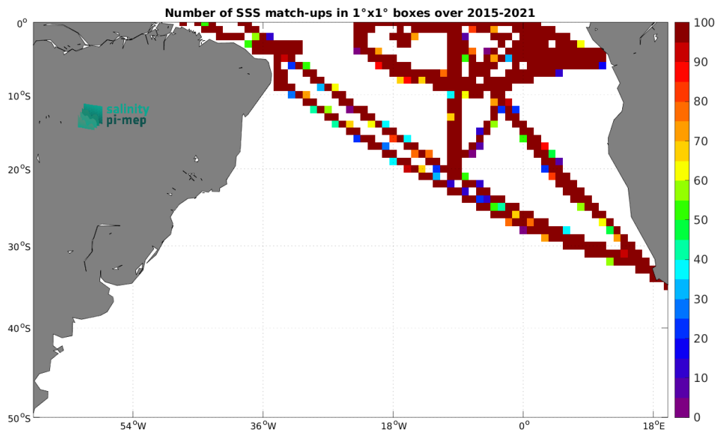
Figure 5: Number of SSS match-ups between TSG (GOSUD-Research-vessel) SSS and the SMAP SSS L3 v5.3 - Monthly (RSS) SSS product for the South Atlantic Ocean Pi-MEP region over 1^\circ \times 1^\circ boxes and for the full satellite product period.
