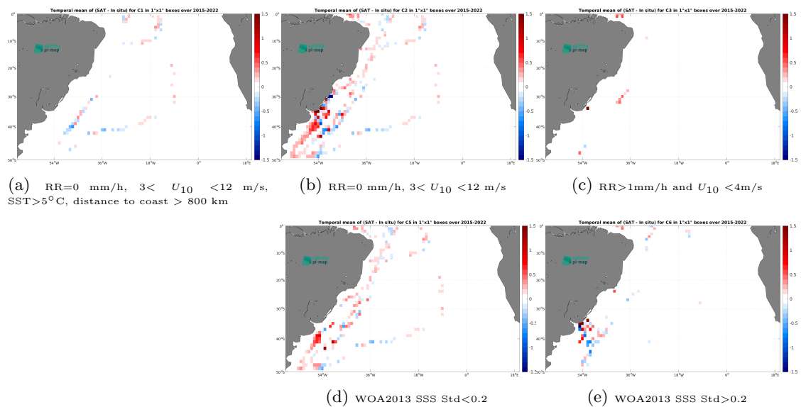
Figure 14: Temporal mean gridded over spatial boxes of size 1^\circ \times 1^\circ of \Delta SSS (SMAP SSS L3 v5.3 - Monthly (RSS) - TSG (CSIC-UTM)) for 5 different subdatasets corresponding to:RR=0 mm/h, 3 < U_{10} < 12 m/s, SST>5°C, distance to coast > 800 km (a), RR=0 mm/h, 3 < U_{10} < 12 m/s (b), RR>1mm/h and U_{10} < 4 m/s (c), WOA2013 SSS Std<0.2 (d), WOA2013 SSS Std>0.2 (e).
