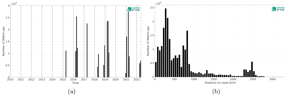
Figure 2: Number of match-ups between TSG (CSIC-UTM) and SMAP SSS L3 v5.3 - Monthly (RSS) SSS as a function of time (a) and as function of the distance to coast (b) over the South Atlantic Ocean Pi-MEP region and for the full satellite product period.
