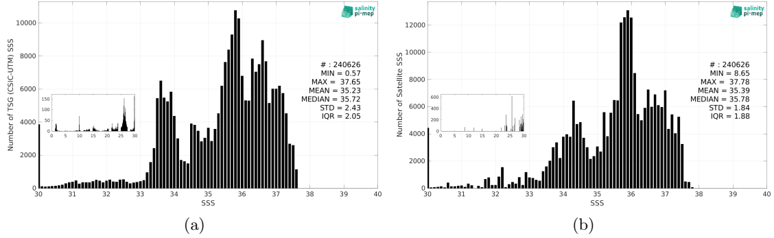
Figure 3: Histograms of SSS from TSG (CSIC-UTM) (a) and SMAP SSS L3 v5.3 - Monthly (RSS) (b) considering all match-up pairs per bins of 0.1 over the South Atlantic Ocean Pi-MEP region and for the full satellite product period.
