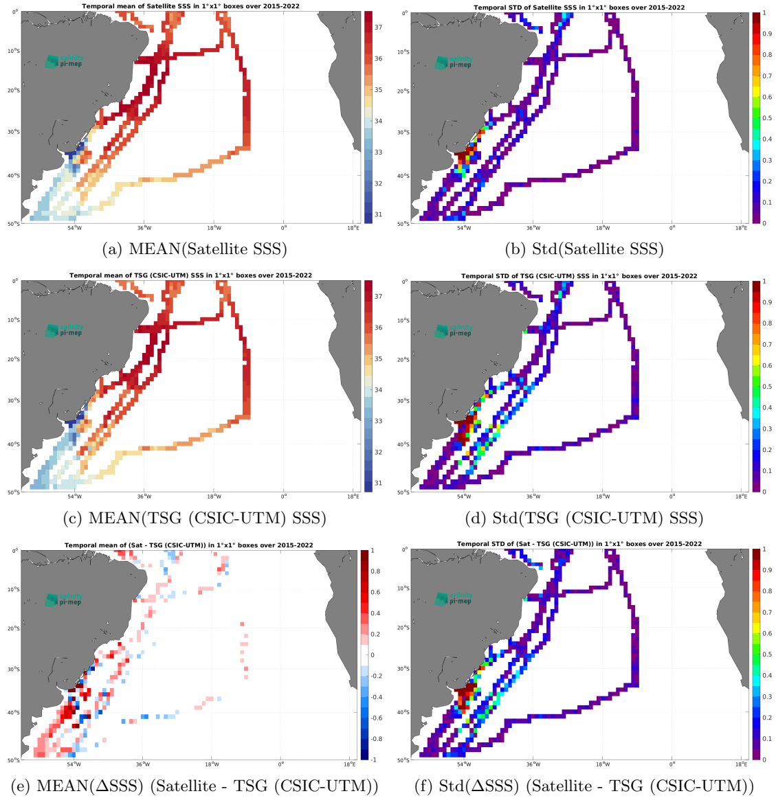
Figure 7: Temporal mean (left) and Std (right) of SSS from SMAP SSS L3 v5.3 - Monthly (RSS) (top), TSG (CSIC-UTM) (middle), and of \Delta SSS (Satellite - TSG (CSIC-UTM)). Only match-up pairs are used to generate these maps.
