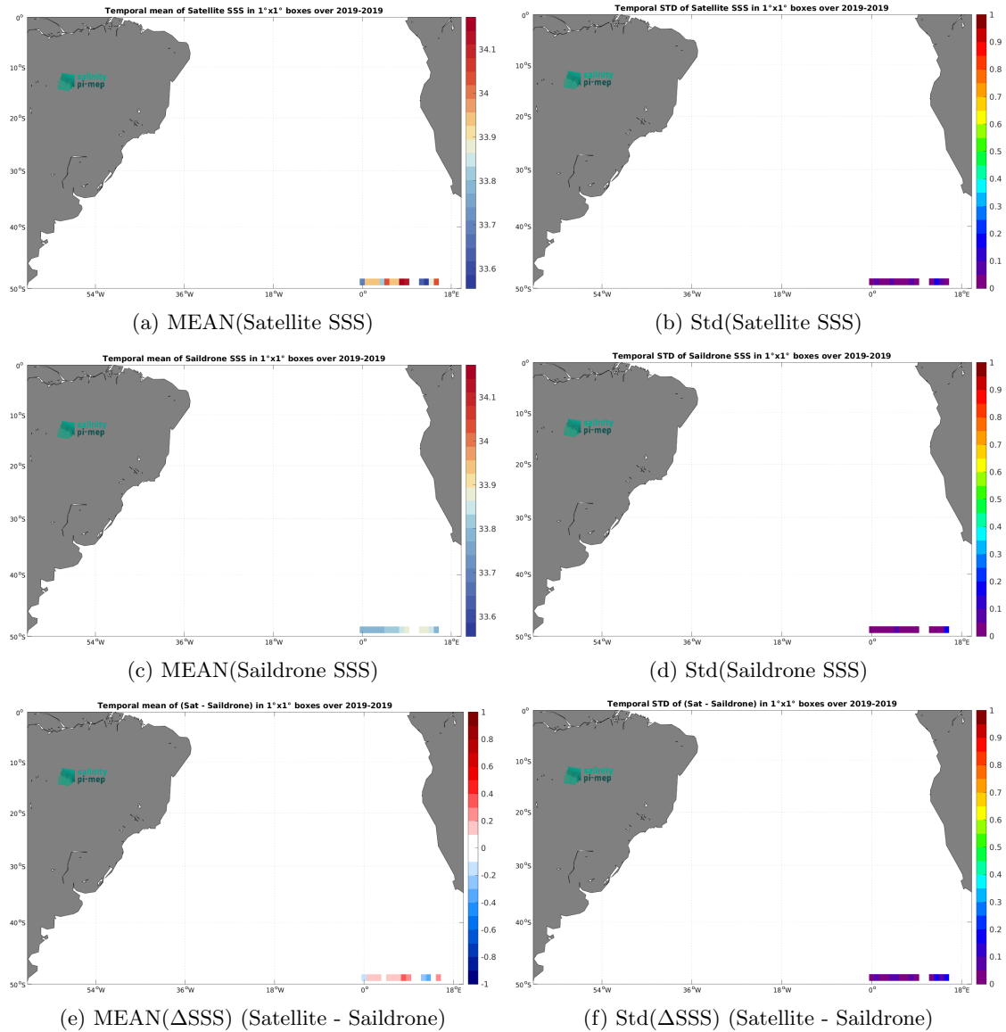
Figure 7: Temporal mean (left) and Std (right) of SSS from SMAP SSS L3 v5.3 - Monthly (RSS) (top), Saildrone (middle), and of \Delta SSS (Satellite - Saildrone). Only match-up pairs are used to generate these maps.
