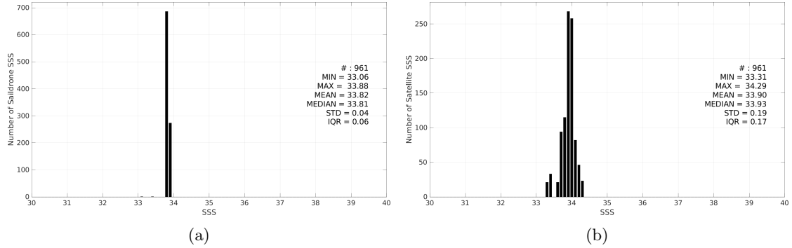
Figure 3: Histograms of SSS from Saildrone (a) and SMAP SSS L3 v5.3 - Monthly (RSS) (b) considering all match-up pairs per bins of 0.1 over the South Atlantic Ocean Pi-MEP region and for the full satellite product period.
