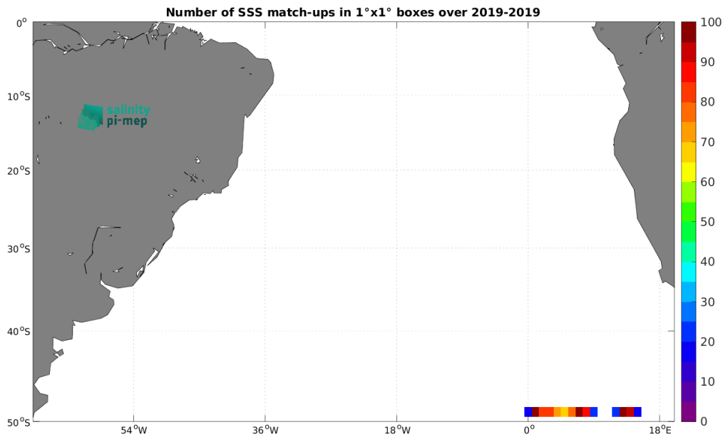
Figure 5: Number of SSS match-ups between Saildrone SSS and the SMAP SSS L3 v5.3 - Monthly (RSS) SSS product for the South Atlantic Ocean Pi-MEP region over 1°×1° boxes and for the full satellite product period.
