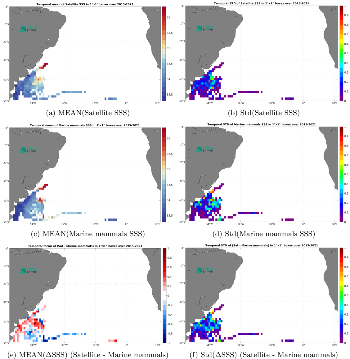
Figure 7: Temporal mean (left) and Std (right) of SSS from SMAP SSS L3 v5.3 - Monthly (RSS) (top), Marine mammals (middle), and of \Delta SSS (Satellite - Marine mammals). Only match-up pairs are used to generate these maps.
