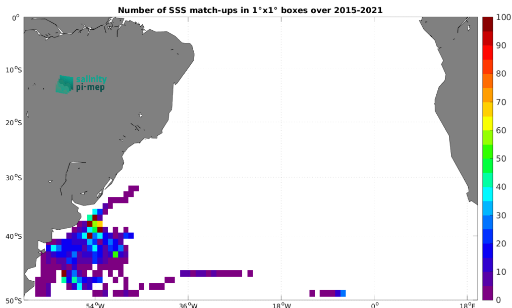
Figure 5: Number of SSS match-ups between Marine mammals SSS and the SMAP SSS L3 v5.3 - Monthly (RSS) SSS product for the South Atlantic Ocean Pi-MEP region over 1^\circ \times 1^\circ boxes and for the full satellite product period.
