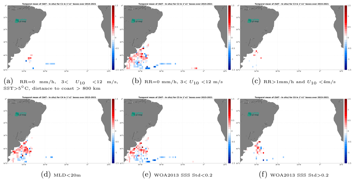
Figure 14: Temporal mean gridded over spatial boxes of size 1^\circ \times 1^\circ of \Delta SSS (SMAP SSS L3 v5.3 - Monthly (RSS) - Marine mammals) for 6 different subdatasets corresponding to:RR=0 mm/h, 3 < U_{10} < 12 m/s, SST > 5^\circ\text{C} , distance to coast > 800 km (a), RR=0 mm/h, 3 < U_{10} < 12 m/s (b), RR > 1 mm/h and U_{10} < 4 m/s (c),MLD < 20 m (d),WOA2013 SSS Std < 0.2 (e),WOA2013 SSS Std > 0.2 (f).
