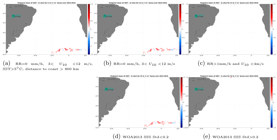
Figure 13: Temporal mean gridded over spatial boxes of size 1^\circ \times 1^\circ of \Delta SSS (SMAP SSS L3 v5.3 - Monthly (RSS) - Surface drifters) for 5 different subdatasets corresponding to:RR=0 mm/h, 3 < U_{10} < 12 m/s, SST >5^\circ\text{C} , distance to coast > 800 km (a), RR=0 mm/h, 3 < U_{10} < 12 m/s (b), RR >1 mm/h and U_{10} < 4 m/s (c), WOA2013 SSS Std <0.2 (d), WOA2013 SSS Std >0.2 (e).
