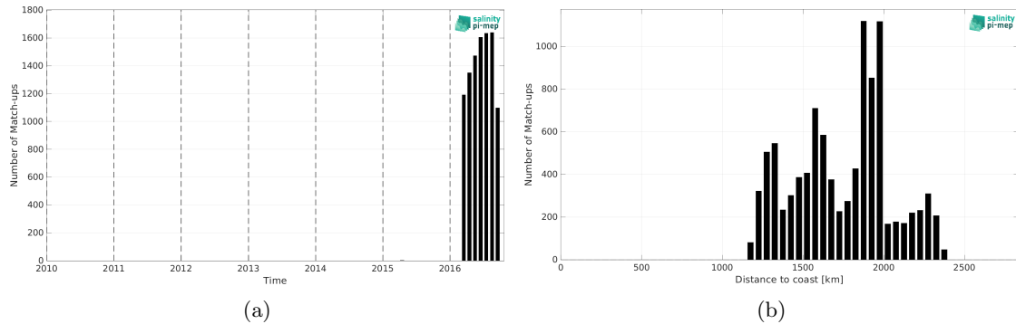
Figure 2: Number of match-ups between Surface drifters and SMAP SSS L3 v5.3 - Monthly (RSS) SSS as a function of time (a) and as function of the distance to coast (b) over the South Atlantic Ocean Pi-MEP region and for the full satellite product period.
