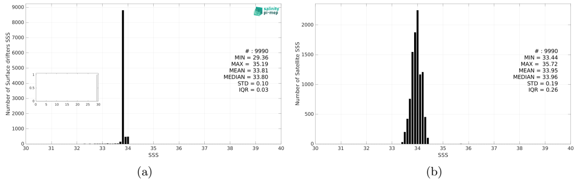
Figure 3: Histograms of SSS from Surface drifters (a) and SMAP SSS L3 v5.3 - Monthly (RSS) (b) considering all match-up pairs per bins of 0.1 over the South Atlantic Ocean Pi-MEP region and for the full satellite product period.
