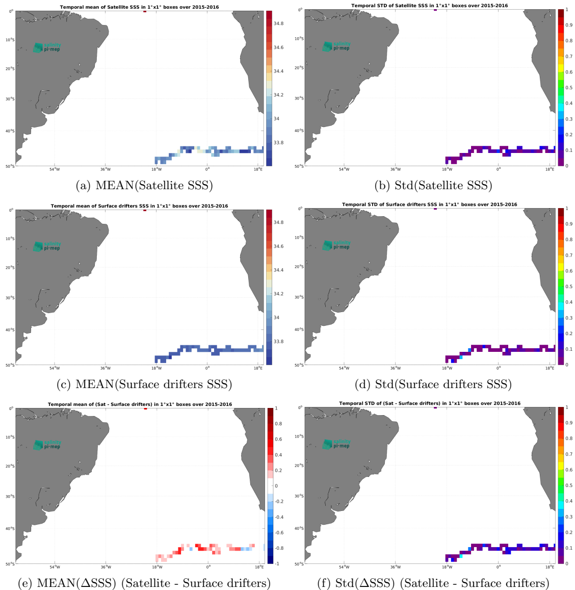
Figure 6: Temporal mean (left) and Std (right) of SSS from SMAP SSS L3 v5.3 - Monthly (RSS) (top), Surface drifters (middle), and of \Delta SSS (Satellite - Surface drifters). Only match-up pairs are used to generate these maps.
