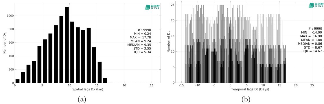
Figure 5: Histograms of the spatial (a) and temporal (b) lags between the location/time of the Surface drifters measurement and the date of the corresponding SMAP SSS L3 v5.3 - Monthly (RSS) SSS pixel.
