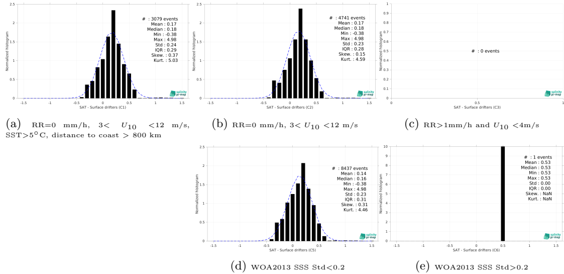
Figure 14: Normalized histogram of \Delta SSS (SMAP SSS L3 v5.3 - Monthly (RSS) - Surface drifters) for 5 different subdatasets corresponding to: RR=0 mm/h, 3 < U_{10} < 12 m/s, SST > 5°C, distance to coast > 800 km (a), RR=0 mm/h, 3 < U_{10} < 12 m/s (b), RR > 1mm/h and U_{10} < 4 m/s (c), WOA2013 SSS Std < 0.2 (d), WOA2013 SSS Std > 0.2 (e).
