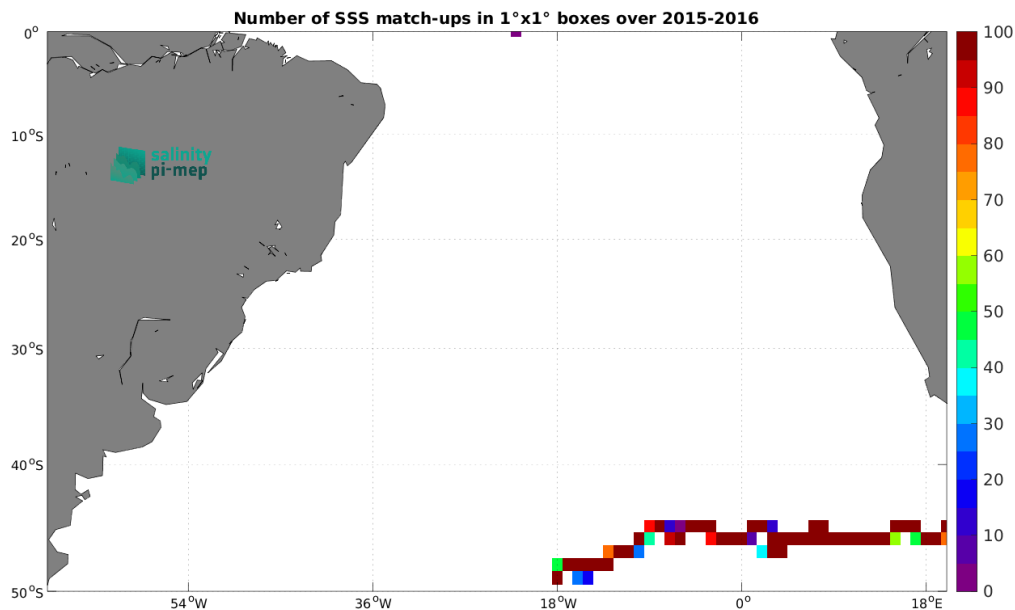
Figure 4: Number of SSS match-ups between Surface drifters SSS and the SMAP SSS L3 v5.3 - Monthly (RSS) SSS product for the South Atlantic Ocean Pi-MEP region over 1^\circ \times 1^\circ boxes and for the full satellite product period.
