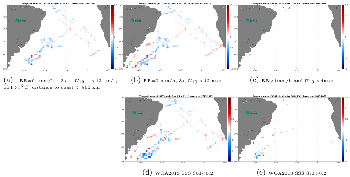
Figure 12: Temporal mean gridded over spatial boxes of size 1^\circ \times 1^\circ of \Delta\text{SSS} (SMAP SSS L3 v5 - 8-Day running (RSS) - TSG (SAMOS)) for 5 different subdatasets corresponding to:RR=0 mm/h, 3 < U_{10} < 12 m/s, SST >5^\circ\text{C} , distance to coast > 800 km (a), RR=0 mm/h, 3 < U_{10} < 12 m/s (b), RR >1 mm/h and U_{10} < 4 m/s (c), WOA2013 SSS Std <0.2 (d), WOA2013 SSS Std >0.2 (e).
