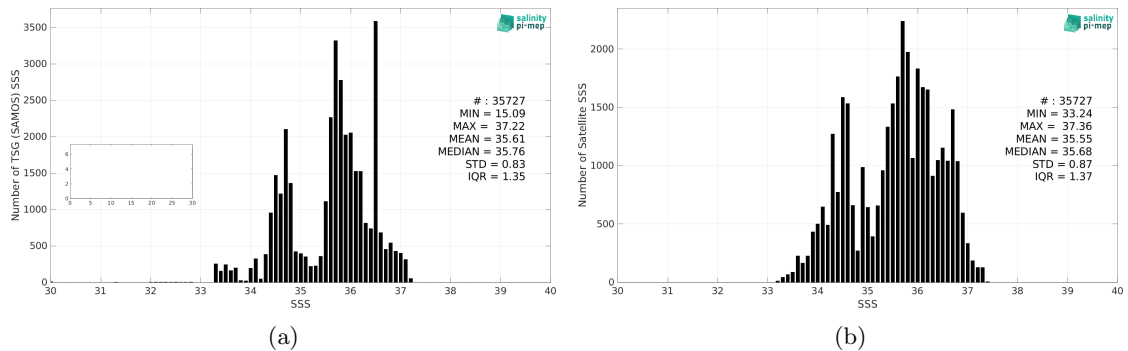
Figure 2: Histograms of SSS from TSG (SAMOS) (a) and SMAP SSS L3 v5 - 8-Day running (RSS) (b) considering all match-up pairs per bins of 0.1 over the South Atlantic Ocean Pi-MEP region and for the full satellite product period.
