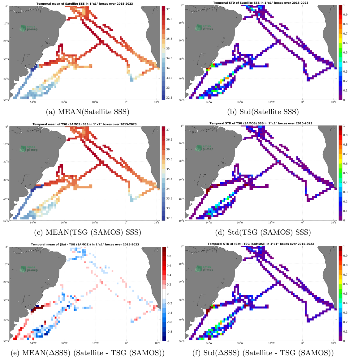
Figure 6: Temporal mean (left) and Std (right) of SSS from SMAP SSS L3 v5 - 8-Day running (RSS) (top), TSG (SAMOS) (middle), and of \Delta SSS (Satellite - TSG (SAMOS)). Only match-up pairs are used to generate these maps.
