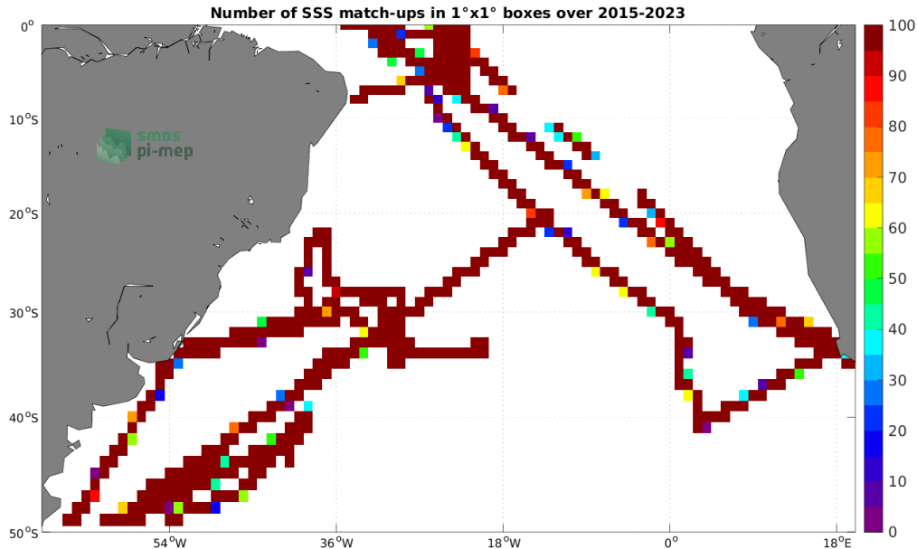
Figure 4: Number of SSS match-ups between TSG (SAMOS) SSS and the SMAP SSS L3 v5 - 8-Day running (RSS) SSS product for the South Atlantic Ocean Pi-MEP region over 1^\circ \times 1^\circ boxes and for the full satellite product period.
