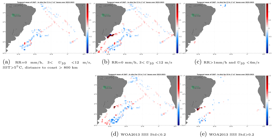
Figure 12: Temporal mean gridded over spatial boxes of size 1^\circ \times 1^\circ of \Delta SSS (SMAP SSS L3 v5 - 8-Day running (RSS) - TSG (SAMOS)) for 5 different subdatasets corresponding to:RR=0 mm/h, 3 < U_{10} < 12 m/s, SST >5^\circ\text{C} , distance to coast > 800 km (a), RR=0 mm/h, 3 < U_{10} < 12 m/s (b), RR >1 mm/h and U_{10} < 4 m/s (c), WOA2013 SSS Std <0.2 (d), WOA2013 SSS Std >0.2 (e).
