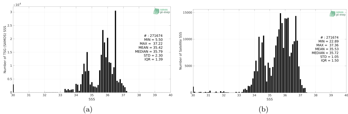
Figure 2: Histograms of SSS from TSG (SAMOS) (a) and SMAP SSS L3 v5 - 8-Day running (RSS) (b) considering all match-up pairs per bins of 0.1 over the South Atlantic Ocean Pi-MEP region and for the full satellite product period.
