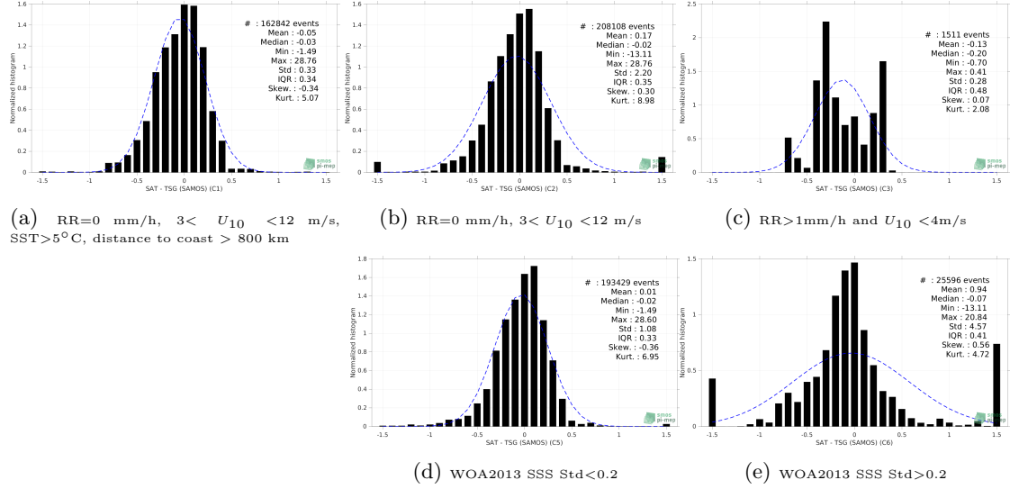
Figure 13: Normalized histogram of \Delta\text{SSS} (SMAP SSS L3 v5 - 8-Day running (RSS) - TSG (SAMOS)) for 5 different subdatasets corresponding to: RR=0 mm/h, 3 < U_{10} < 12 m/s, SST>5°C, distance to coast > 800 km (a), RR=0 mm/h, 3 < U_{10} < 12 m/s (b), RR>1mm/h and U_{10} < 4 m/s (c), WOA2013 SSS Std<0.2 (d), WOA2013 SSS Std>0.2 (e).
