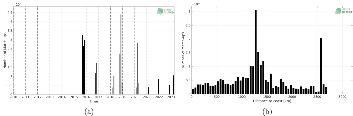
Figure 1: Number of match-ups between TSG (SAMOS) and SMAP SSS L3 v5 - 8-Day running (RSS) SSS as a function of time (a) and as function of the distance to coast (b) over the South Atlantic Ocean Pi-MEP region and for the full satellite product period.
