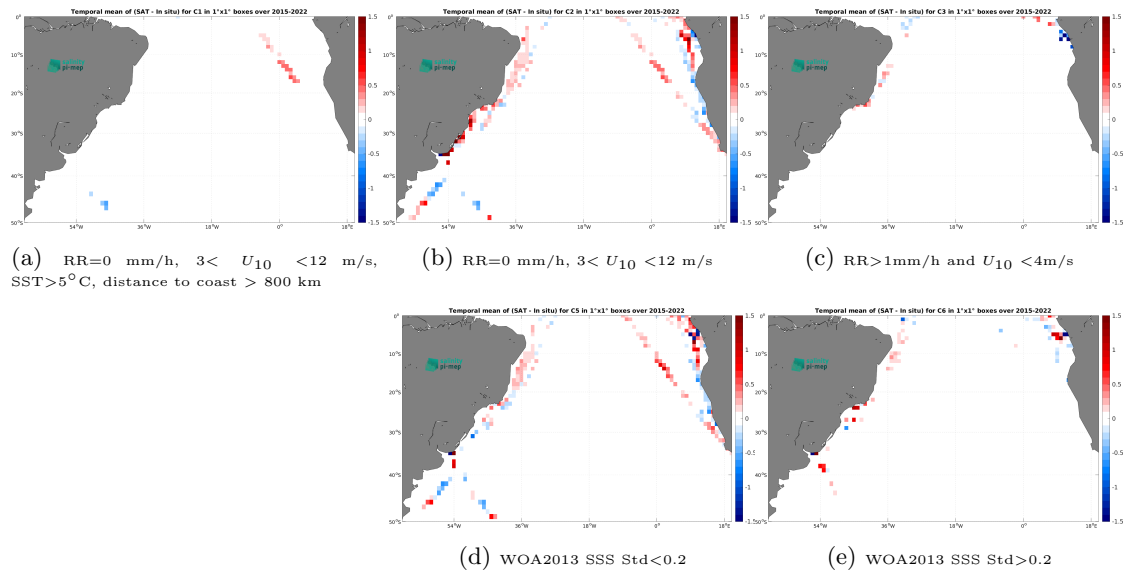
Figure 12: Temporal mean gridded over spatial boxes of size 1^\circ \times 1^\circ of \Delta\text{SSS} (SMAP SSS L3 v5 - 8-Day running (RSS) - TSG (LEGOS-DM)) for 5 different subdatasets corresponding to:RR=0 mm/h, 3 < U_{10} < 12 m/s, SST >5^\circ\text{C} , distance to coast > 800 km (a), RR=0 mm/h, 3 < U_{10} < 12 m/s (b), RR >1 mm/h and U_{10} < 4 m/s (c), WOA2013 SSS Std <0.2 (d), WOA2013 SSS Std >0.2 (e).
