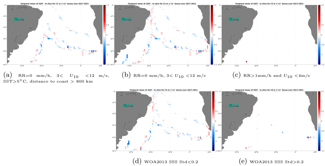
Figure 12: Temporal mean gridded over spatial boxes of size 1^\circ \times 1^\circ of \Delta\text{SSS} (SMAP SSS L3 v5 - 8-Day running (RSS) - TSG (GOSUD-Sailing-ship)) for 5 different subdatasets corresponding to:RR=0 mm/h, 3 < U_{10} < 12 m/s, SST >5^\circ\text{C} , distance to coast > 800 km (a), RR=0 mm/h, 3 < U_{10} < 12 m/s (b), RR >1 mm/h and U_{10} < 4 m/s (c), WOA2013 SSS Std <0.2 (d), WOA2013 SSS Std >0.2 (e).
