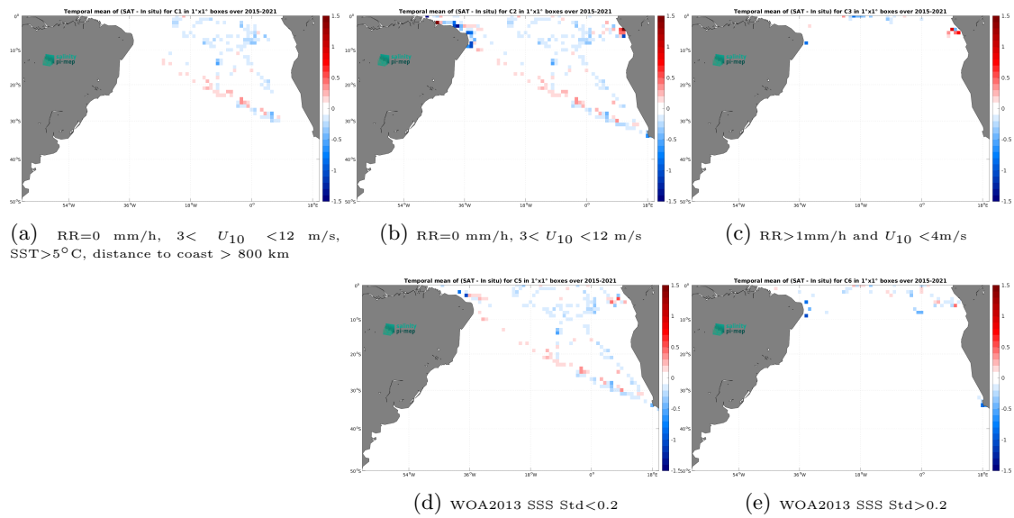
Figure 12: Temporal mean gridded over spatial boxes of size 1^\circ \times 1^\circ of \Delta\text{SSS} (SMAP SSS L3 v5 - 8-Day running (RSS) - TSG (GOSUD-Research-vessel)) for 5 different subdatasets corresponding to:RR=0 mm/h, 3 < U_{10} < 12 m/s, SST >5^\circ\text{C} , distance to coast > 800 km (a), RR=0 mm/h, 3 < U_{10} < 12 m/s (b), RR >1 mm/h and U_{10} < 4 m/s (c), WOA2013 SSS Std <0.2 (d), WOA2013 SSS Std >0.2 (e).
