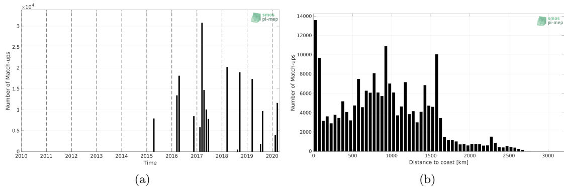
Figure 1: Number of match-ups between TSG (GOSUD-Research-vessel) and SMAP SSS L3 v5 - 8-Day running (RSS) SSS as a function of time (a) and as function of the distance to coast (b) over the South Atlantic Ocean Pi-MEP region and for the full satellite product period.
