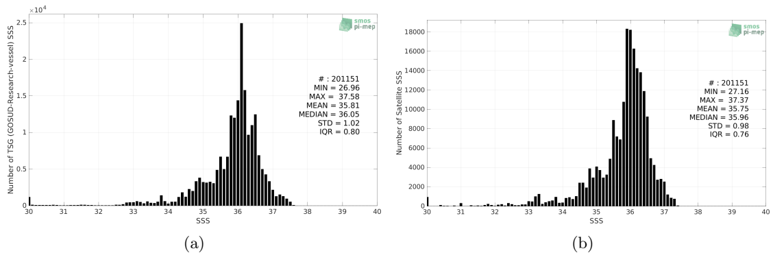
Figure 2: Histograms of SSS from TSG (GOSUD-Research-vessel) (a) and SMAP SSS L3 v5 - 8-Day running (RSS) (b) considering all match-up pairs per bins of 0.1 over the South Atlantic Ocean Pi-MEP region and for the full satellite product period.
