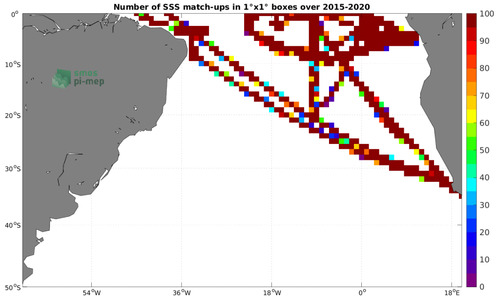
Figure 4: Number of SSS match-ups between TSG (GOSUD-Research-vessel) SSS and the SMAP SSS L3 v5 - 8-Day running (RSS) SSS product for the South Atlantic Ocean Pi-MEP region over 1^\circ \times 1^\circ boxes and for the full satellite product period.
