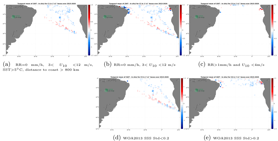
Figure 12: Temporal mean gridded over spatial boxes of size 1^\circ \times 1^\circ of \Delta\text{SSS} (SMAP SSS L3 v5 - 8-Day running (RSS) - TSG (GOSUD-Research-vessel)) for 5 different subdatasets corresponding to:RR=0 mm/h, 3 < U_{10} < 12 m/s, SST >5^\circ\text{C} , distance to coast > 800 km (a), RR=0 mm/h, 3 < U_{10} < 12 m/s (b), RR >1 mm/h and U_{10} < 4 m/s (c), WOA2013 SSS Std <0.2 (d), WOA2013 SSS Std >0.2 (e).
