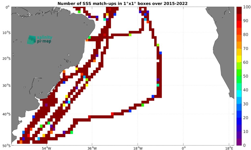
Figure 4: Number of SSS match-ups between TSG (CSIC-UTM) SSS and the SMAP SSS L3 v5 - 8-Day running (RSS) SSS product for the South Atlantic Ocean Pi-MEP region over 1^\circ \times 1^\circ boxes and for the full satellite product period.
