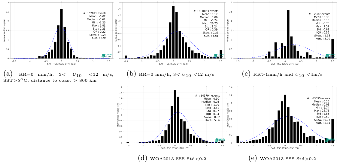
Figure 13: Normalized histogram of \Delta SSS (SMAP SSS L3 v5 - 8-Day running (RSS) - TSG (CSIC-UTM)) for 5 different subdatasets corresponding to: RR=0 mm/h, 3 < U_{10} < 12 m/s, SST > 5°C, distance to coast > 800 km (a), RR=0 mm/h, 3 < U_{10} < 12 m/s (b), RR > 1mm/h and U_{10} < 4 m/s (c), WOA2013 SSS Std < 0.2 (d), WOA2013 SSS Std > 0.2 (e).
