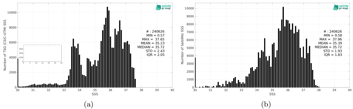
Figure 2: Histograms of SSS from TSG (CSIC-UTM) (a) and SMAP SSS L3 v5 - 8-Day running (RSS) (b) considering all match-up pairs per bins of 0.1 over the South Atlantic Ocean Pi-MEP region and for the full satellite product period.
