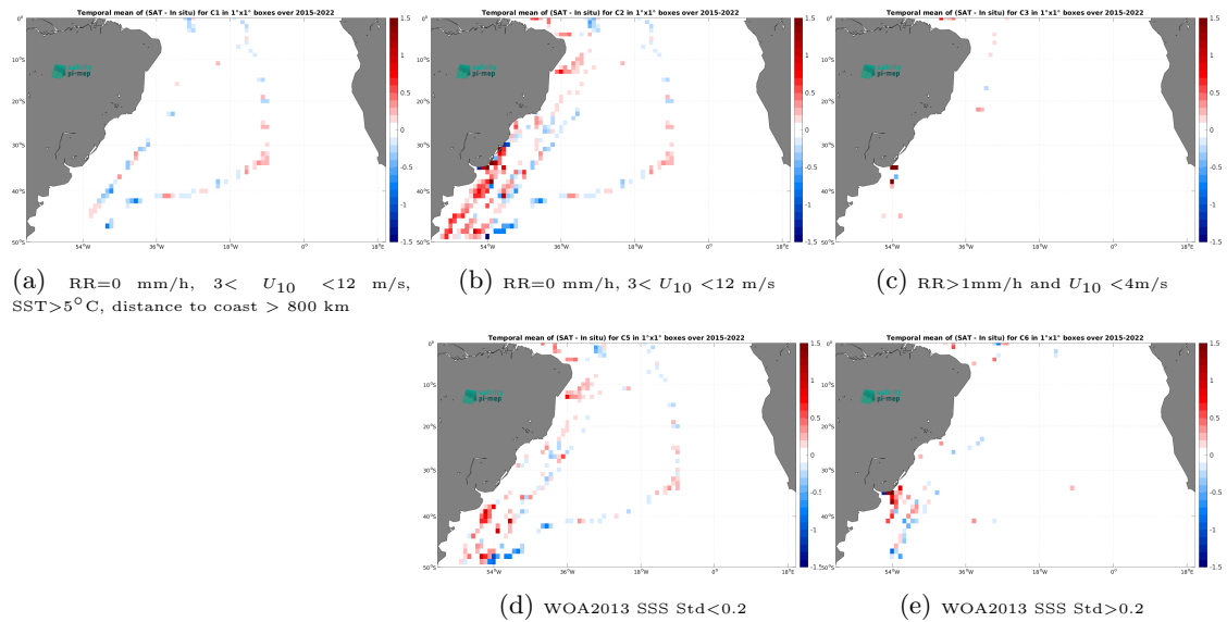
Figure 12: Temporal mean gridded over spatial boxes of size 1^\circ \times 1^\circ of \Delta\text{SSS} (SMAP SSS L3 v5 - 8-Day running (RSS) - TSG (CSIC-UTM)) for 5 different subdatasets corresponding to:RR=0 mm/h, 3 < U_{10} < 12 m/s, SST >5^\circ\text{C} , distance to coast > 800 km (a), RR=0 mm/h, 3 < U_{10} < 12 m/s (b), RR >1 mm/h and U_{10} < 4 m/s (c), WOA2013 SSS Std <0.2 (d), WOA2013 SSS Std >0.2 (e).
