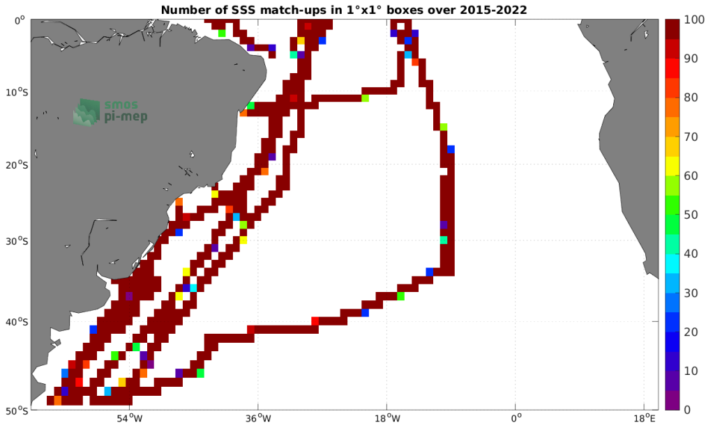
Figure 4: Number of SSS match-ups between TSG (CSIC-UTM) SSS and the SMAP SSS L3 v5 - 8-Day running (RSS) SSS product for the South Atlantic Ocean Pi-MEP region over 1^{\circ} \times 1^{\circ} boxes and for the full satellite product period.
