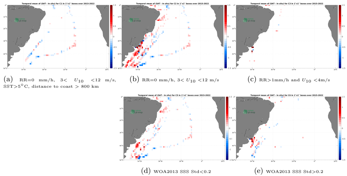
Figure 12: Temporal mean gridded over spatial boxes of size 1^\circ \times 1^\circ of \Delta SSS (SMAP SSS L3 v5 - 8-Day running (RSS) - TSG (CSIC-UTM)) for 5 different subdatasets corresponding to:RR=0 mm/h, 3 < U_{10} < 12 m/s, SST >5^\circ\text{C} , distance to coast > 800 km (a), RR=0 mm/h, 3 < U_{10} < 12 m/s (b), RR >1 mm/h and U_{10} < 4 m/s (c), WOA2013 SSS Std <0.2 (d), WOA2013 SSS Std >0.2 (e).
