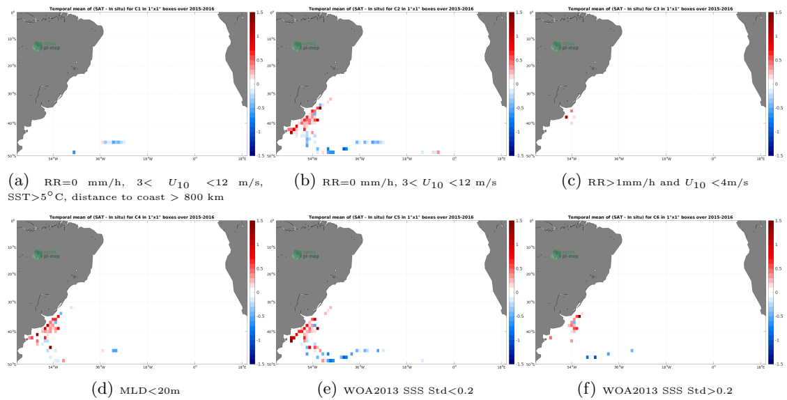
Figure 12: Temporal mean gridded over spatial boxes of size 1^\circ \times 1^\circ of \Delta SSS (SMAP SSS L3 v5 - 8-Day running (RSS) - Marine mammals) for 6 different subdatasets corresponding to:RR=0 mm/h, 3 < U_{10} < 12 m/s, SST >5^\circ C, distance to coast > 800 km (a), RR=0 mm/h, 3 < U_{10} < 12 m/s (b), RR >1 mm/h and U_{10} < 4 m/s (c),MLD <20 m (d),WOA2013 SSS Std <0.2 (e),WOA2013 SSS Std >0.2 (f).
