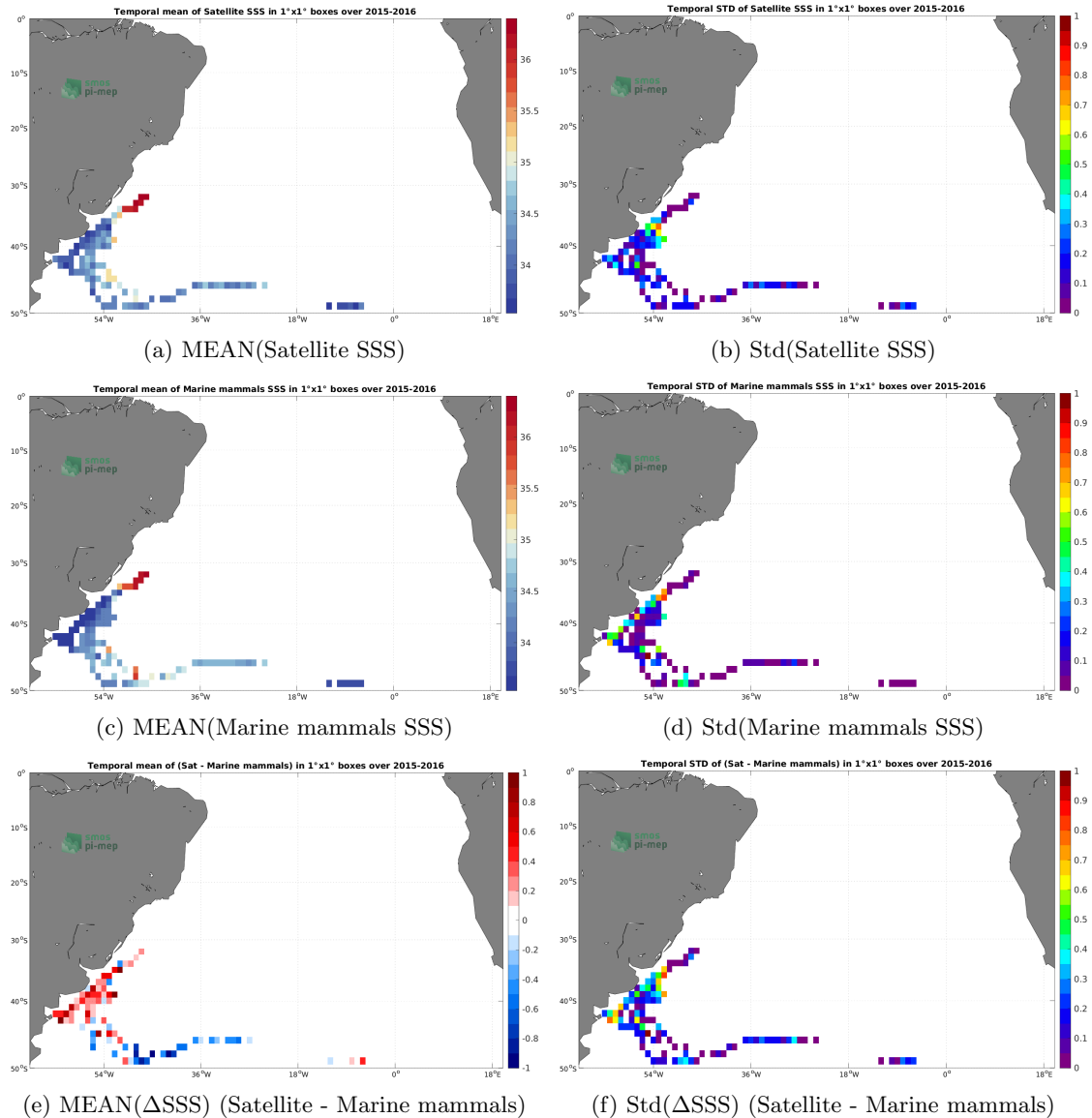
Figure 6: Temporal mean (left) and Std (right) of SSS from SMAP SSS L3 v5 - 8-Day running (RSS) (top), Marine mammals (middle), and of \Delta SSS (Satellite - Marine mammals). Only match-up pairs are used to generate these maps.
