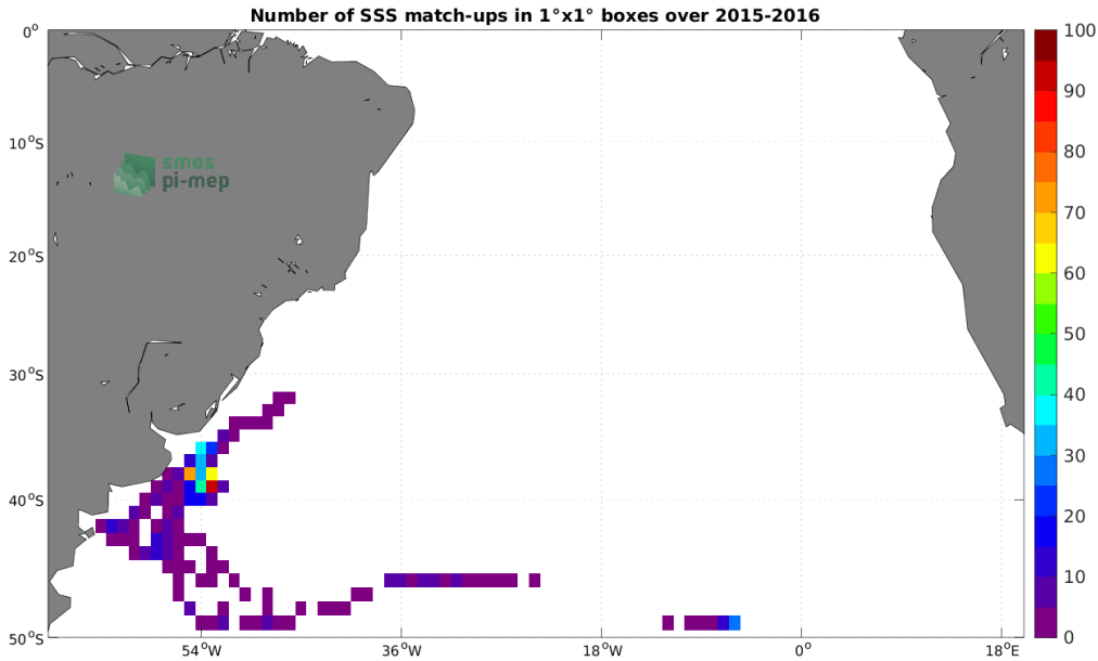
Figure 4: Number of SSS match-ups between Marine mammals SSS and the SMAP SSS L3 v5 - 8-Day running (RSS) SSS product for the South Atlantic Ocean Pi-MEP region over 1^\circ \times 1^\circ boxes and for the full satellite product period.
