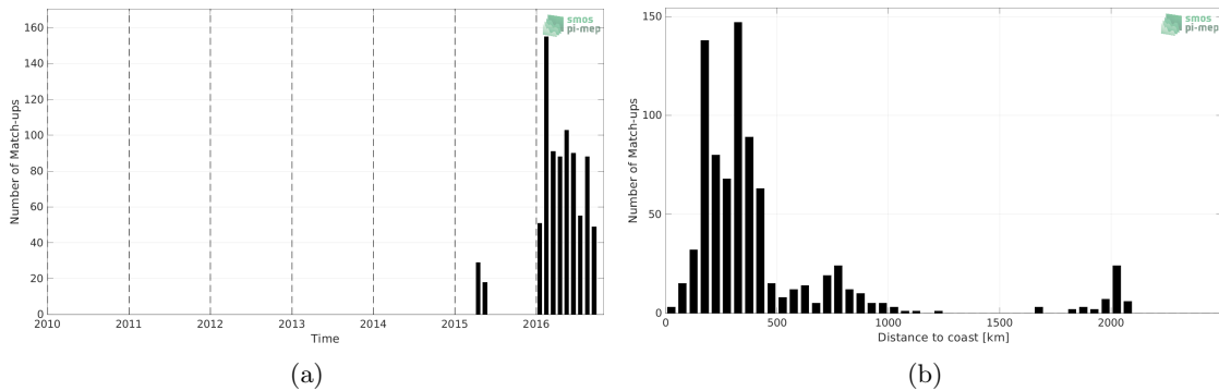
Figure 1: Number of match-ups between Marine mammals and SMAP SSS L3 v5 - 8-Day running (RSS) SSS as a function of time (a) and as function of the distance to coast (b) over the South Atlantic Ocean Pi-MEP region and for the full satellite product period.
