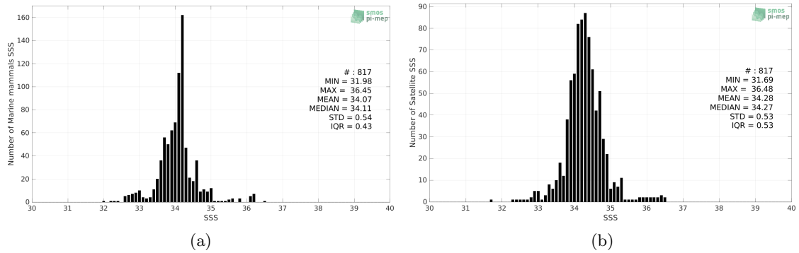
Figure 2: Histograms of SSS from Marine mammals (a) and SMAP SSS L3 v5 - 8-Day running (RSS) (b) considering all match-up pairs per bins of 0.1 over the South Atlantic Ocean Pi-MEP region and for the full satellite product period.
