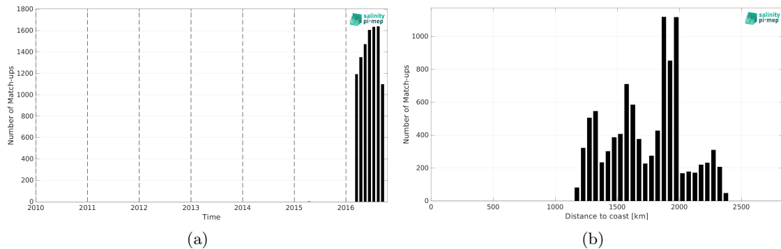
Figure 1: Number of match-ups between Surface drifters and SMAP SSS L3 v5 - 8-Day running (RSS) SSS as a function of time (a) and as function of the distance to coast (b) over the South Atlantic Ocean Pi-MEP region and for the full satellite product period.
