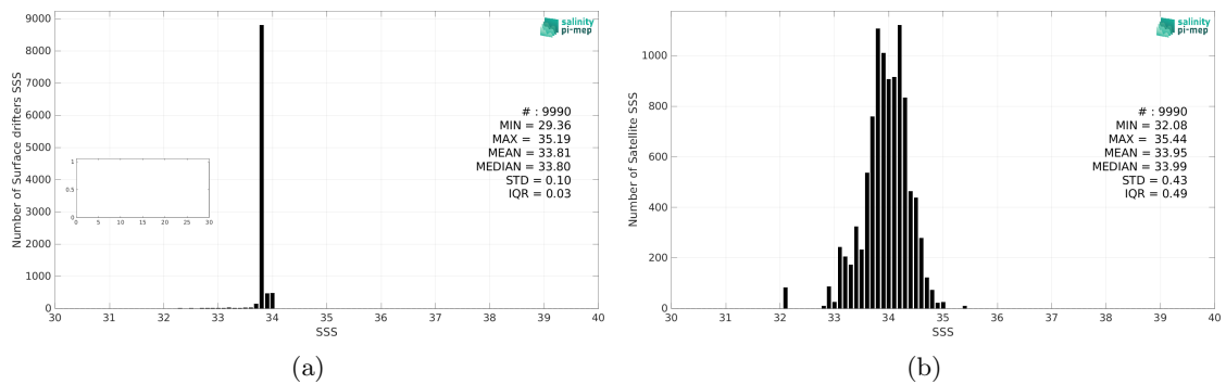
Figure 2: Histograms of SSS from Surface drifters (a) and SMAP SSS L3 v5 - 8-Day running (RSS) (b) considering all match-up pairs per bins of 0.1 over the South Atlantic Ocean Pi-MEP region and for the full satellite product period.
