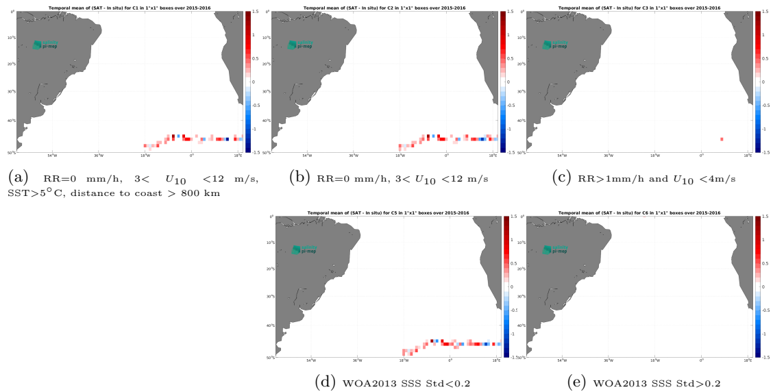
Figure 11: Temporal mean gridded over spatial boxes of size 1^\circ \times 1^\circ of \Delta SSS (SMAP SSS L3 v5 - 8-Day running (RSS) - Surface drifters) for 5 different subdatasets corresponding to:RR=0 mm/h, 3 < U_{10} < 12 m/s, SST >5^\circ\text{C} , distance to coast > 800 km (a), RR=0 mm/h, 3 < U_{10} < 12 m/s (b), RR >1 mm/h and U_{10} < 4 m/s (c), WOA2013 SSS Std <0.2 (d), WOA2013 SSS Std >0.2 (e).
