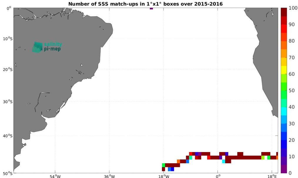
Figure 3: Number of SSS match-ups between Surface drifters SSS and the SMAP SSS L3 v5 - 8-Day running (RSS) SSS product for the South Atlantic Ocean Pi-MEP region over 1^\circ \times 1^\circ boxes and for the full satellite product period.
