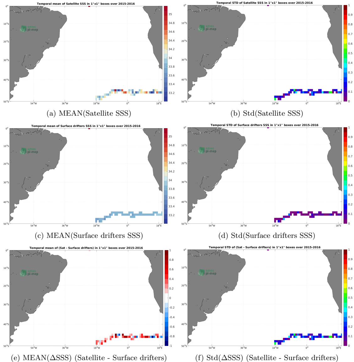
Figure 5: Temporal mean (left) and Std (right) of SSS from SMAP SSS L3 v5 - 8-Day running (RSS) (top), Surface drifters (middle), and of \Delta SSS (Satellite - Surface drifters). Only match-up pairs are used to generate these maps.
