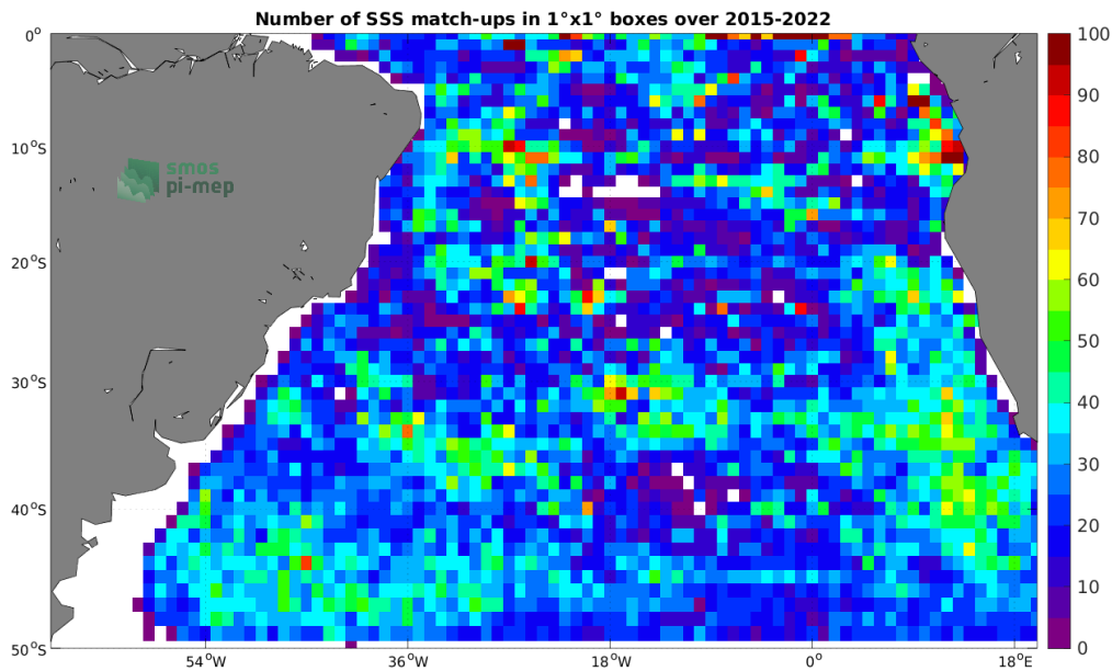
Figure 4: Number of SSS match-ups between Argo SSS and the SMAP SSS L3 v5 - 8-Day running (RSS) SSS product for the South Atlantic Ocean Pi-MEP region over 1^\circ \times 1^\circ boxes and for the full satellite product period.
