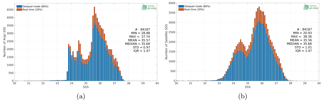
Figure 2: Histograms of SSS from Argo (a) and SMAP SSS L3 v5 - 8-Day running (RSS) (b) considering all match-up pairs per bins of 0.1 over the South Atlantic Ocean Pi-MEP region and for the full satellite product period.
