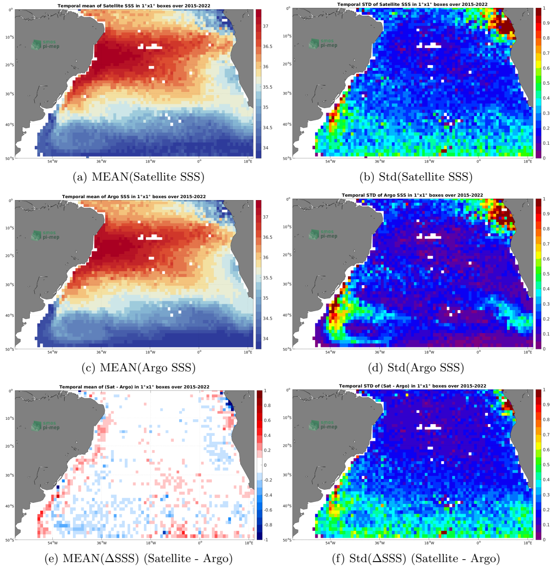
Figure 6: Temporal mean (left) and Std (right) of SSS from SMAP SSS L3 v5 - 8-Day running (RSS) (top), Argo (middle), and of \Delta SSS (Satellite - Argo). Only match-up pairs are used to generate these maps.
