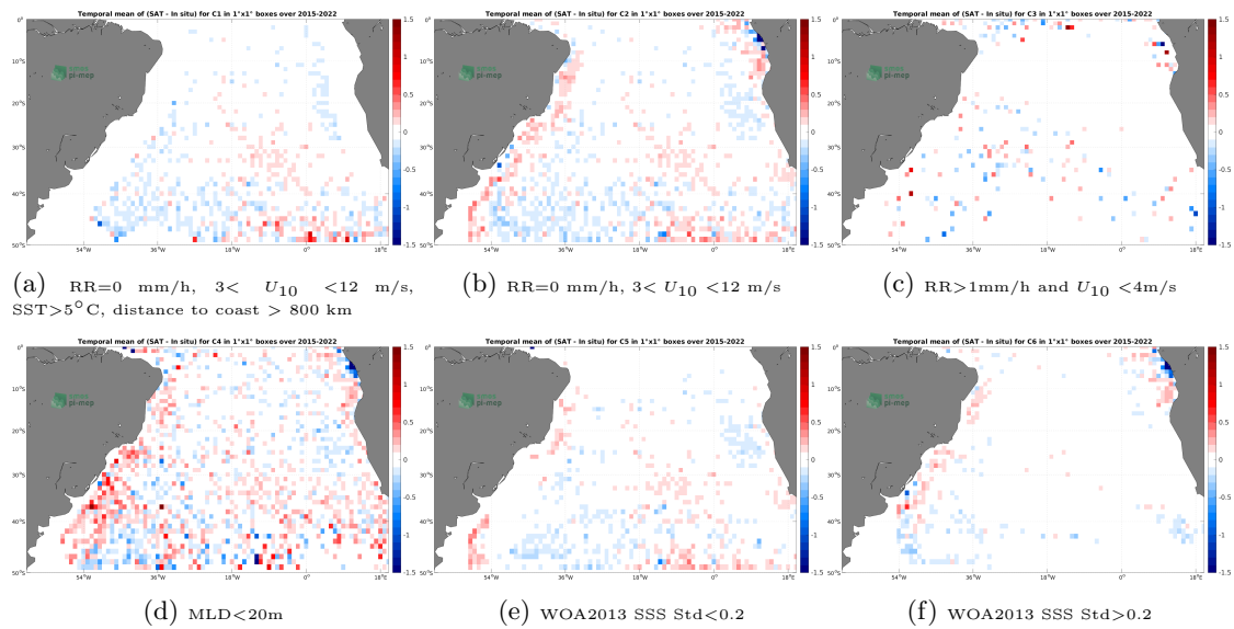
Figure 12: Temporal mean gridded over spatial boxes of size 1^\circ \times 1^\circ of \Delta SSS (SMAP SSS L3 v5 - 8-Day running (RSS) - Argo) for 6 different subdatasets corresponding to:RR=0 mm/h, 3 < U_{10} < 12 m/s, SST >5^\circ C, distance to coast > 800 km (a), RR=0 mm/h, 3 < U_{10} < 12 m/s (b), RR >1 mm/h and U_{10} < 4 m/s (c),MLD <20 m (d),WOA2013 SSS Std <0.2 (e),WOA2013 SSS Std >0.2 (f).
