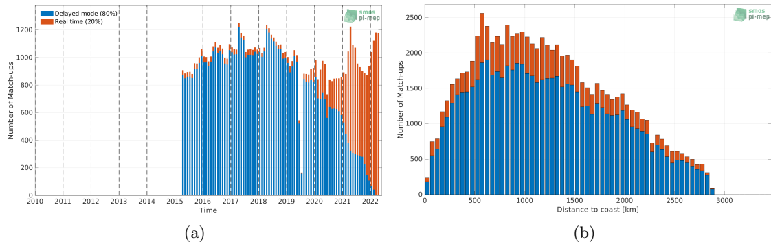
Figure 1: Number of match-ups between Argo and SMAP SSS L3 v5 - 8-Day running (RSS) SSS as a function of time (a) and as function of the distance to coast (b) over the South Atlantic Ocean Pi-MEP region and for the full satellite product period.
