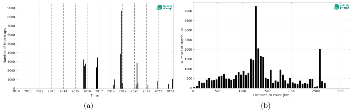
Figure 1: Number of match-ups between TSG (SAMOS) and SMAP SSS L3 v5 - Monthly (RSS) SSS as a function of time (a) and as function of the distance to coast (b) over the South Atlantic Ocean Pi-MEP region and for the full satellite product period.
