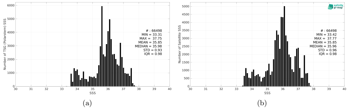
Figure 2: Histograms of SSS from TSG (Polarstern) (a) and SMAP SSS L3 v5 - Monthly (RSS) (b) considering all match-up pairs per bins of 0.1 over the South Atlantic Ocean Pi-MEP region and for the full satellite product period.
