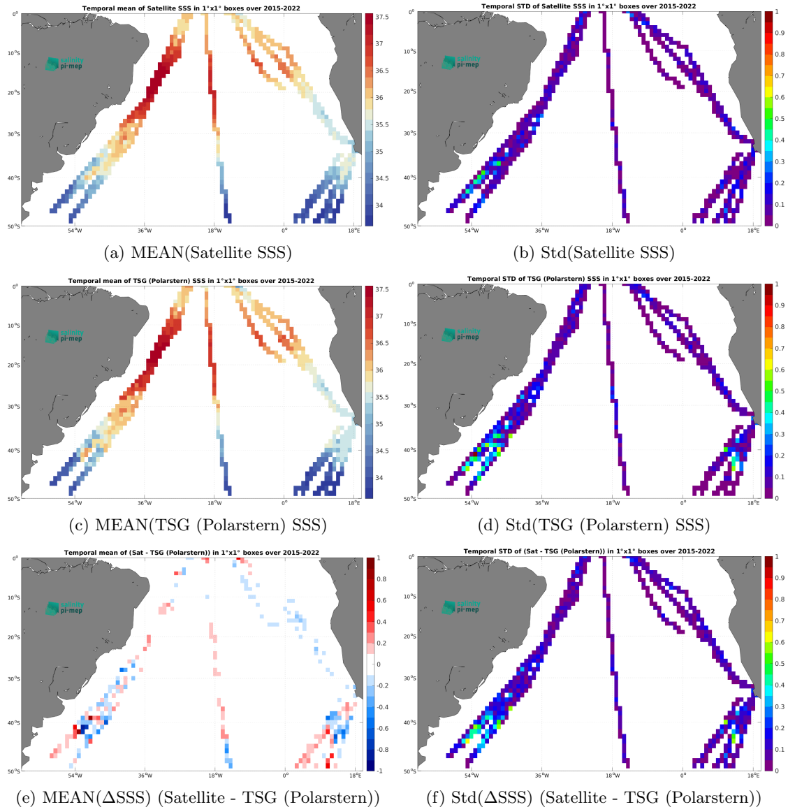
Figure 6: Temporal mean (left) and Std (right) of SSS from SMAP SSS L3 v5 - Monthly (RSS) (top), TSG (Polarstern) (middle), and of \Delta SSS (Satellite - TSG (Polarstern)). Only match-up pairs are used to generate these maps.
