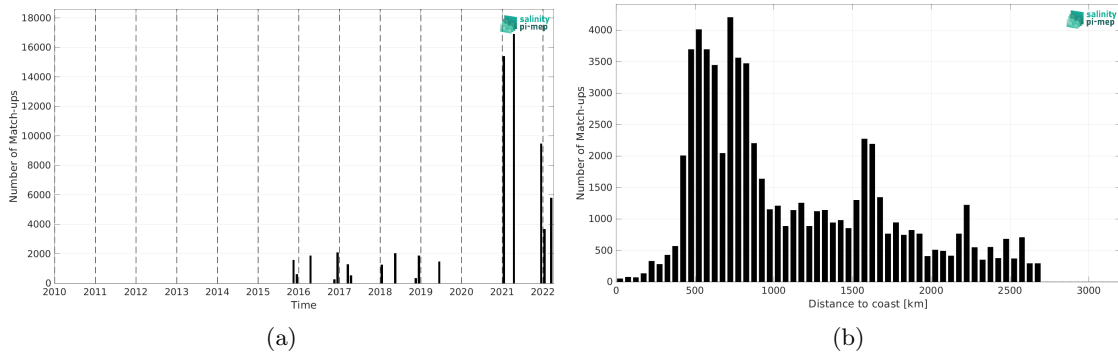
Figure 1: Number of match-ups between TSG (Polarstern) and SMAP SSS L3 v5 - Monthly (RSS) SSS as a function of time (a) and as function of the distance to coast (b) over the South Atlantic Ocean Pi-MEP region and for the full satellite product period.
