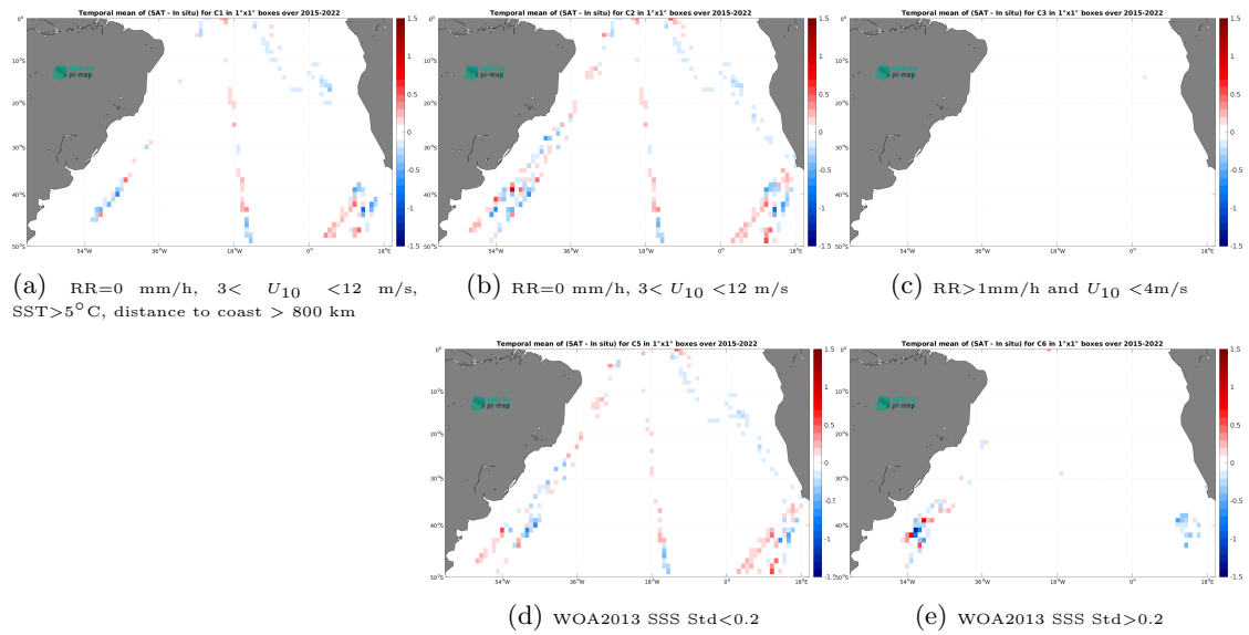
Figure 12: Temporal mean gridded over spatial boxes of size 1^\circ \times 1^\circ of \Delta SSS (SMAP SSS L3 v5 - Monthly (RSS) - TSG (Polarstern)) for 5 different subdatasets corresponding to:RR=0 mm/h, 3 < U_{10} < 12 m/s, SST >5^\circ\text{C} , distance to coast > 800 km (a), RR=0 mm/h, 3 < U_{10} < 12 m/s (b), RR >1 mm/h and U_{10} < 4 m/s (c), WOA2013 SSS Std <0.2 (d), WOA2013 SSS Std >0.2 (e).
