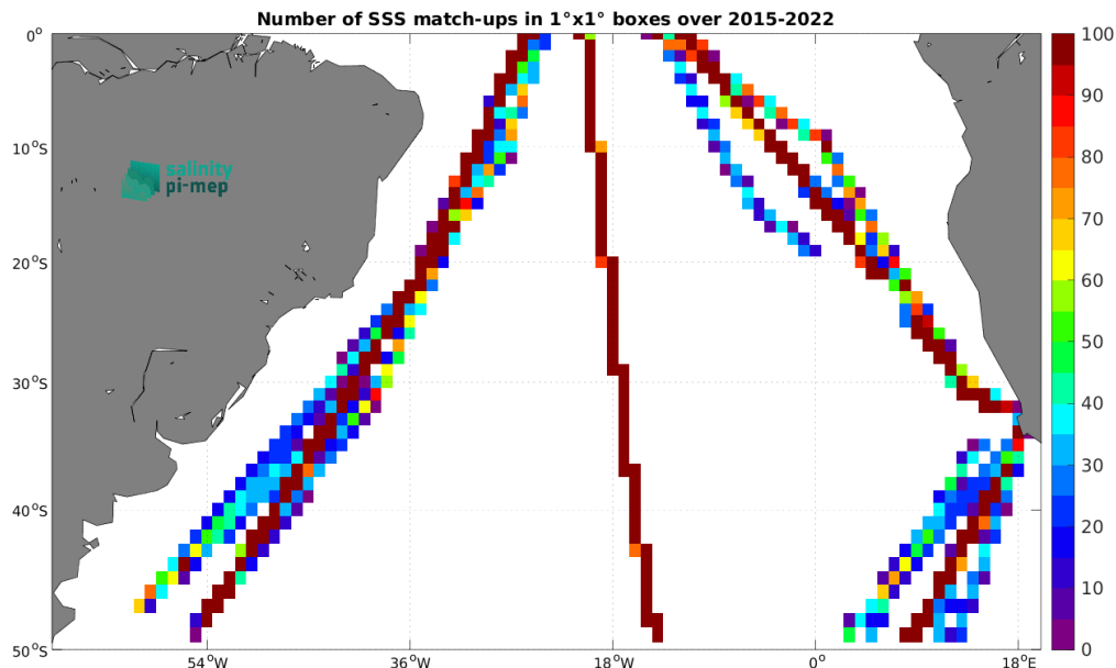
Figure 4: Number of SSS match-ups between TSG (Polarstern) SSS and the SMAP SSS L3 v5 - Monthly (RSS) SSS product for the South Atlantic Ocean Pi-MEP region over 1^\circ \times 1^\circ boxes and for the full satellite product period.
