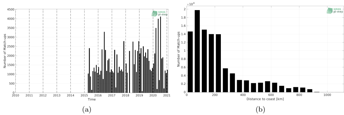
Figure 1: Number of match-ups between TSG (LEGOS-DM) and SMAP SSS L3 v5 - Monthly (RSS) SSS as a function of time (a) and as function of the distance to coast (b) over the South Atlantic Ocean Pi-MEP region and for the full satellite product period.
