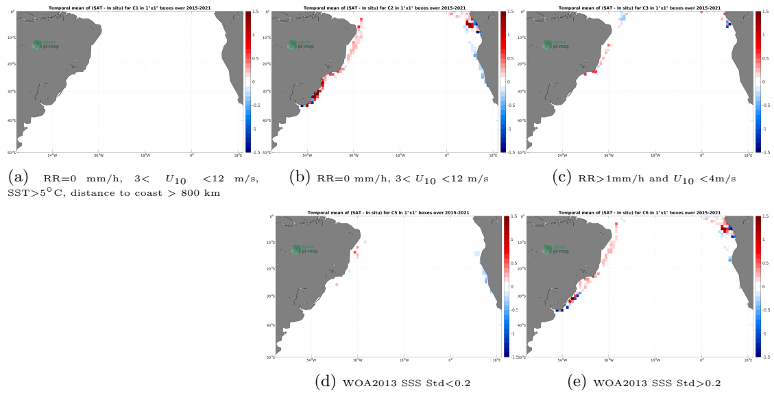
Figure 12: Temporal mean gridded over spatial boxes of size 1^\circ \times 1^\circ of \Delta SSS (SMAP SSS L3 v5 - Monthly (RSS) - TSG (LEGOS-DM)) for 5 different subdatasets corresponding to:RR=0 mm/h, 3 < U_{10} < 12 m/s, SST >5^\circ\text{C} , distance to coast > 800 km (a), RR=0 mm/h, 3 < U_{10} < 12 m/s (b), RR >1 mm/h and U_{10} < 4 m/s (c), WOA2013 SSS Std <0.2 (d), WOA2013 SSS Std >0.2 (e).
