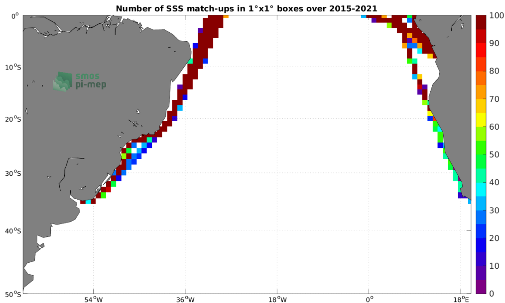
Figure 4: Number of SSS match-ups between TSG (LEGOS-DM) SSS and the SMAP SSS L3 v5 - Monthly (RSS) SSS product for the South Atlantic Ocean Pi-MEP region over 1^\circ \times 1^\circ boxes and for the full satellite product period.
