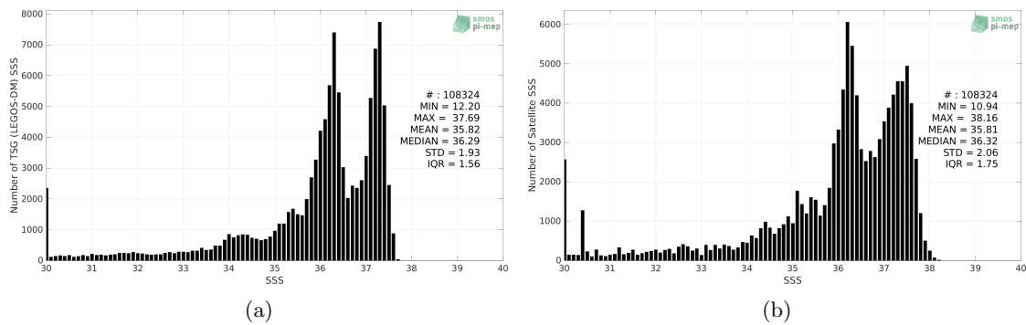
Figure 2: Histograms of SSS from TSG (LEGOS-DM) (a) and SMAP SSS L3 v5 - Monthly (RSS) (b) considering all match-up pairs per bins of 0.1 over the South Atlantic Ocean Pi-MEP region and for the full satellite product period.
