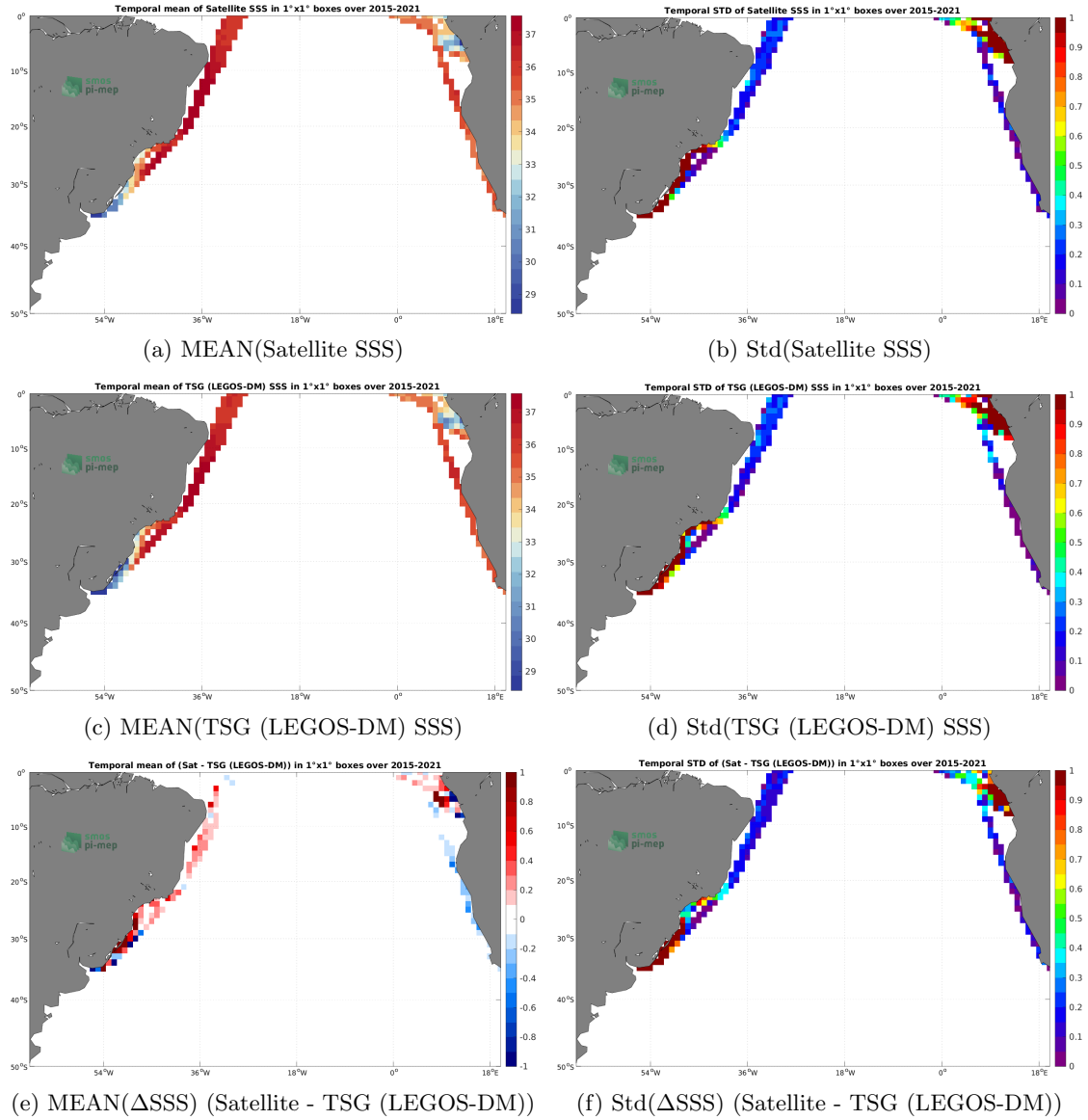
Figure 6: Temporal mean (left) and Std (right) of SSS from SMAP SSS L3 v5 - Monthly (RSS) (top), TSG (LEGOS-DM) (middle), and of \Delta SSS (Satellite - TSG (LEGOS-DM)). Only match-up pairs are used to generate these maps.
