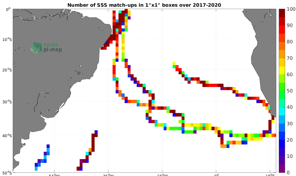
Figure 4: Number of SSS match-ups between TSG (GOSUD-Sailing-ship) SSS and the SMAP SSS L3 v5 - Monthly (RSS) SSS product for the South Atlantic Ocean Pi-MEP region over 1^\circ \times 1^\circ boxes and for the full satellite product period.
