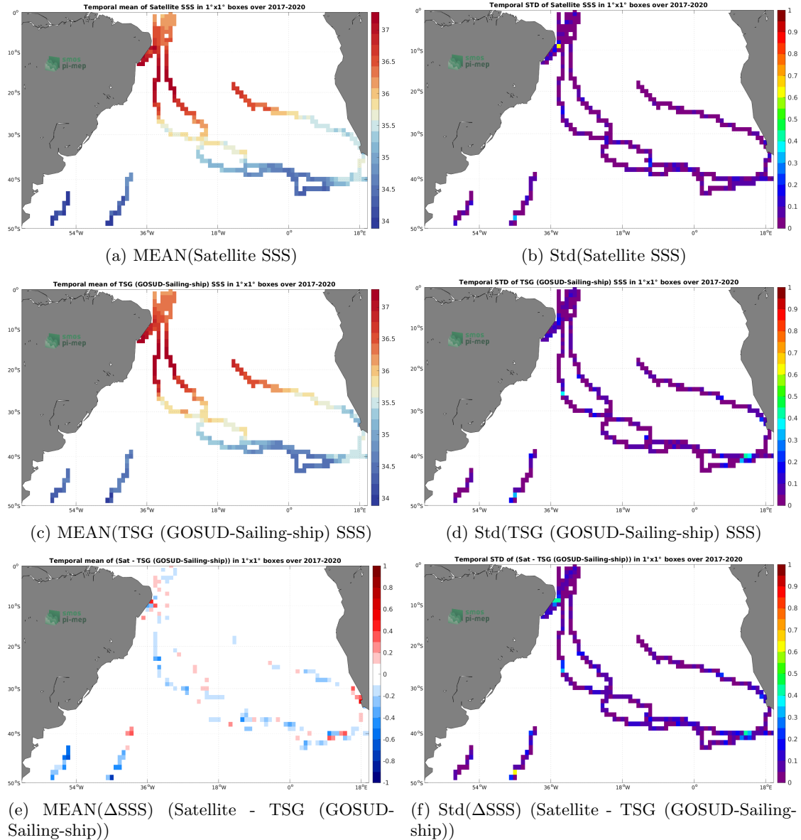
Figure 6: Temporal mean (left) and Std (right) of SSS from SMAP SSS L3 v5 - Monthly (RSS) (top), TSG (GOSUD-Sailing-ship) (middle), and of \Delta SSS (Satellite - TSG (GOSUD-Sailing-ship)). Only match-up pairs are used to generate these maps.
