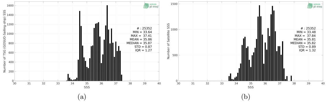
Figure 2: Histograms of SSS from TSG (GOSUD-Sailing-ship) (a) and SMAP SSS L3 v5 - Monthly (RSS) (b) considering all match-up pairs per bins of 0.1 over the South Atlantic Ocean Pi-MEP region and for the full satellite product period.
