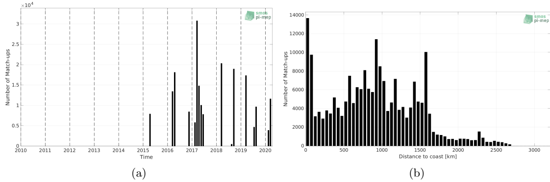
Figure 1: Number of match-ups between TSG (GOSUD-Research-vessel) and SMAP SSS L3 v5 - Monthly (RSS) SSS as a function of time (a) and as function of the distance to coast (b) over the South Atlantic Ocean Pi-MEP region and for the full satellite product period.
