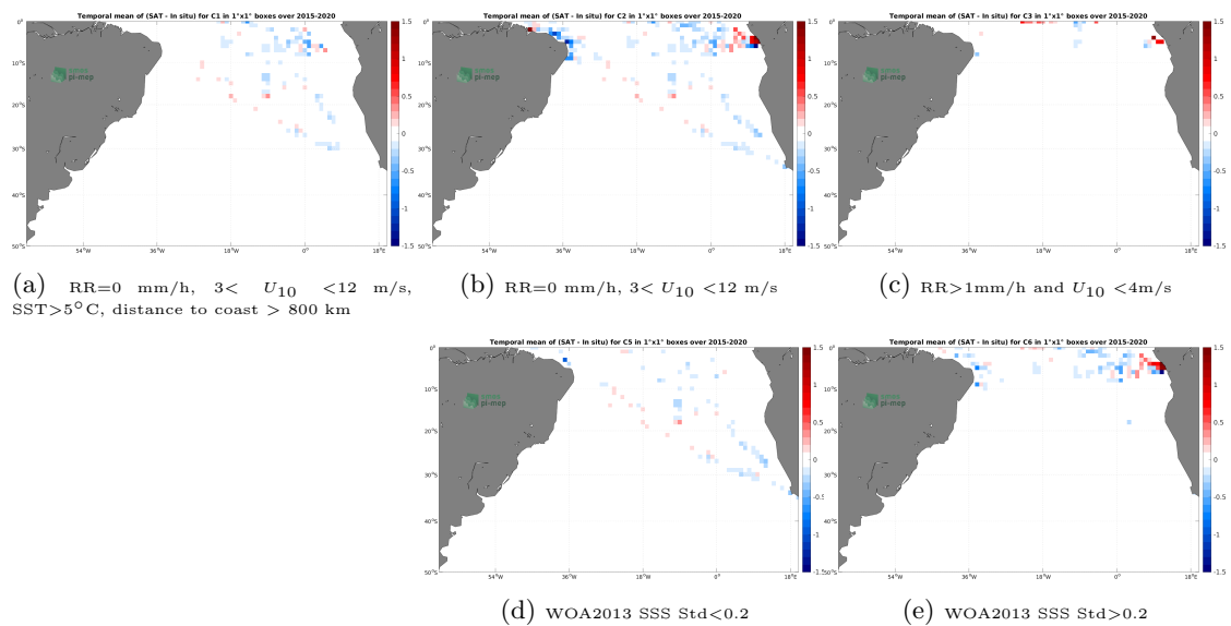
Figure 12: Temporal mean gridded over spatial boxes of size 1^\circ \times 1^\circ of \Delta SSS (SMAP SSS L3 v5 - Monthly (RSS) - TSG (GOSUD-Research-vessel)) for 5 different subdatasets corresponding to:RR=0 mm/h, 3 < U_{10} < 12 m/s, SST>5°C, distance to coast > 800 km (a), RR=0 mm/h, 3 < U_{10} < 12 m/s (b), RR>1mm/h and U_{10} < 4 m/s (c), WOA2013 SSS Std<0.2 (d), WOA2013 SSS Std>0.2 (e).
