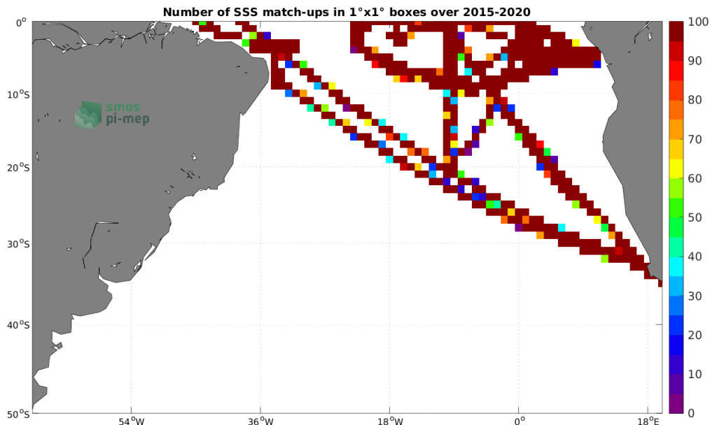
Figure 4: Number of SSS match-ups between TSG (GOSUD-Research-vessel) SSS and the SMAP SSS L3 v5 - Monthly (RSS) SSS product for the South Atlantic Ocean Pi-MEP region over 1^\circ \times 1^\circ boxes and for the full satellite product period.
