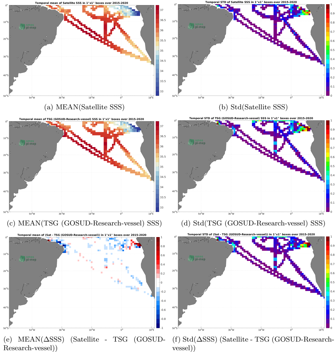
Figure 6: Temporal mean (left) and Std (right) of SSS from SMAP SSS L3 v5 - Monthly (RSS) (top), TSG (GOSUD-Research-vessel) (middle), and of \Delta SSS (Satellite - TSG (GOSUD-Research-vessel)). Only match-up pairs are used to generate these maps.
