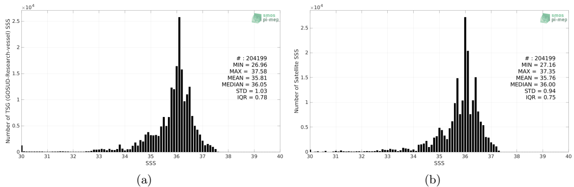
Figure 2: Histograms of SSS from TSG (GOSUD-Research-vessel) (a) and SMAP SSS L3 v5 - Monthly (RSS) (b) considering all match-up pairs per bins of 0.1 over the South Atlantic Ocean Pi-MEP region and for the full satellite product period.
