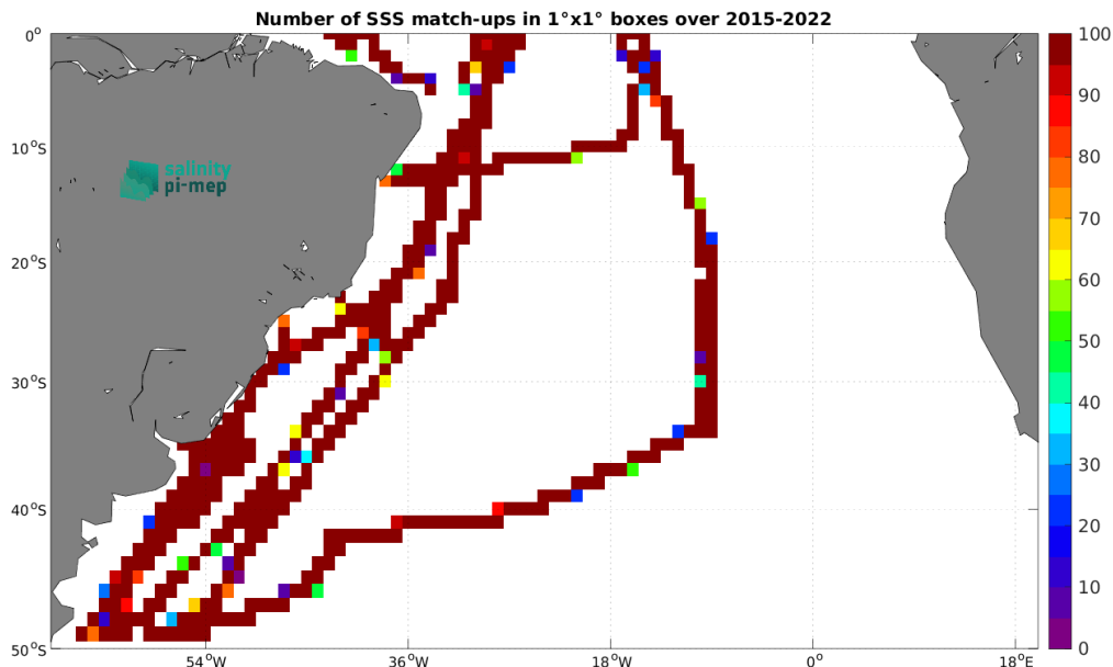
Figure 4: Number of SSS match-ups between TSG (CSIC-UTM) SSS and the SMAP SSS L3 v5 - Monthly (RSS) SSS product for the South Atlantic Ocean Pi-MEP region over 1^\circ \times 1^\circ boxes and for the full satellite product period.
