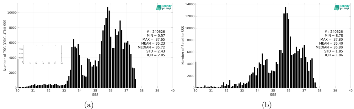
Figure 2: Histograms of SSS from TSG (CSIC-UTM) (a) and SMAP SSS L3 v5 - Monthly (RSS) (b) considering all match-up pairs per bins of 0.1 over the South Atlantic Ocean Pi-MEP region and for the full satellite product period.
