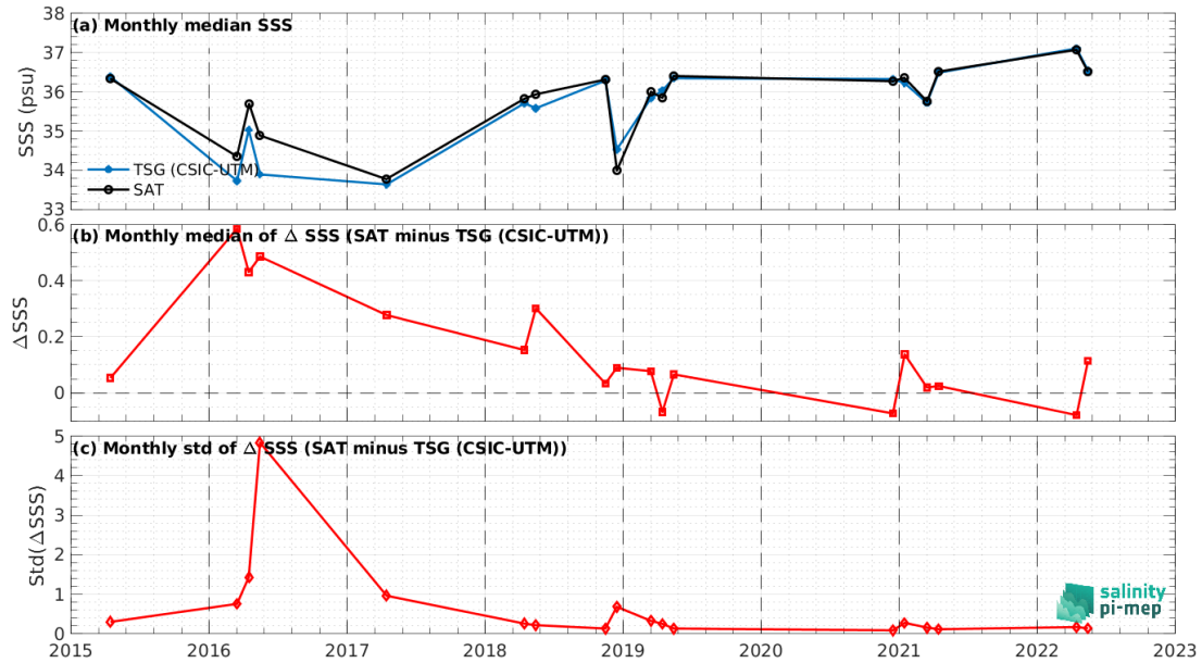
Figure 7: Time series of the monthly median SSS (top), median of \Delta\text{SSS} (Satellite - TSG (CSIC-UTM)) and Std of \Delta\text{SSS} (Satellite - TSG (CSIC-UTM)) over the South Atlantic Ocean Pi-MEP region considering all match-ups collected by the Pi-MEP.
