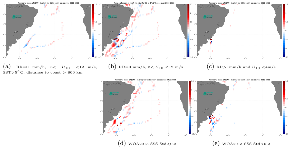
Figure 12: Temporal mean gridded over spatial boxes of size 1^\circ \times 1^\circ of \Delta\text{SSS} (SMAP SSS L3 v5 - Monthly (RSS) - TSG (CSIC-UTM)) for 5 different subdatasets corresponding to: \text{RR}=0 mm/h, 3 < U_{10} < 12 m/s, \text{SST} > 5^\circ\text{C} , distance to coast > 800 km (a), \text{RR}=0 mm/h, 3 < U_{10} < 12 m/s (b), \text{RR} > 1\text{mm/h} and U_{10} < 4\text{m/s} (c), WOA2013 SSS Std < 0.2 (d), WOA2013 SSS Std > 0.2 (e).
