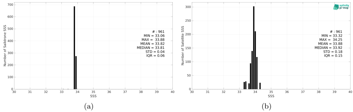
Figure 2: Histograms of SSS from Saildrone (a) and SMAP SSS L3 v5 - Monthly (RSS) (b) considering all match-up pairs per bins of 0.1 over the South Atlantic Ocean Pi-MEP region and for the full satellite product period.
