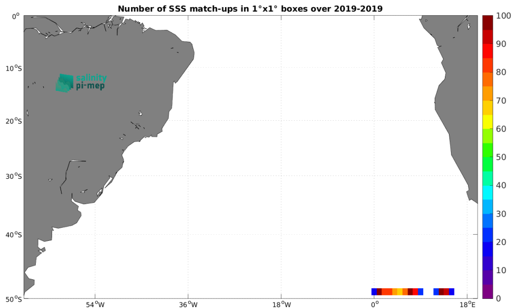
Figure 4: Number of SSS match-ups between Saildrone SSS and the SMAP SSS L3 v5 - Monthly (RSS) SSS product for the South Atlantic Ocean Pi-MEP region over 1^\circ \times 1^\circ boxes and for the full satellite product period.
