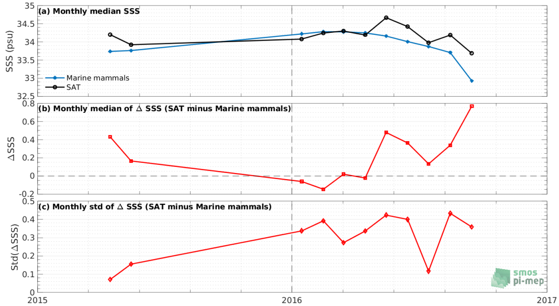
Figure 7: Time series of the monthly median SSS (top), median of \Delta\text{SSS} (Satellite - Marine mammals) and Std of \Delta\text{SSS} (Satellite - Marine mammals) over the South Atlantic Ocean Pi-MEP region considering all match-ups collected by the Pi-MEP.
