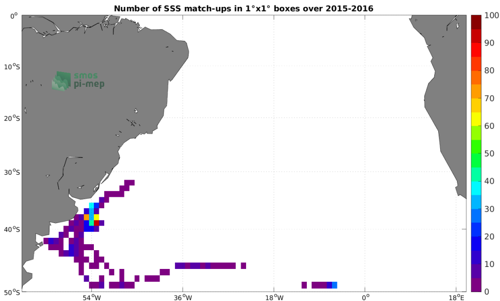
Figure 4: Number of SSS match-ups between Marine mammals SSS and the SMAP SSS L3 v5 - Monthly (RSS) SSS product for the South Atlantic Ocean Pi-MEP region over 1^\circ \times 1^\circ boxes and for the full satellite product period.
