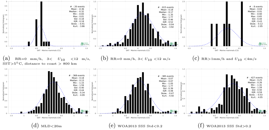
Figure 13: Normalized histogram of \Delta SSS (SMAP SSS L3 v5 - Monthly (RSS) - Marine mammals) for 6 different subdatasets corresponding to: RR=0 mm/h, 3 < U_{10} < 12 m/s, SST>5°C, distance to coast > 800 km (a), RR=0 mm/h, 3 < U_{10} < 12 m/s (b), RR>1mm/h and U_{10} < 4 m/s (c), MLD<20m (d), WOA2013 SSS Std<0.2 (e), WOA2013 SSS Std>0.2 (f).
