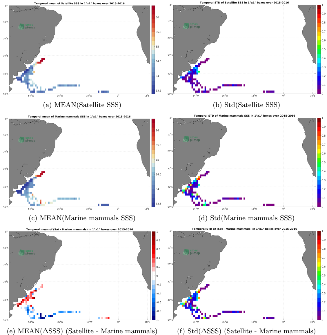
Figure 6: Temporal mean (left) and Std (right) of SSS from SMAP SSS L3 v5 - Monthly (RSS) (top), Marine mammals (middle), and of \Delta SSS (Satellite - Marine mammals). Only match-up pairs are used to generate these maps.
