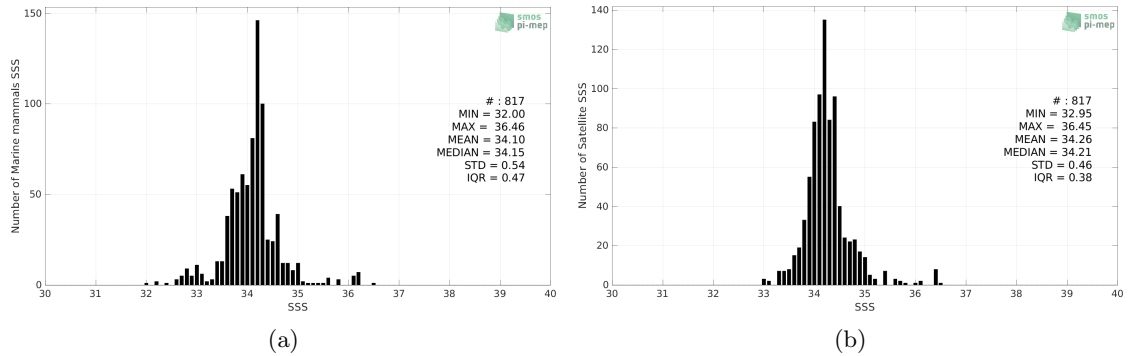
Figure 2: Histograms of SSS from Marine mammals (a) and SMAP SSS L3 v5 - Monthly (RSS) (b) considering all match-up pairs per bins of 0.1 over the South Atlantic Ocean Pi-MEP region and for the full satellite product period.
