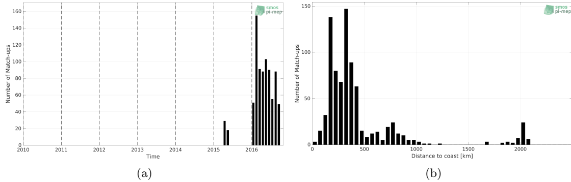
Figure 1: Number of match-ups between Marine mammals and SMAP SSS L3 v5 - Monthly (RSS) SSS as a function of time (a) and as function of the distance to coast (b) over the South Atlantic Ocean Pi-MEP region and for the full satellite product period.
