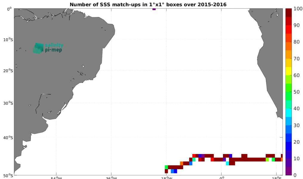
Figure 3: Number of SSS match-ups between Surface drifters SSS and the SMAP SSS L3 v5 - Monthly (RSS) SSS product for the South Atlantic Ocean Pi-MEP region over 1^\circ \times 1^\circ boxes and for the full satellite product period.
