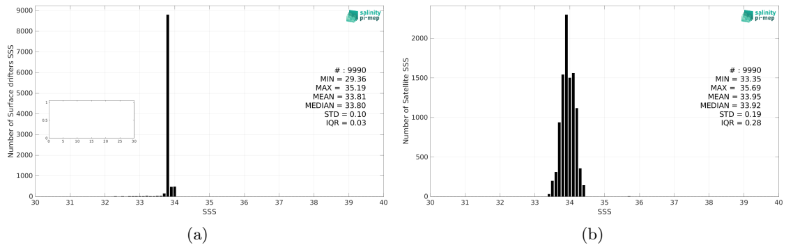
Figure 2: Histograms of SSS from Surface drifters (a) and SMAP SSS L3 v5 - Monthly (RSS) (b) considering all match-up pairs per bins of 0.1 over the South Atlantic Ocean Pi-MEP region and for the full satellite product period.
