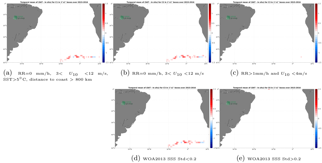
Figure 11: Temporal mean gridded over spatial boxes of size 1^{\circ}\times 1^{\circ} of \Delta\text{SSS} (SMAP SSS L3 v5 - Monthly (RSS) - Surface drifters) for 5 different subdatasets corresponding to: \text{RR}=0 mm/h, 3 < U_{10} < 12 m/s, \text{SST} > 5^{\circ}\text{C} , distance to coast > 800 km (a), \text{RR}=0 mm/h, 3 < U_{10} < 12 m/s (b), \text{RR} > 1 mm/h and U_{10} < 4 m/s (c), WOA2013 SSS Std < 0.2 (d), WOA2013 SSS Std > 0.2 (e).
