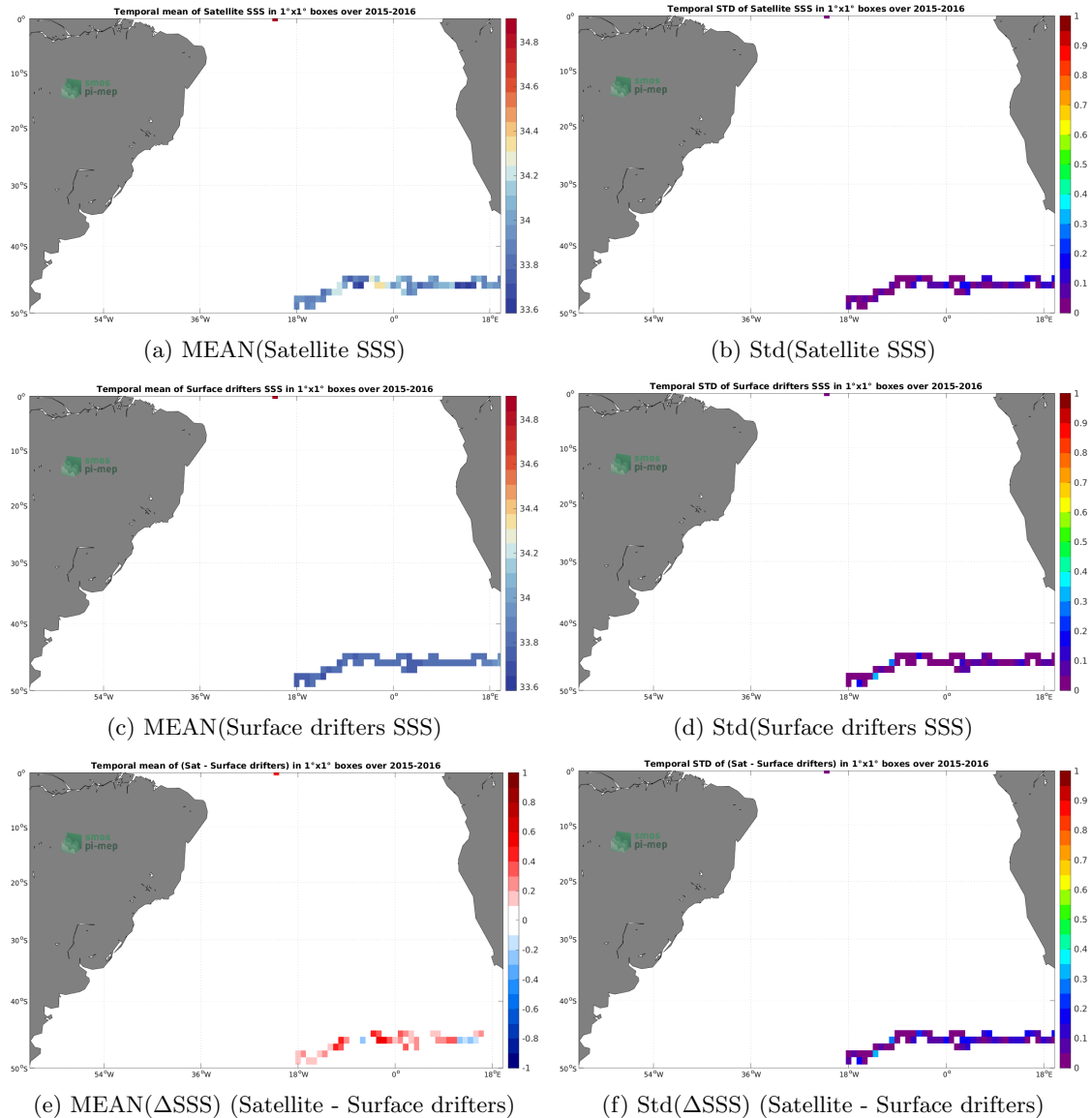
Figure 5: Temporal mean (left) and Std (right) of SSS from SMAP SSS L3 v5 - Monthly (RSS) (top), Surface drifters (middle), and of \Delta SSS (Satellite - Surface drifters). Only match-up pairs are used to generate these maps.
