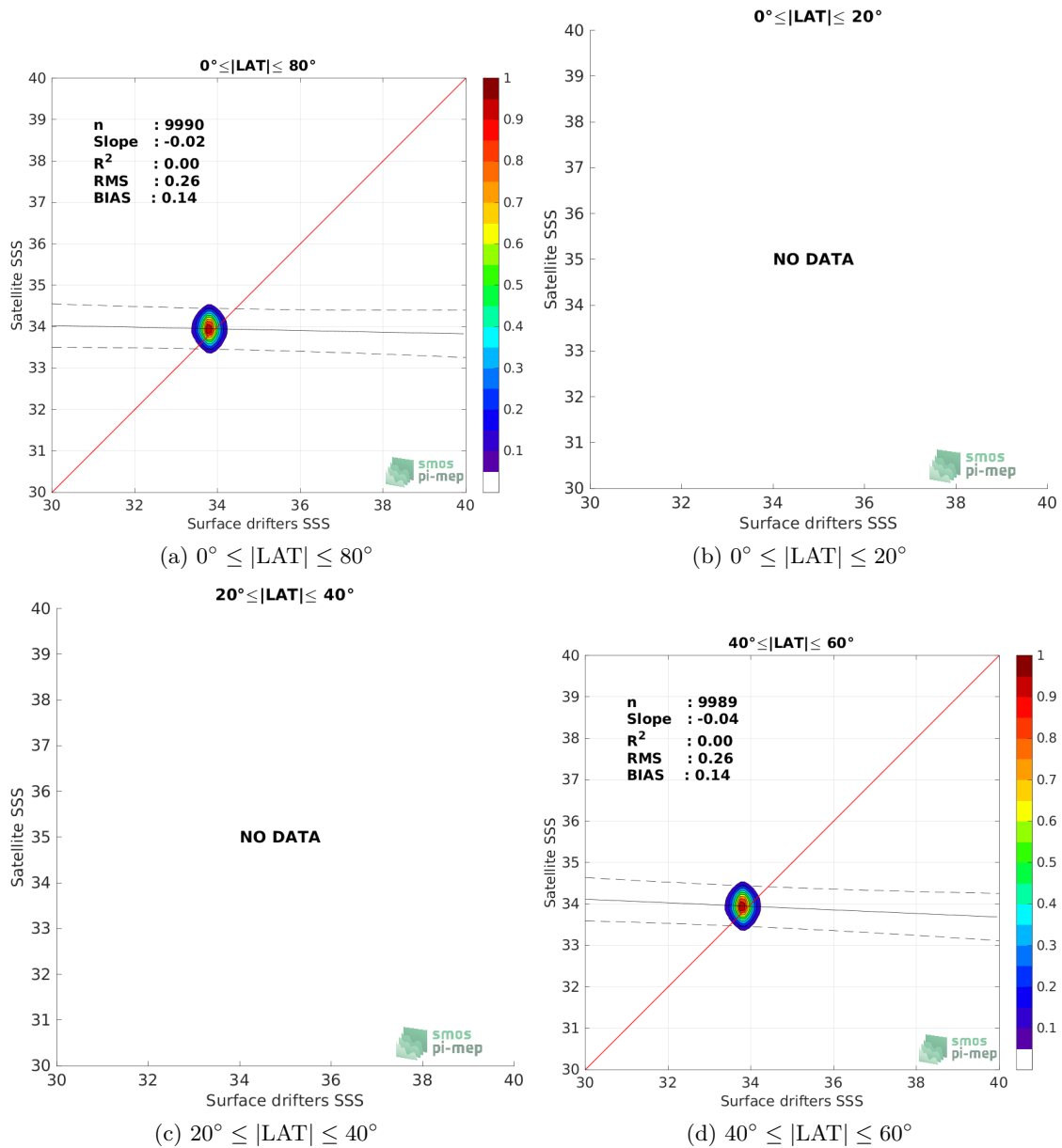
Figure 8: Contour maps of the concentration of SMAP SSS L3 v5 - Monthly (RSS) SSS (y-axis) versus Surface drifters SSS (x-axis) at match-up pairs for different latitude bands. For each plot, the red line shows x=y . The black thin and dashed lines indicate a linear fit through the data cloud and the \pm 95\% confidence levels, respectively. The number match-up pairs n , the slope and R^2 coefficient of the linear fit, the root mean square (RMS) and the mean bias between satellite and in situ data are indicated for each latitude band in each plots.
