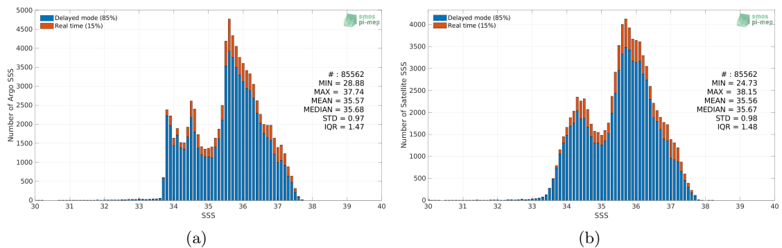
Figure 2: Histograms of SSS from Argo (a) and SMAP SSS L3 v5 - Monthly (RSS) (b) considering all match-up pairs per bins of 0.1 over the South Atlantic Ocean Pi-MEP region and for the full satellite product period.
