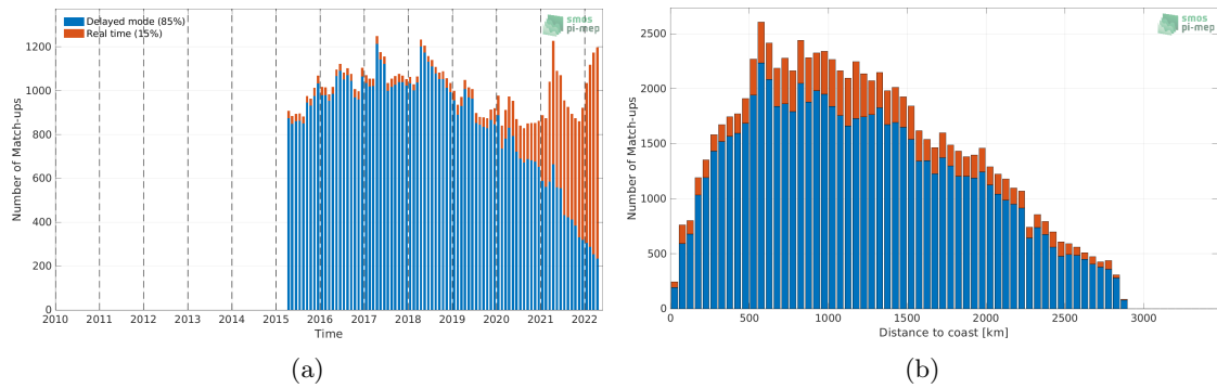
Figure 1: Number of match-ups between Argo and SMAP SSS L3 v5 - Monthly (RSS) SSS as a function of time (a) and as function of the distance to coast (b) over the South Atlantic Ocean Pi-MEP region and for the full satellite product period.
