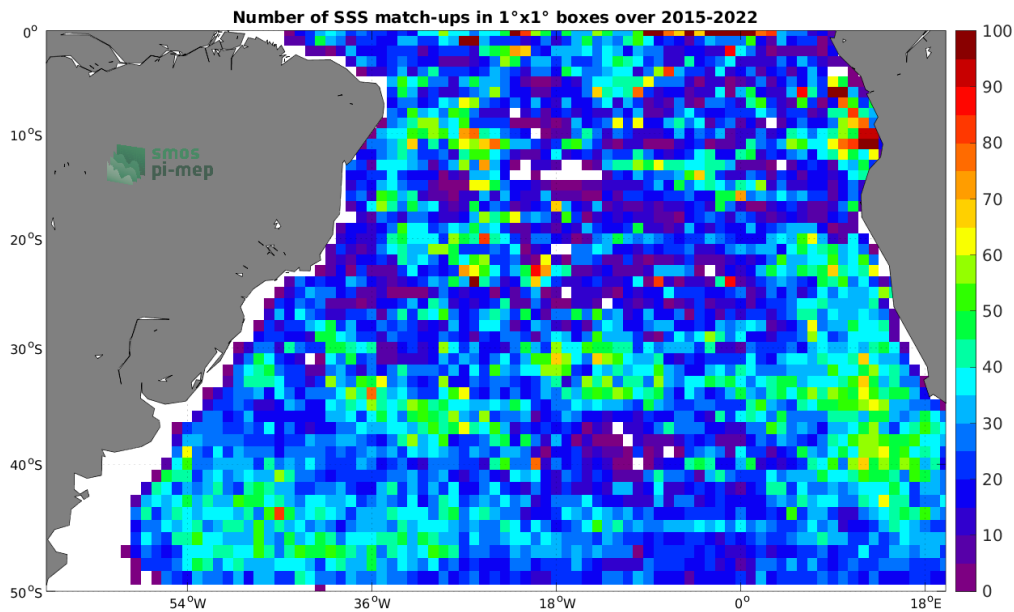
Figure 4: Number of SSS match-ups between Argo SSS and the SMAP SSS L3 v5 - Monthly (RSS) SSS product for the South Atlantic Ocean Pi-MEP region over 1^\circ \times 1^\circ boxes and for the full satellite product period.
