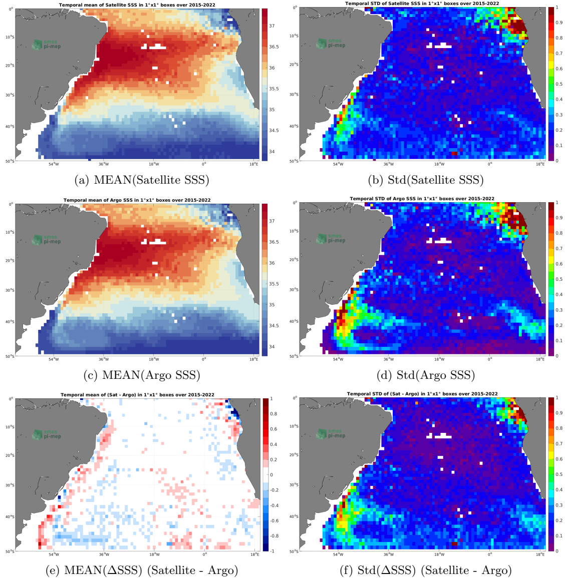
Figure 6: Temporal mean (left) and Std (right) of SSS from SMAP SSS L3 v5 - Monthly (RSS) (top), Argo (middle), and of \Delta SSS (Satellite - Argo). Only match-up pairs are used to generate these maps.
